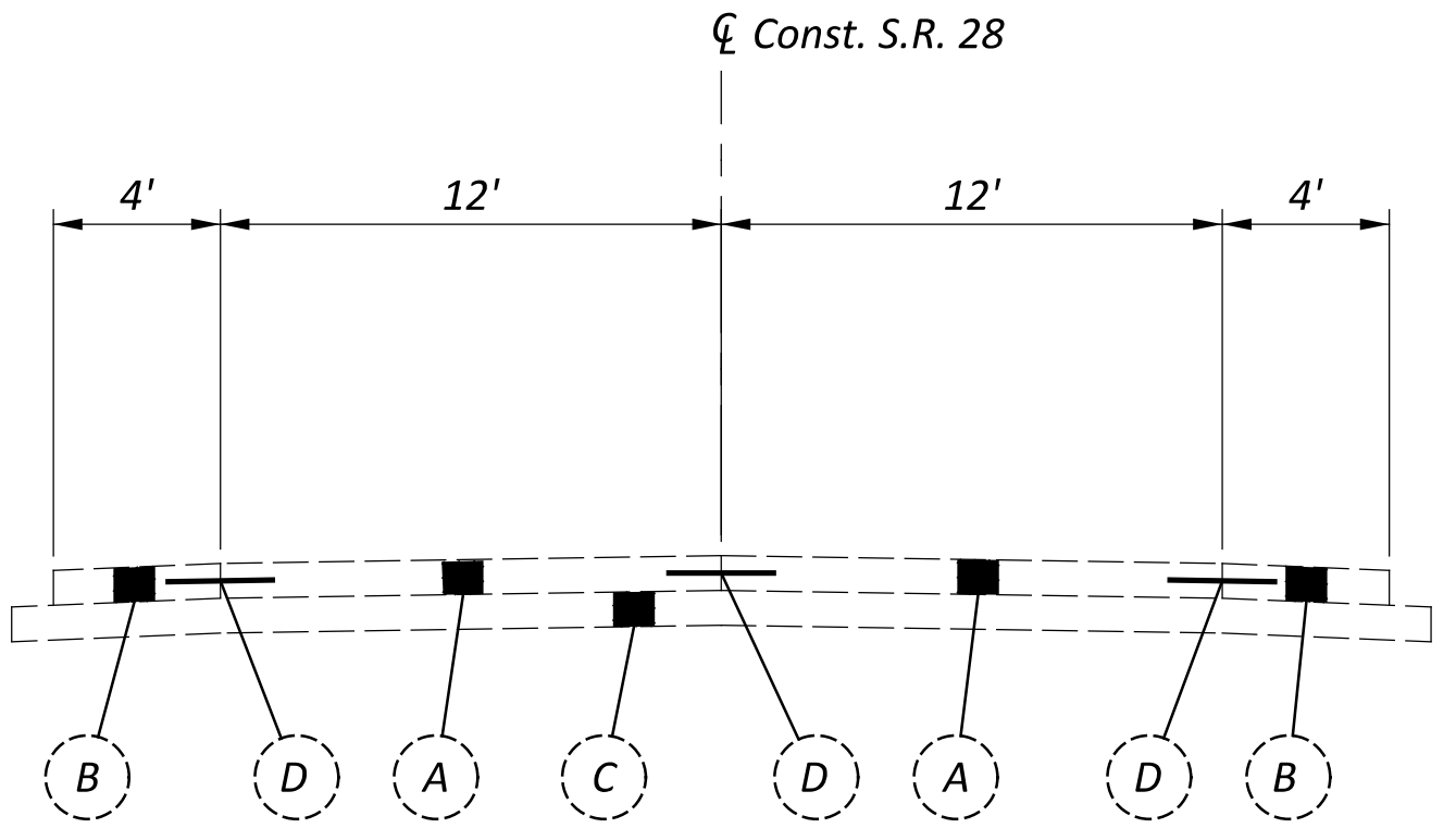
TYPICAL SECTION OF ADJOINING PAVEMENT STA. 2+25, S.R. 28
