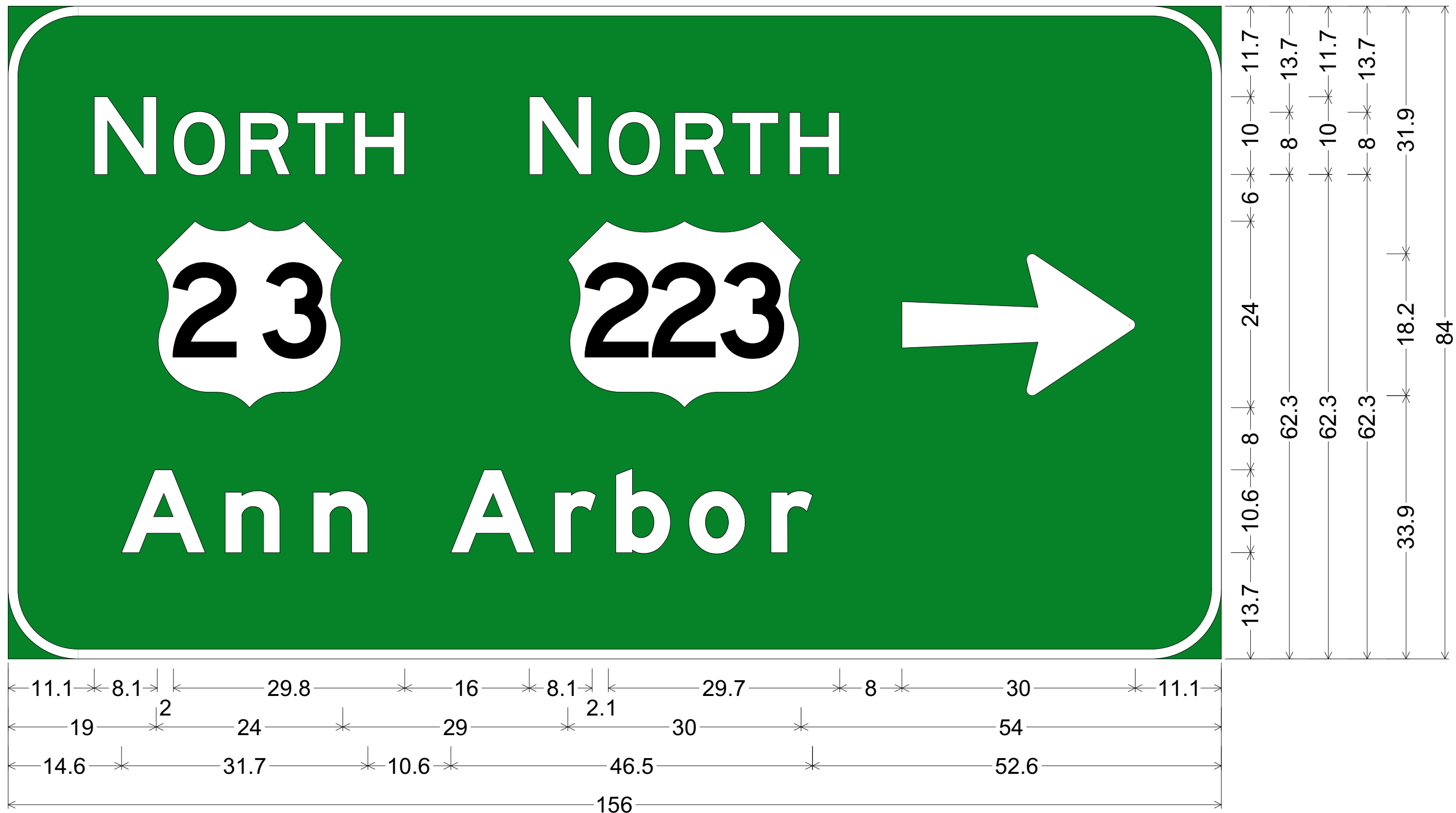
9.0" Radius, 1.3" Border, White on Green; "NORTH", E 2K; US 23 M1-4; "NORTH", E 2K; US 223 M1-4; "Ann Arbor", E Mod 2K; Arrow A-3 - 30.0" 0°;
