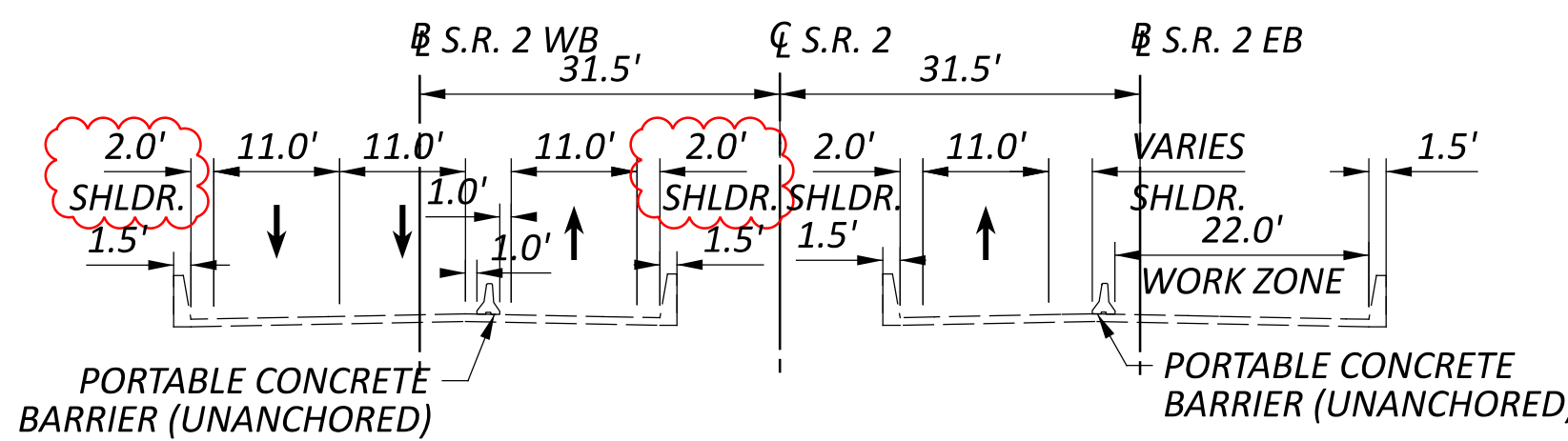
S.R. 2 BRIDGE OVER MURRAY RIDGE RD STA. 608+00 E-E PHASE 2B
