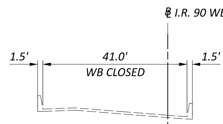
I.R. 90 WB BRIDGE OVER S.R. 2 STA. 626+00 G-G PHASE 2A THROUGH 2B
