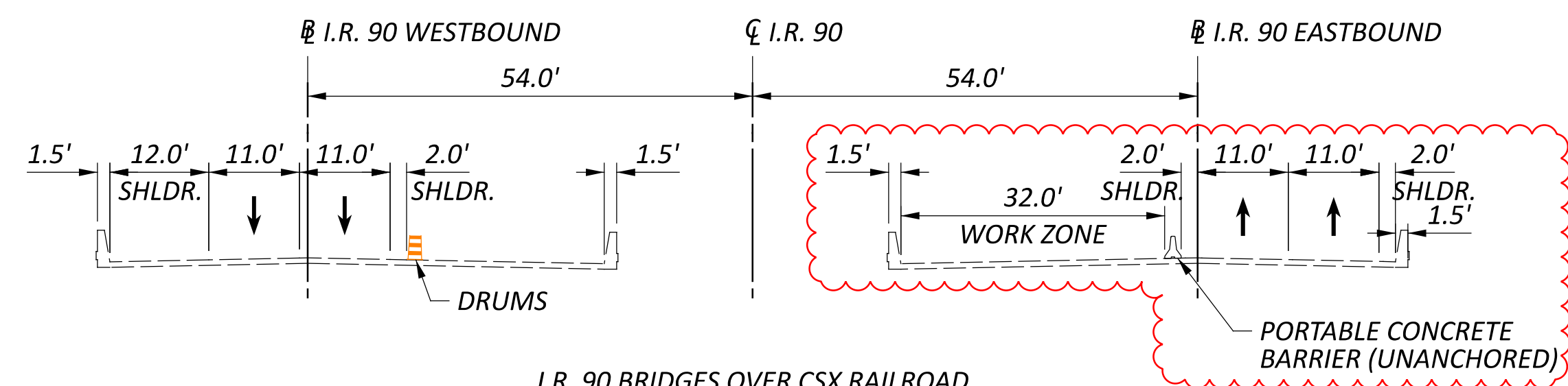
I.R. 90 BRIDGES OVER CSX RAILROAD STA. 662+00 J-J PHASE 2A THROUGH 2B
