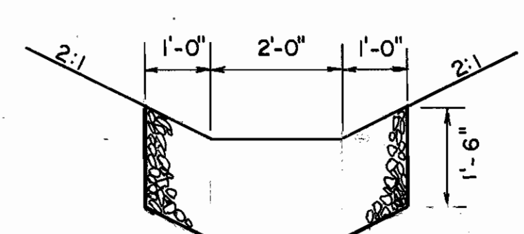
ROCK CHANNEL PROTECTION TYPE C w/FILTER SECTION B-B
