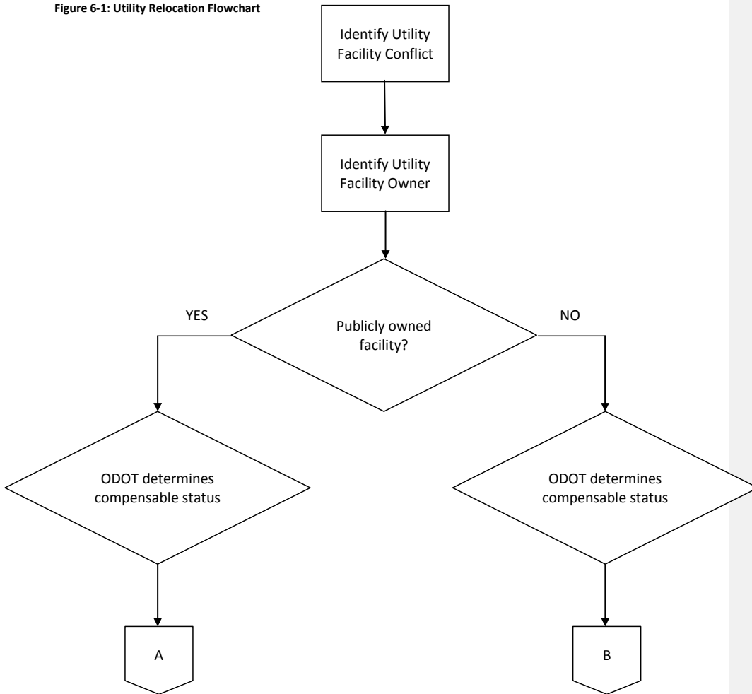
Figure 6-1: Utility Relocation Flowchart
