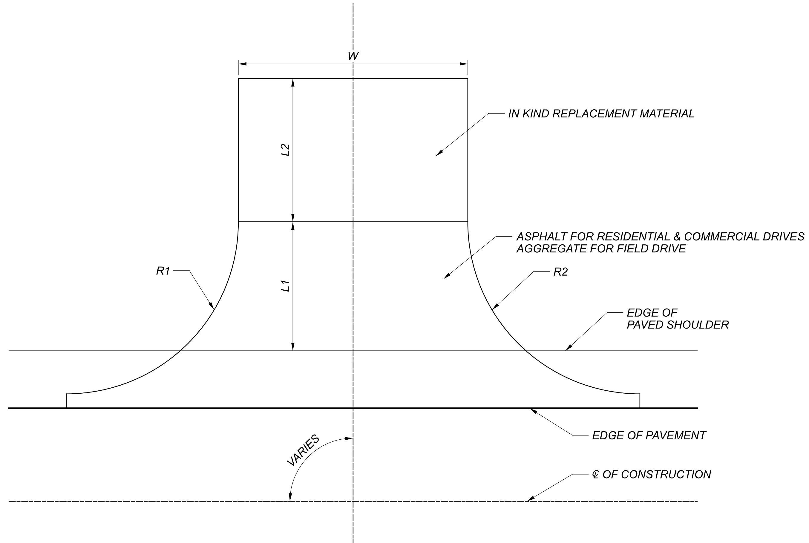
TYPICAL DRIVEWAY PLAN VIEW
