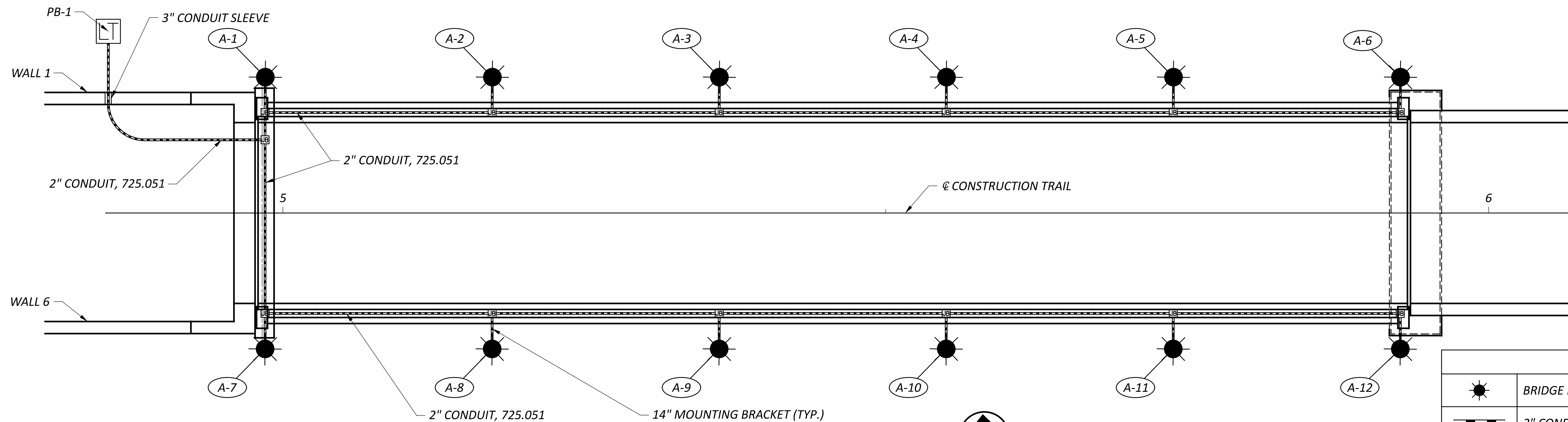
PLAN VIEW
