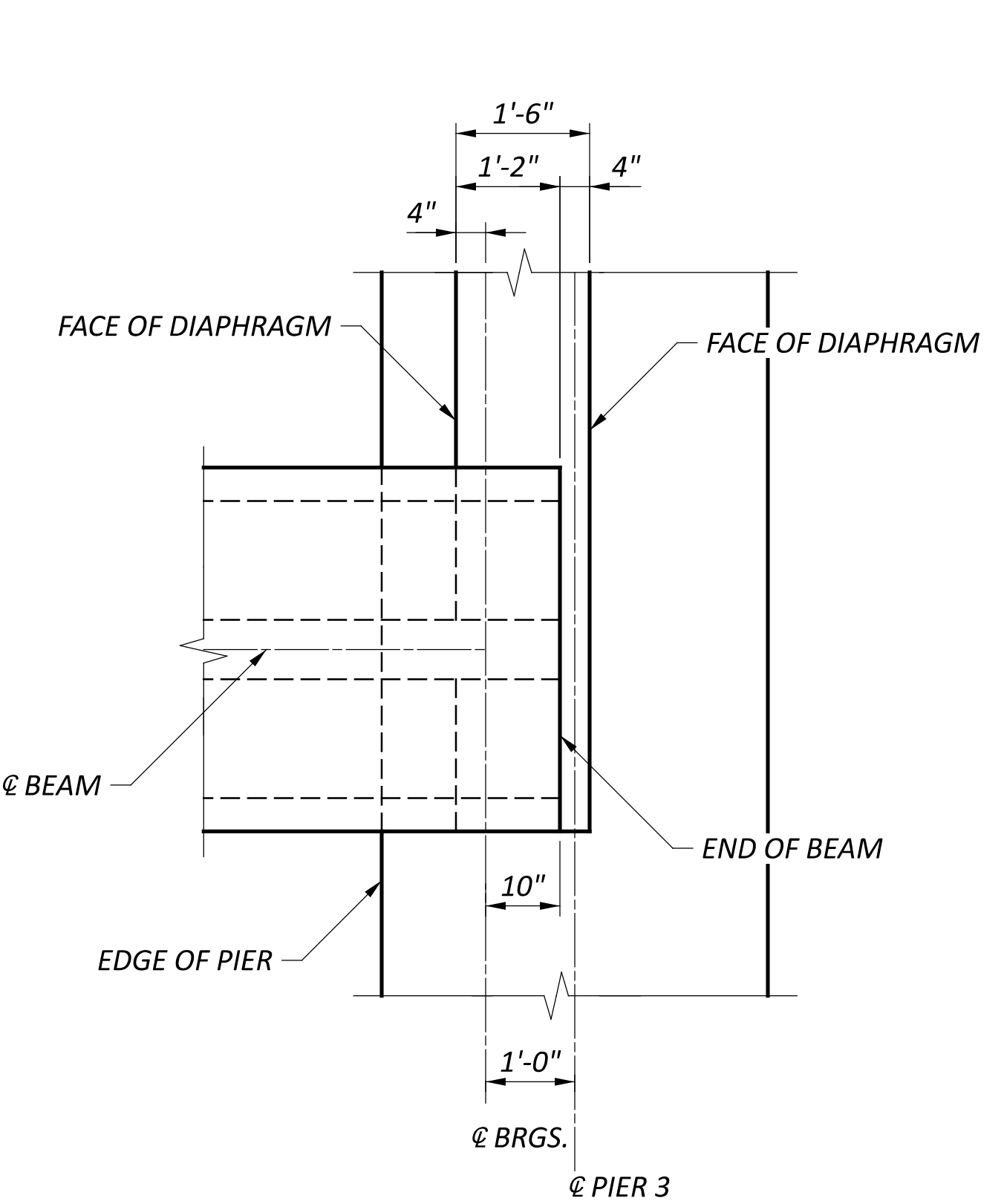
PIER 3 PARTIAL PLAN
