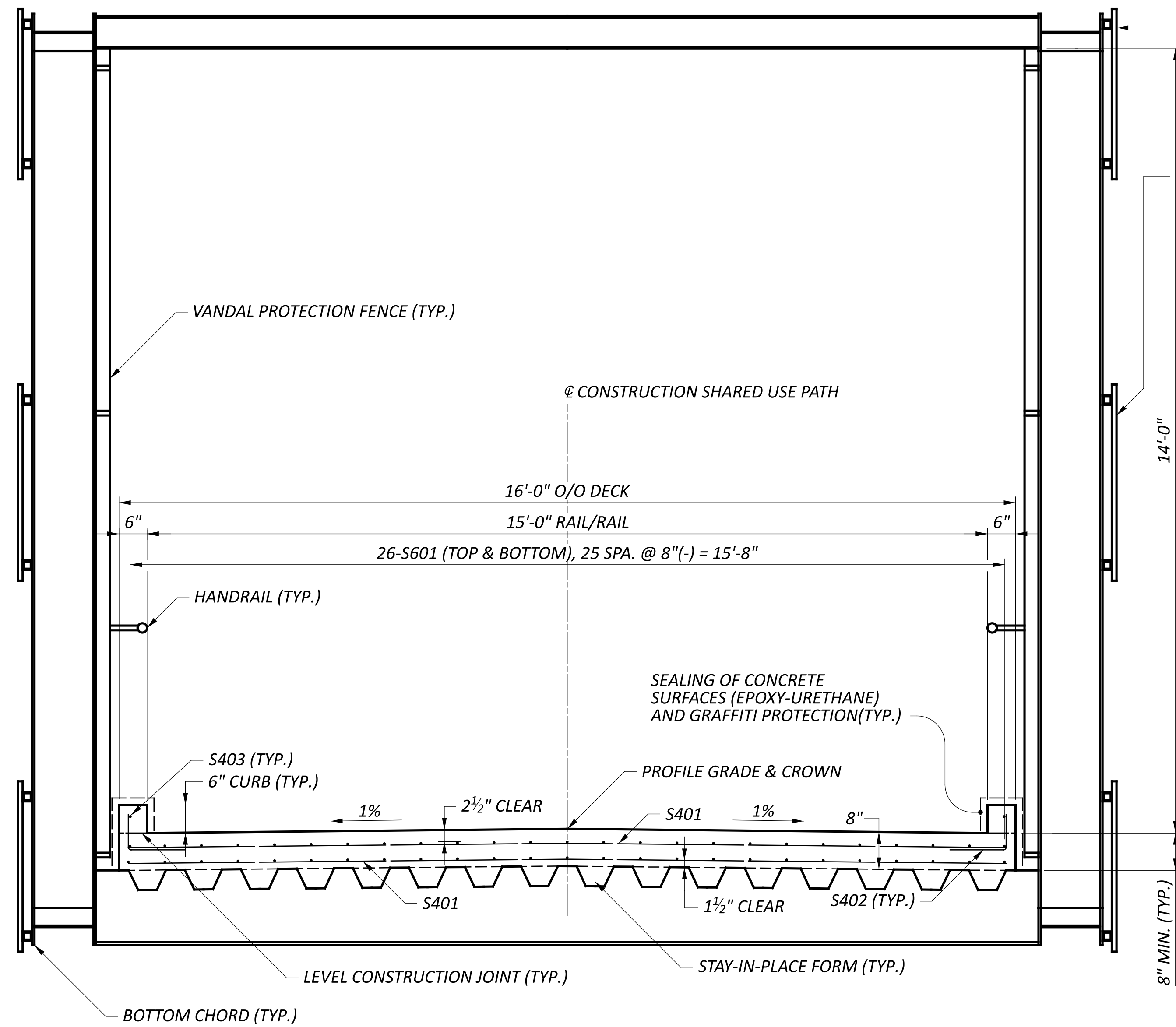
TRANSVERSE SECTION SPAN 1
