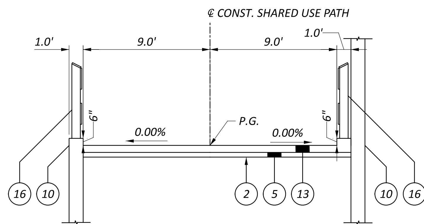
TYPICAL SECTION - SHARED USE PATH
