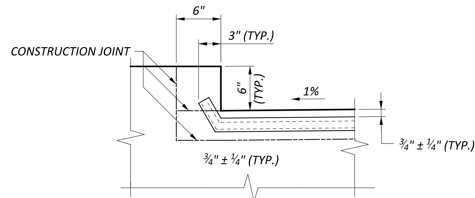
T SECTION 24
