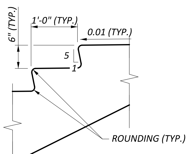
NOSING DETAIL
