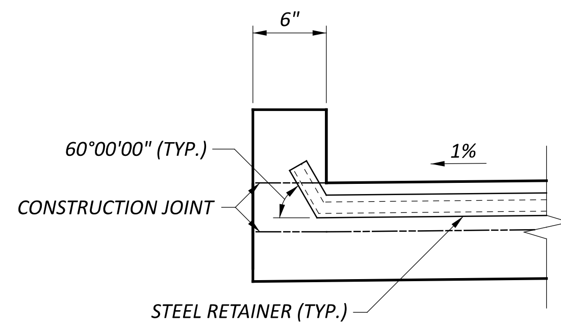
U SECTION 24
