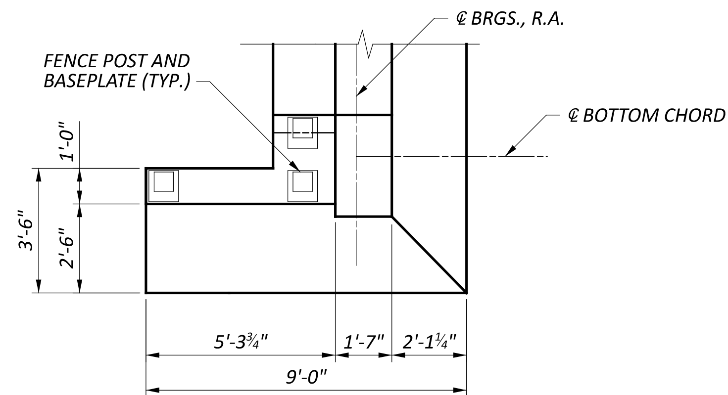
WINGWALL 1 PLAN WINGWALL 2 OPPOSITE, ADJACENT RETAINING WALLS NOT SHOWN
