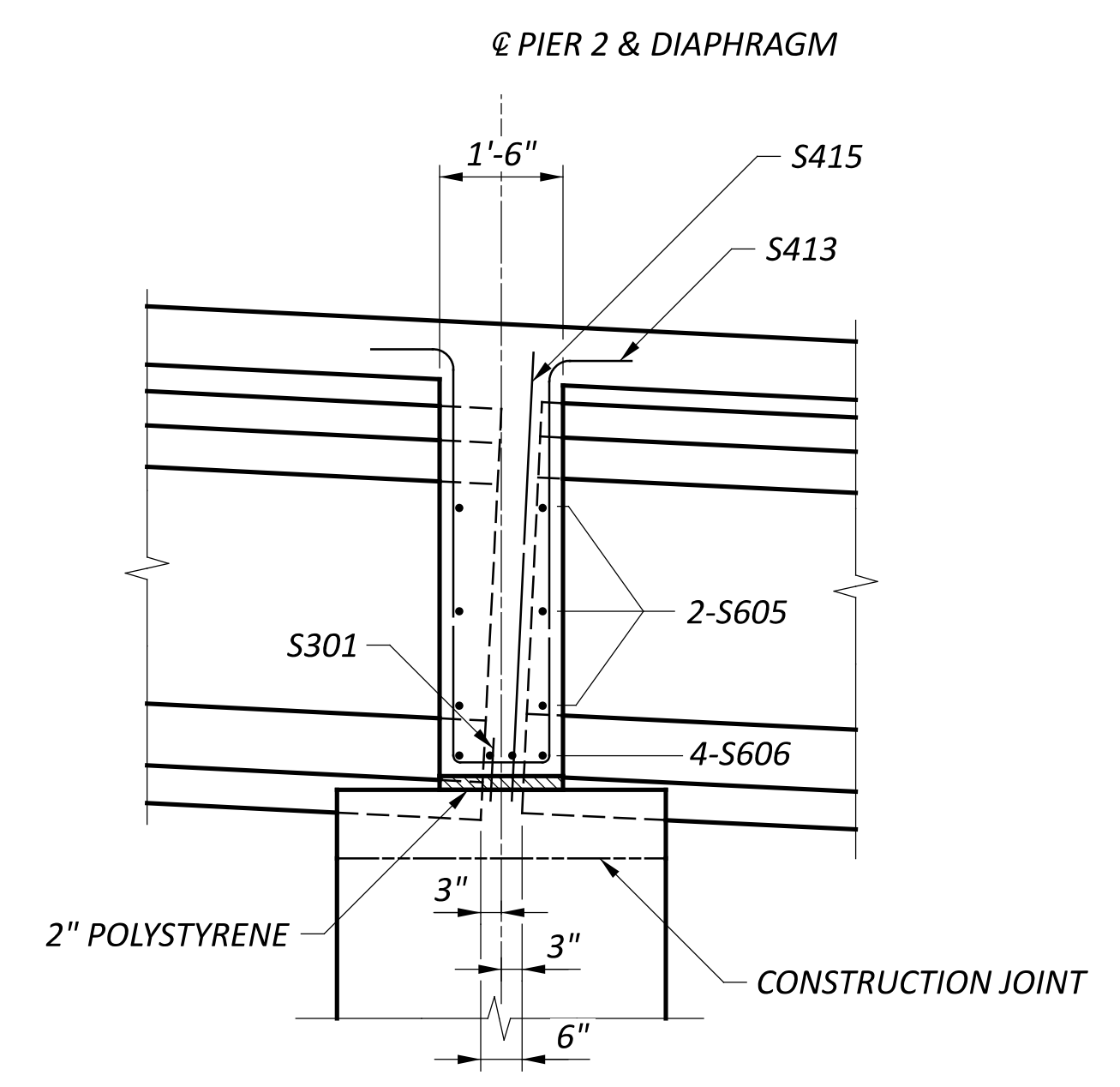
SECTION
