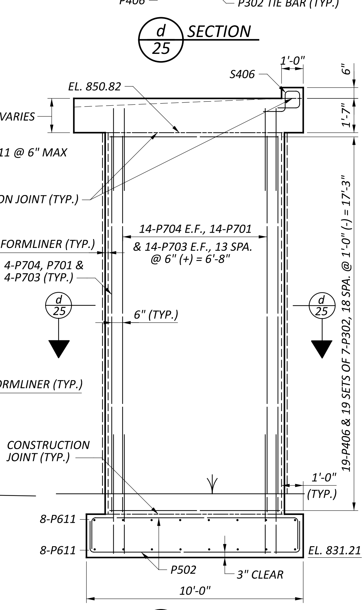
d SECTION 25
