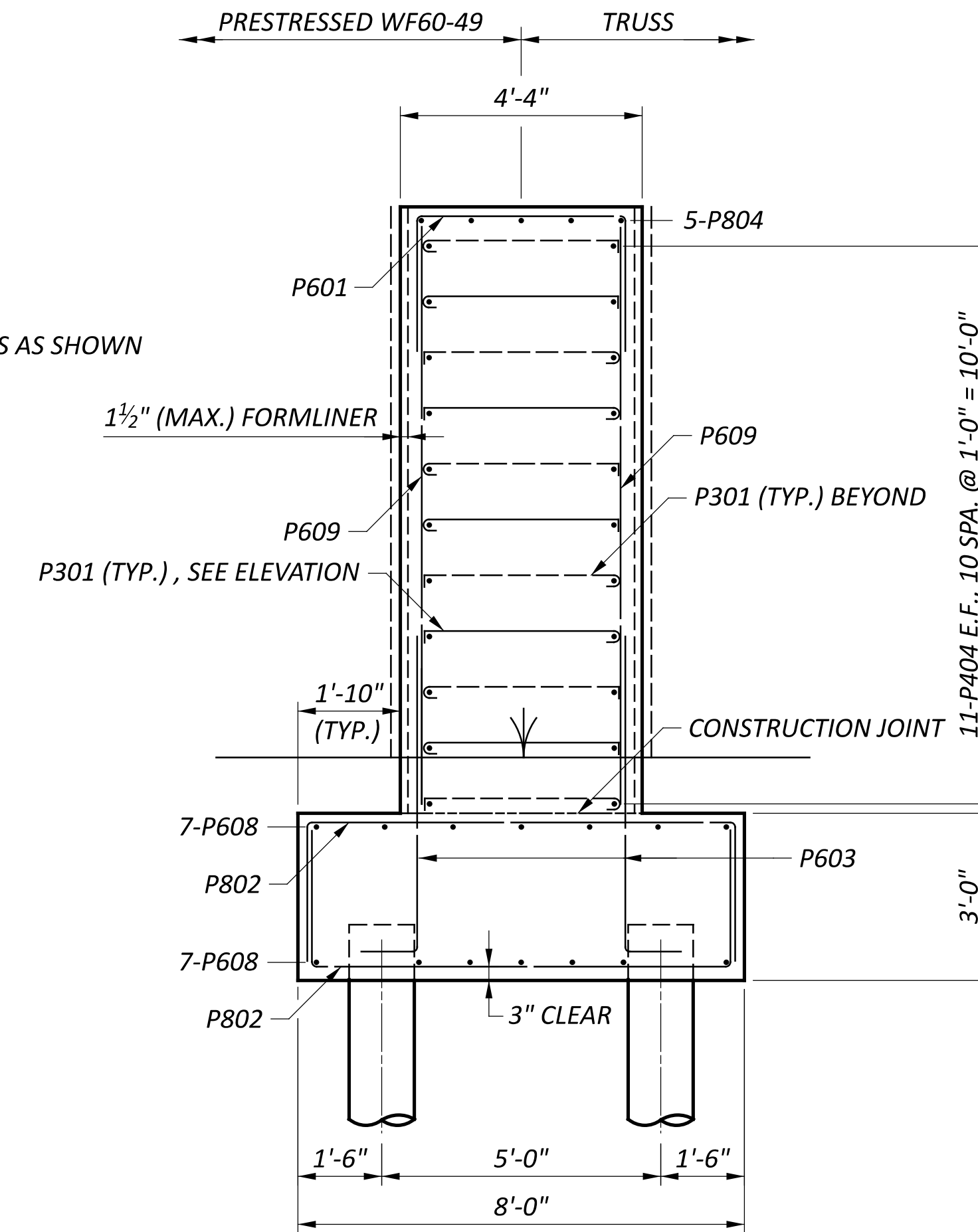
K SECTION 11
