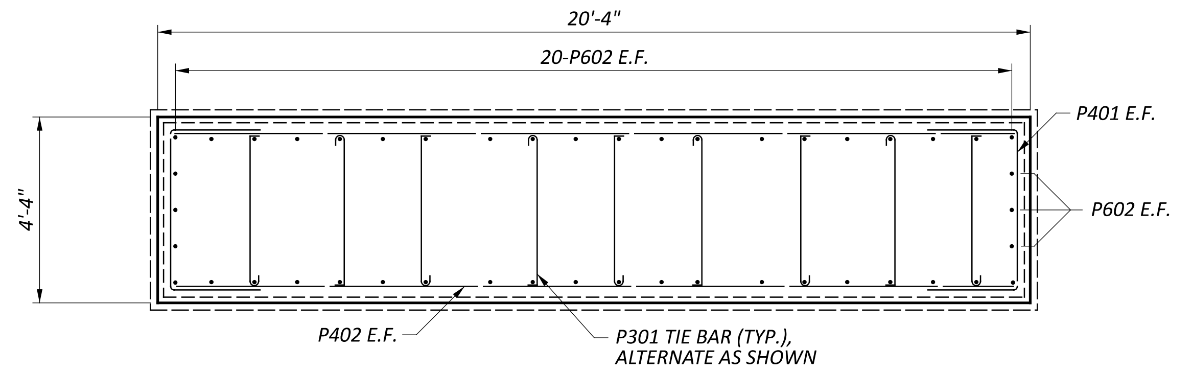
E SECTION 9
