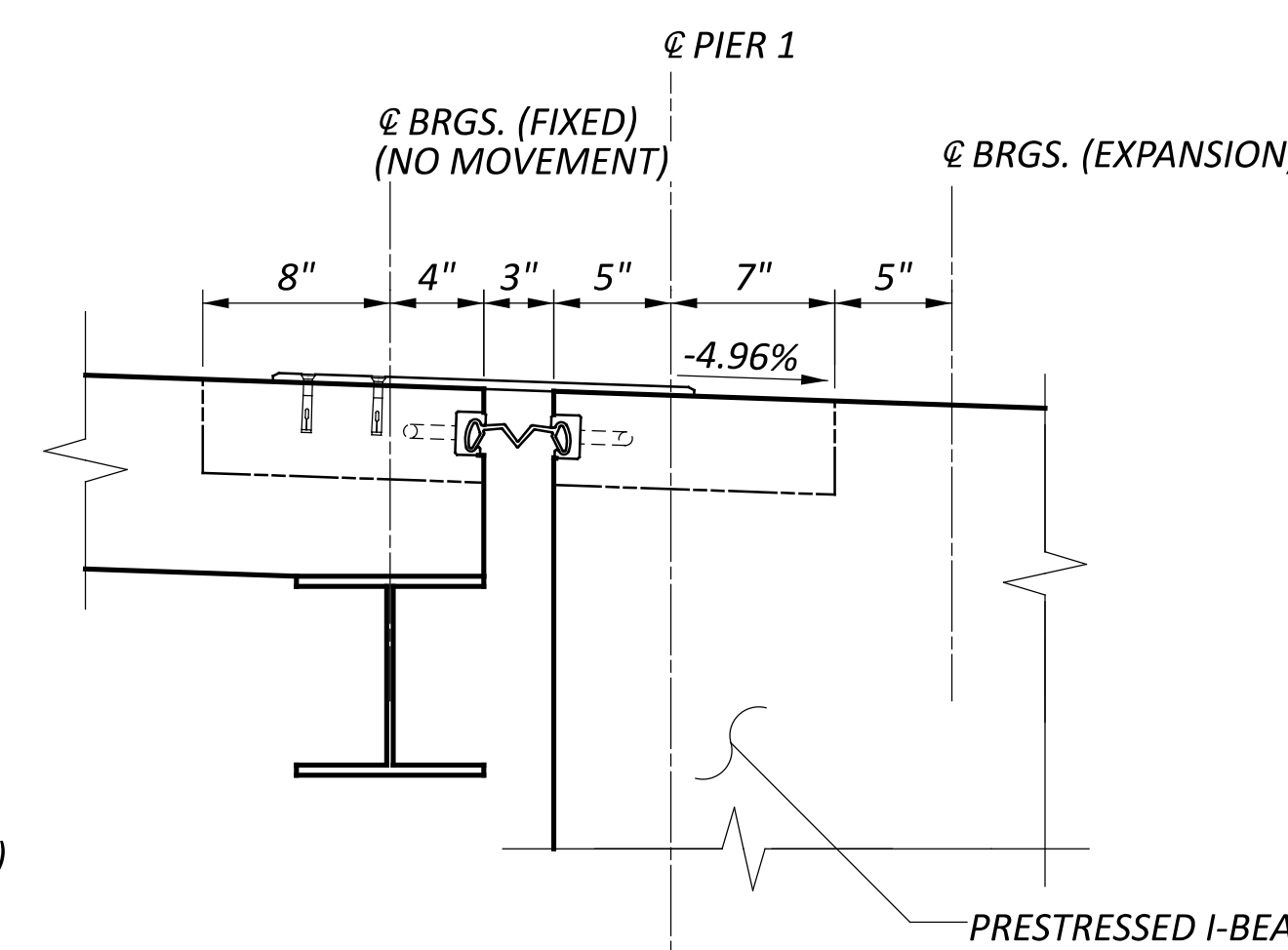
X SECTION 24
