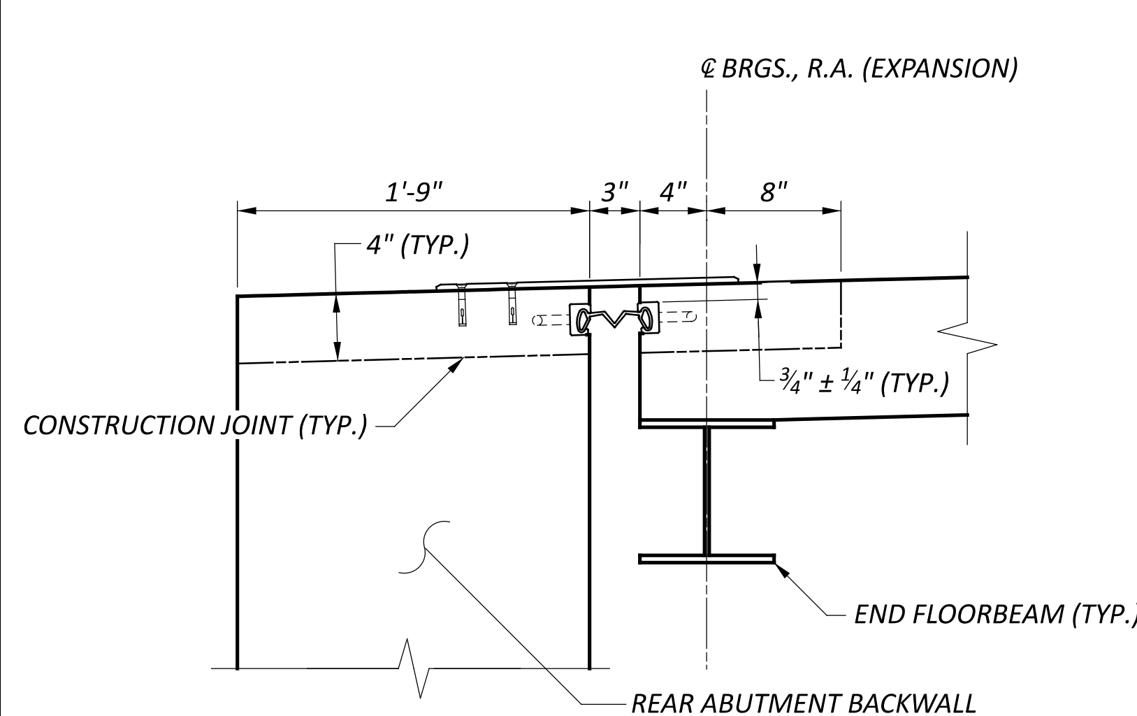
W SECTION 24
