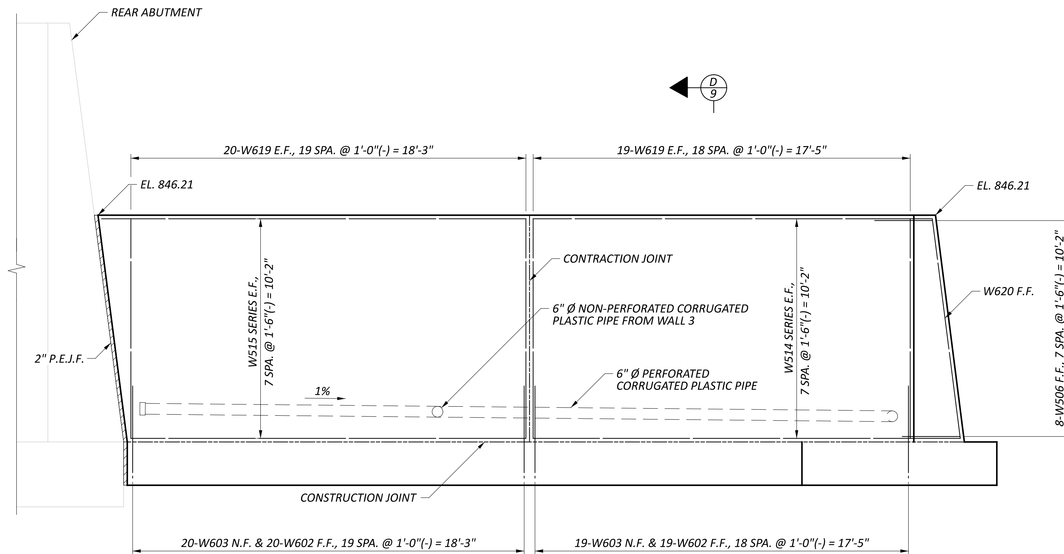
ELEVATION VIEWED ALONG BACK FACE
