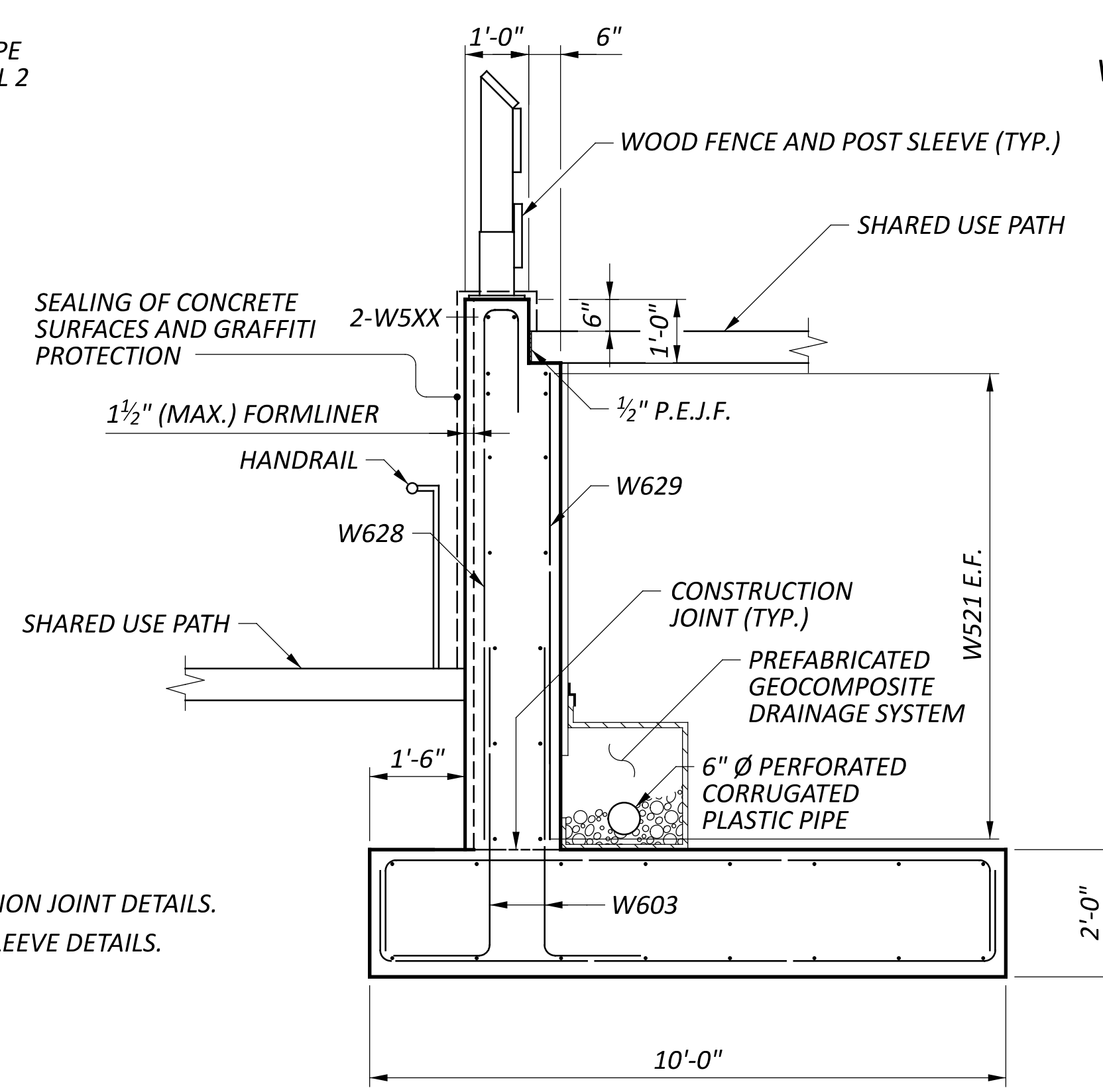
F SECTION 11
