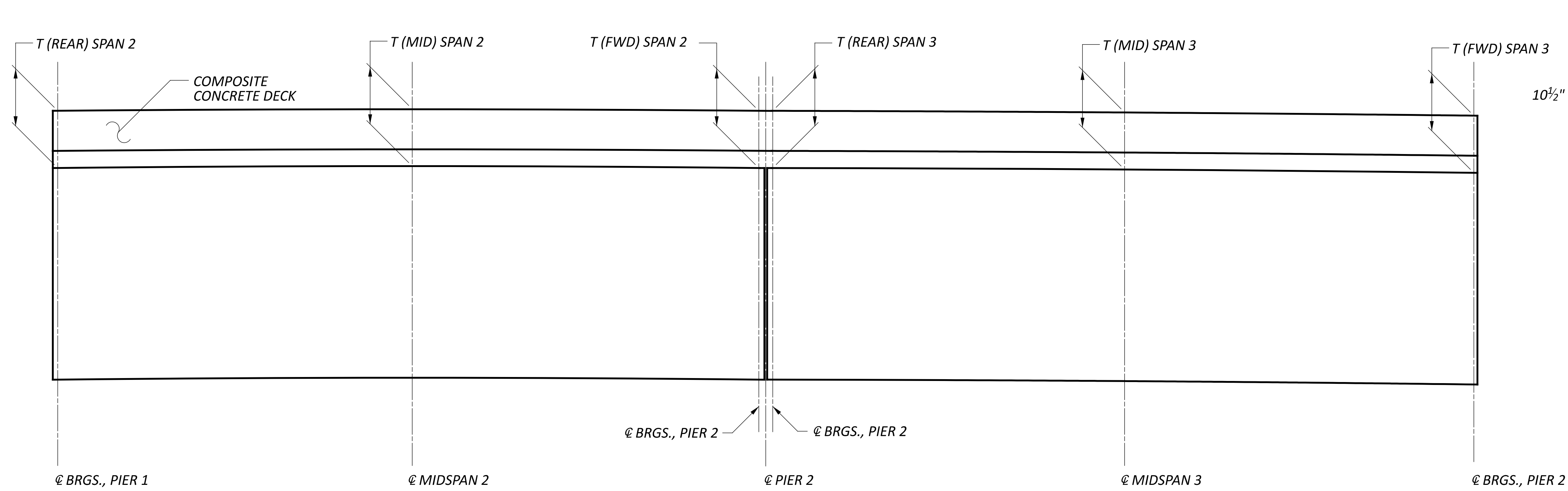
TOPPING DIAGRAM
