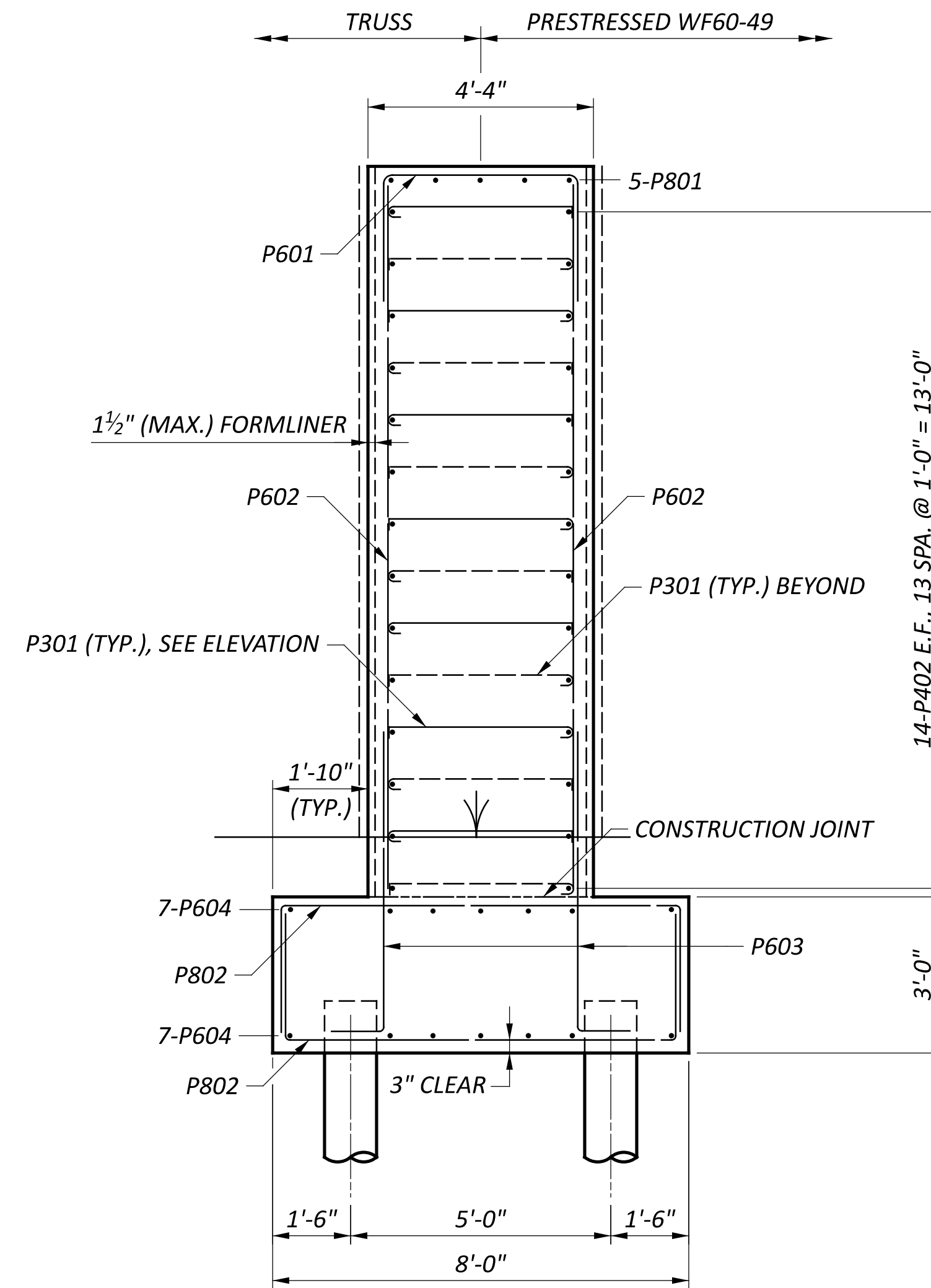
F SECTION 9
