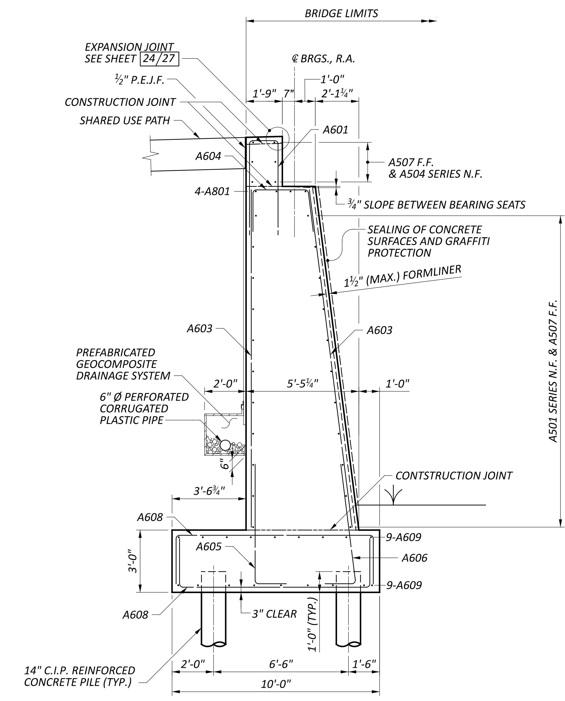
A SECTION
