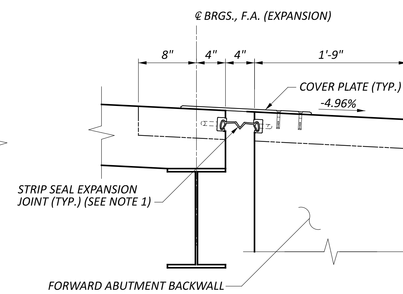
Z SECTION 24
