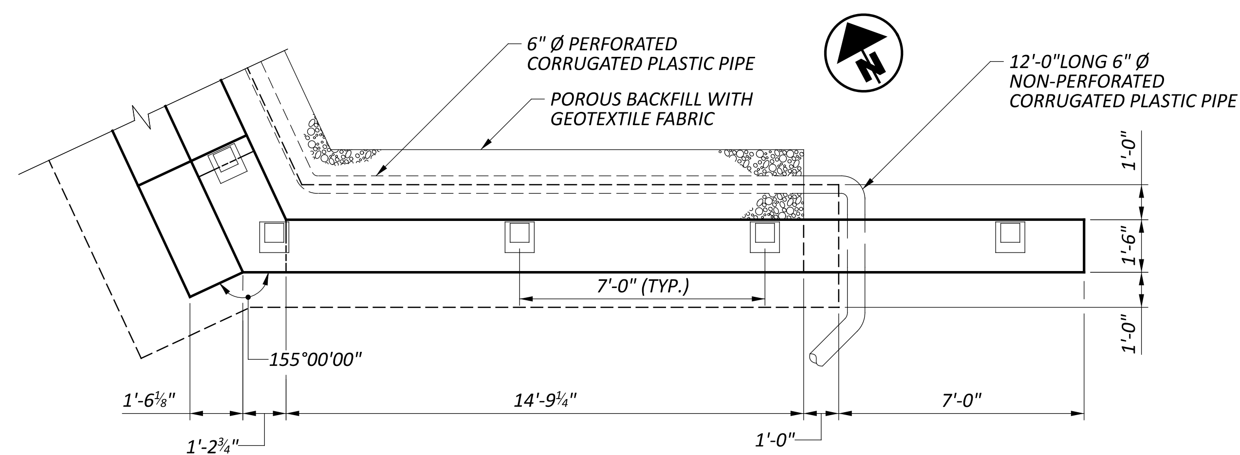
WINGWALL 4 PLAN
