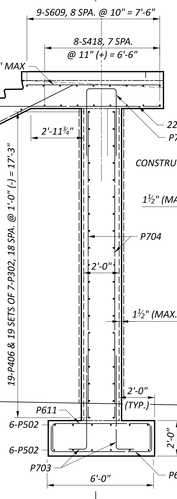
b SECTION 25
