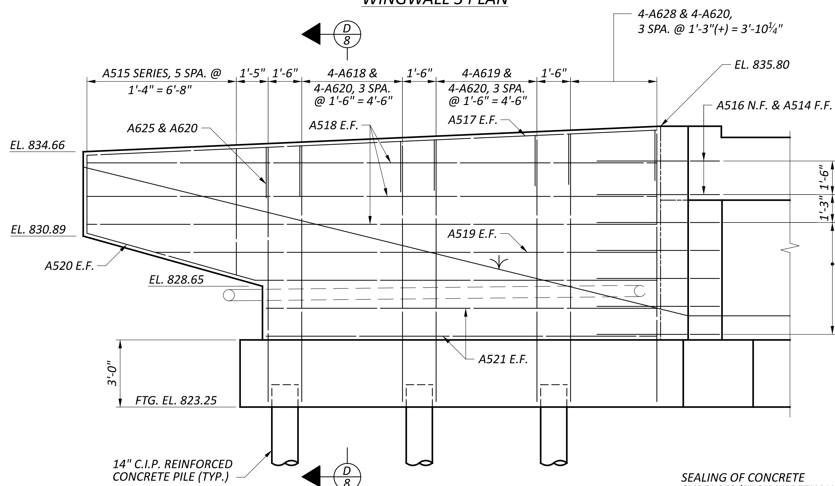
WINGWALL 3 PLAN
