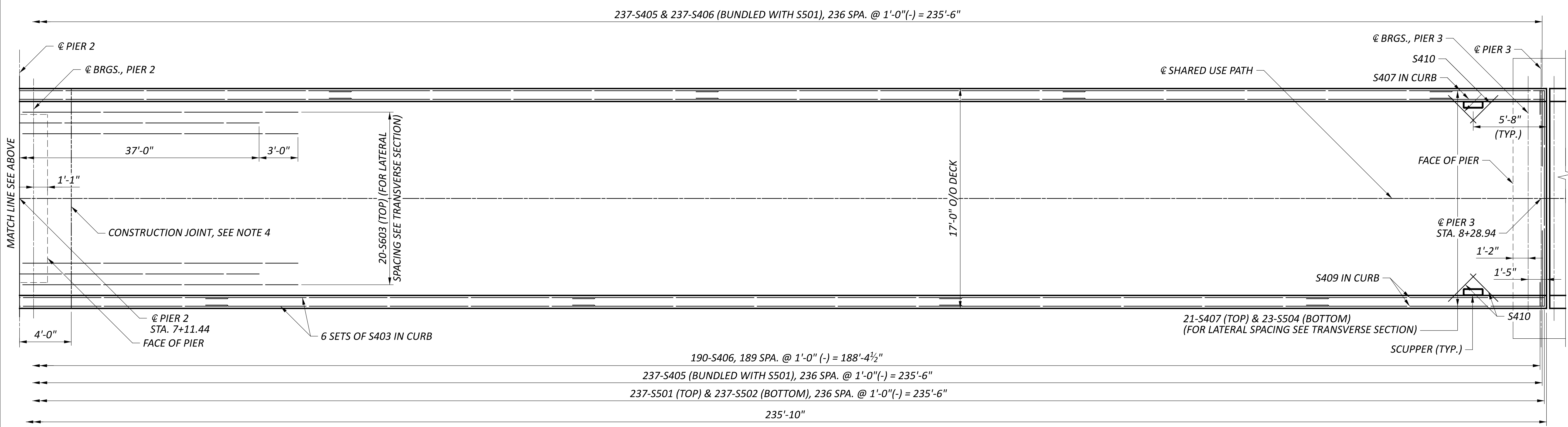
DECK PLAN - SPAN 3
