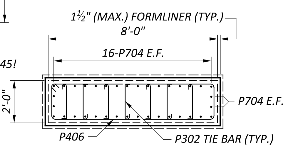
d SECTION 25
