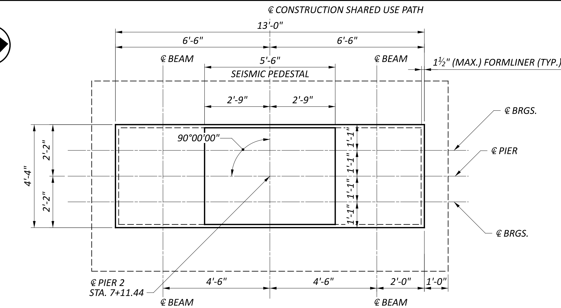
PLAN
