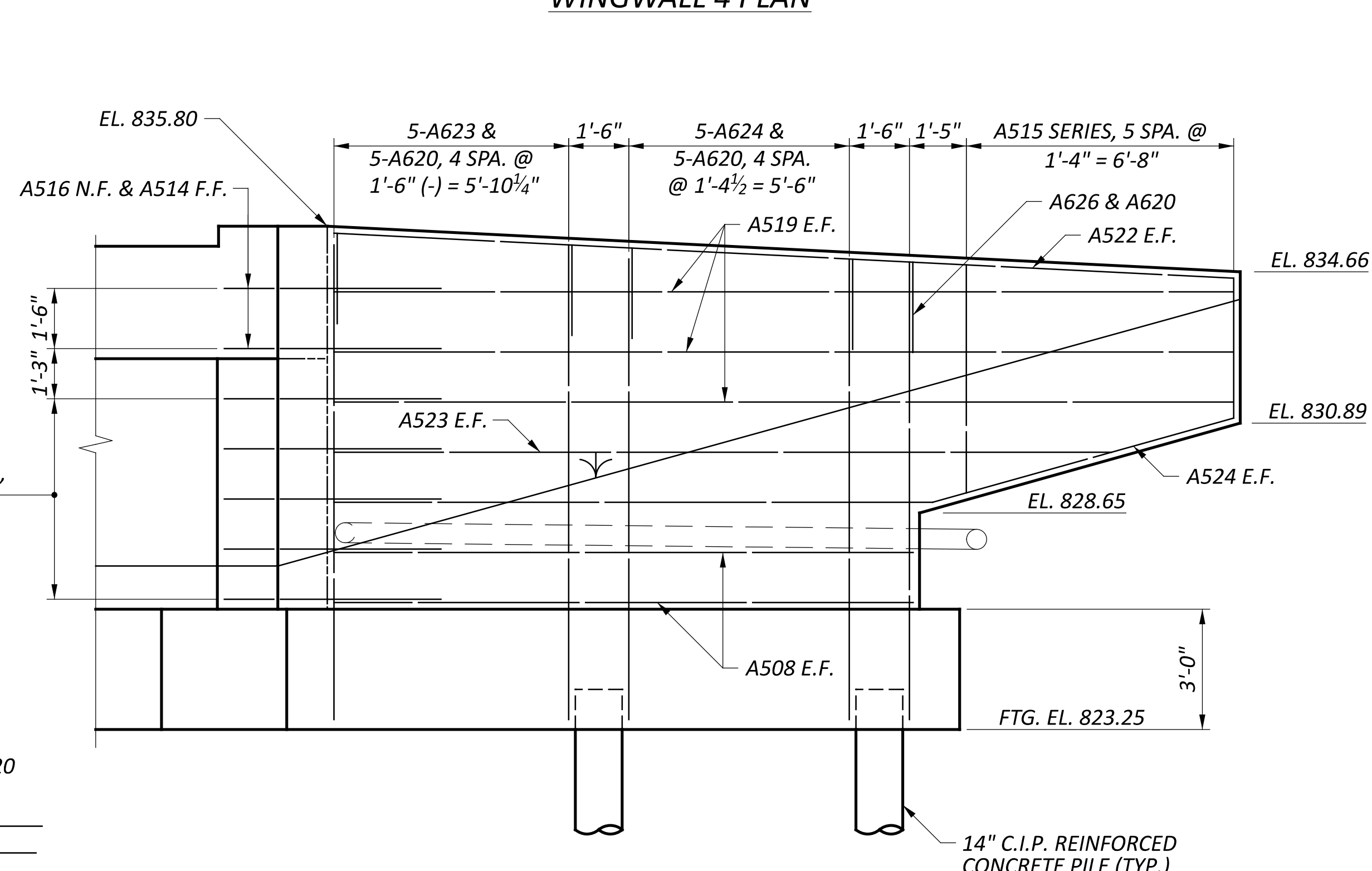
WINGWALL 4 PLAN
