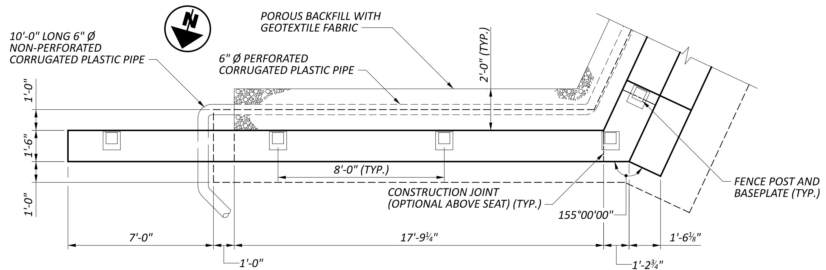
WINGWALL 3 PLAN
