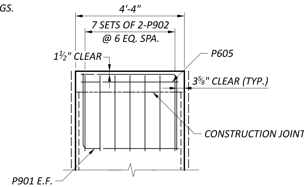
I SECTION 10
