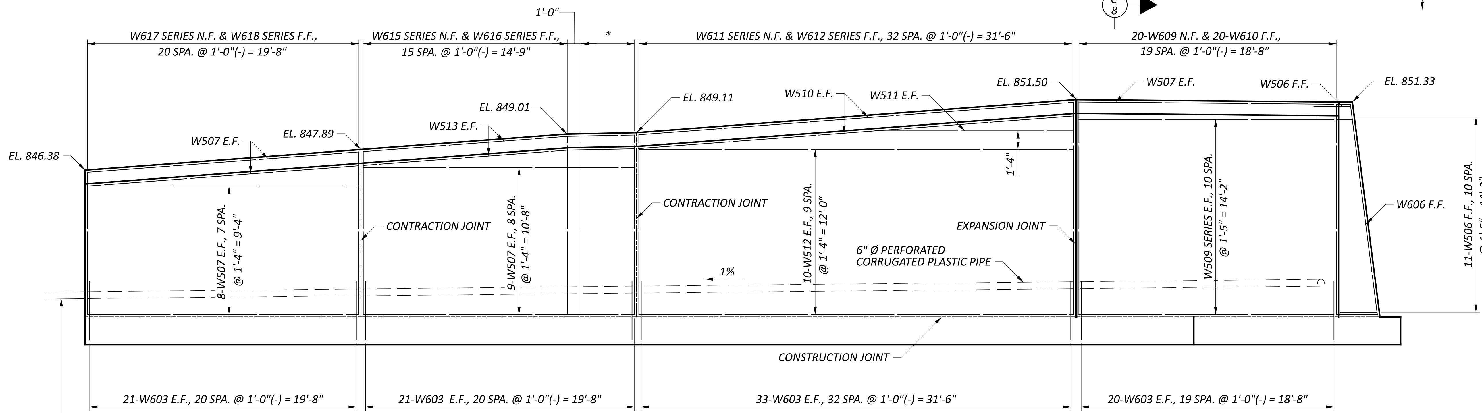
ELEVATION VIEWED ALONG BACK FACE
