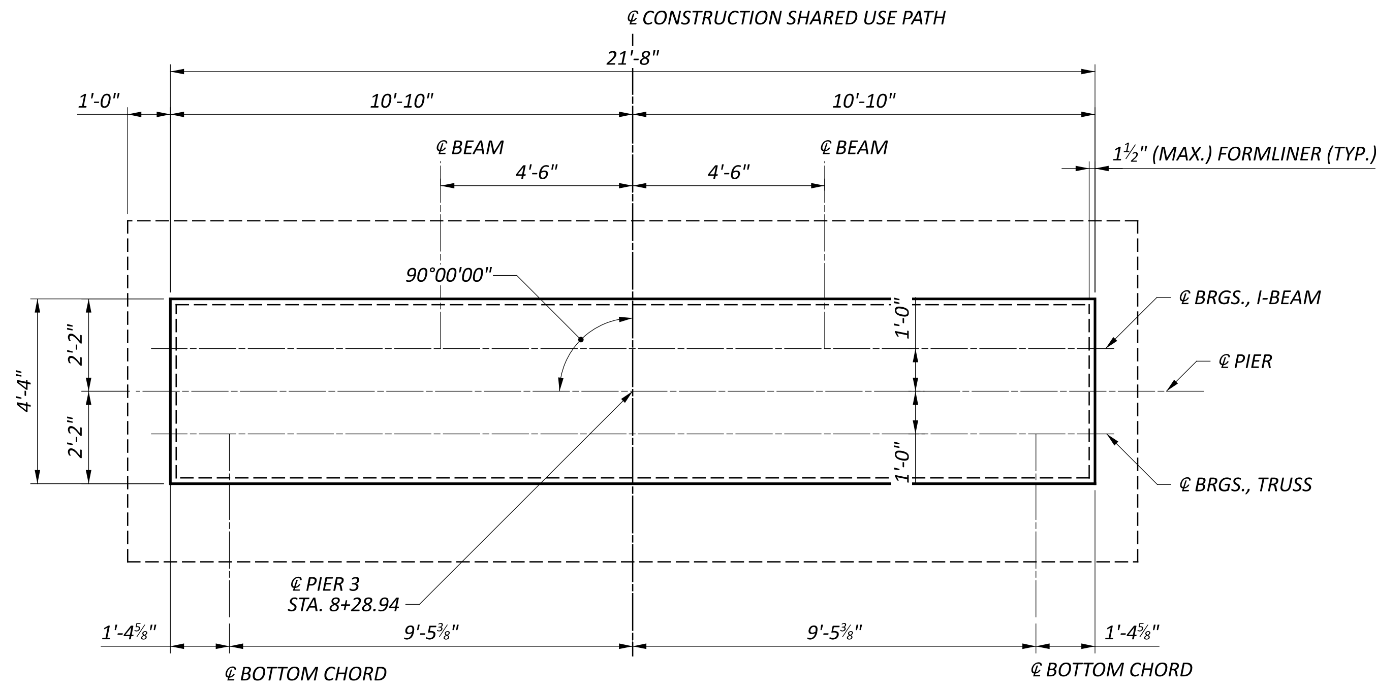
PLAN
