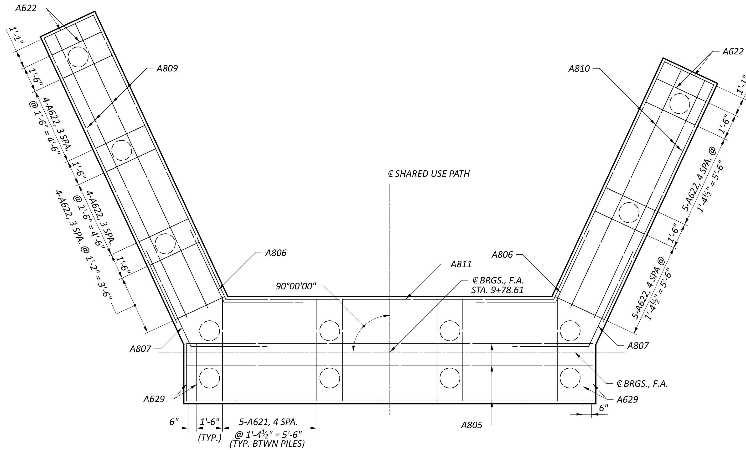
BOTTOM MAT REINFORCEMENT PLAN
