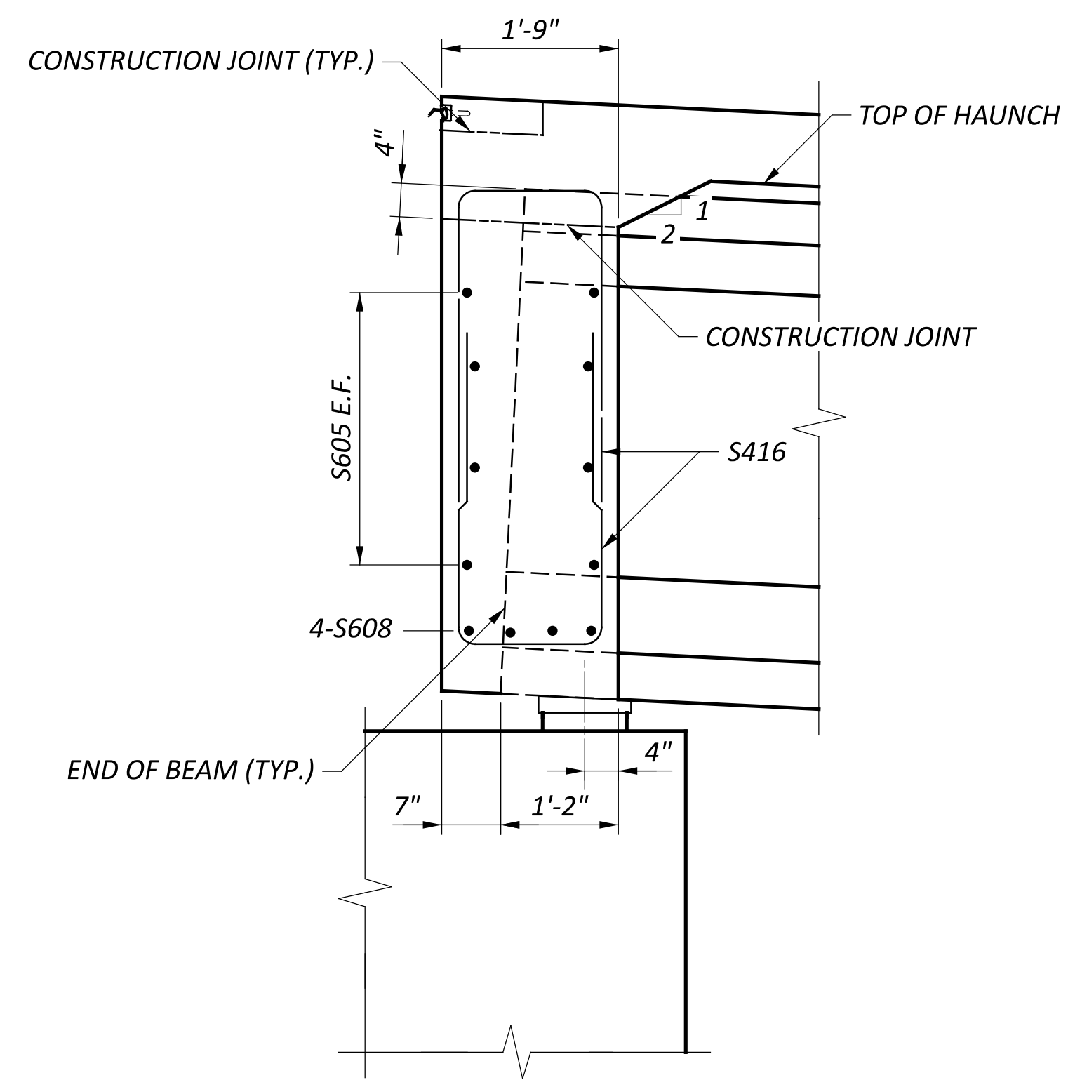
O SECTION 21 PIER 1 SHOWN
