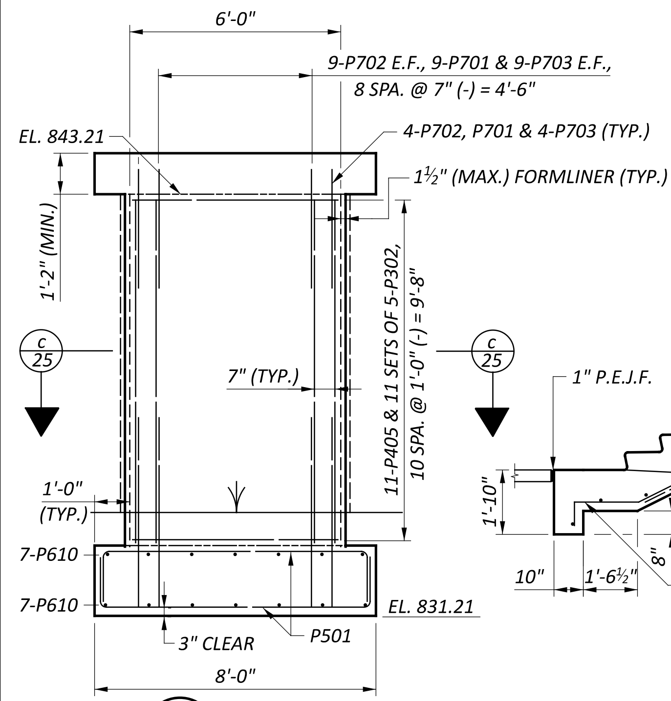
a SECTION 25
