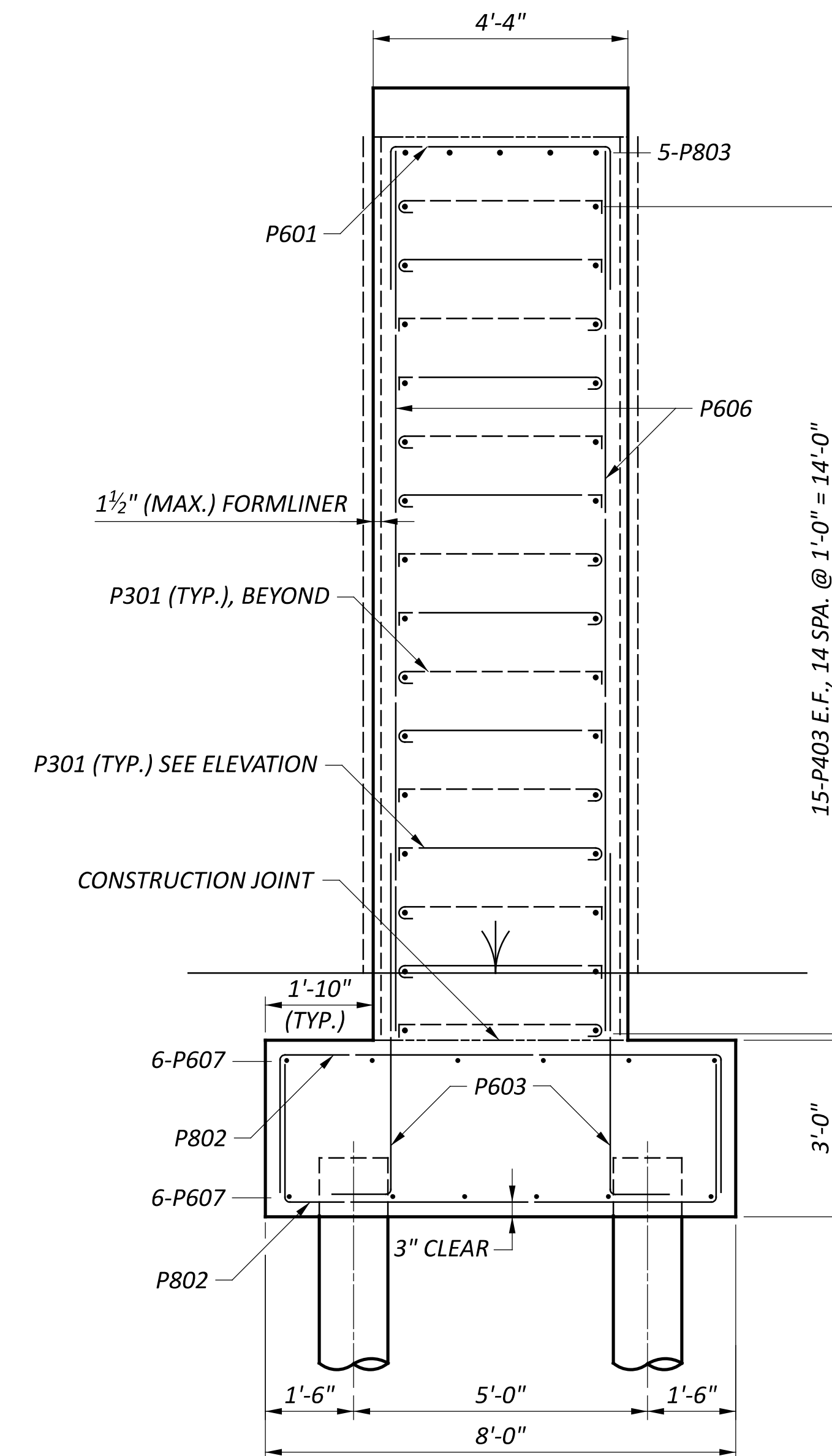
H SECTION 10
