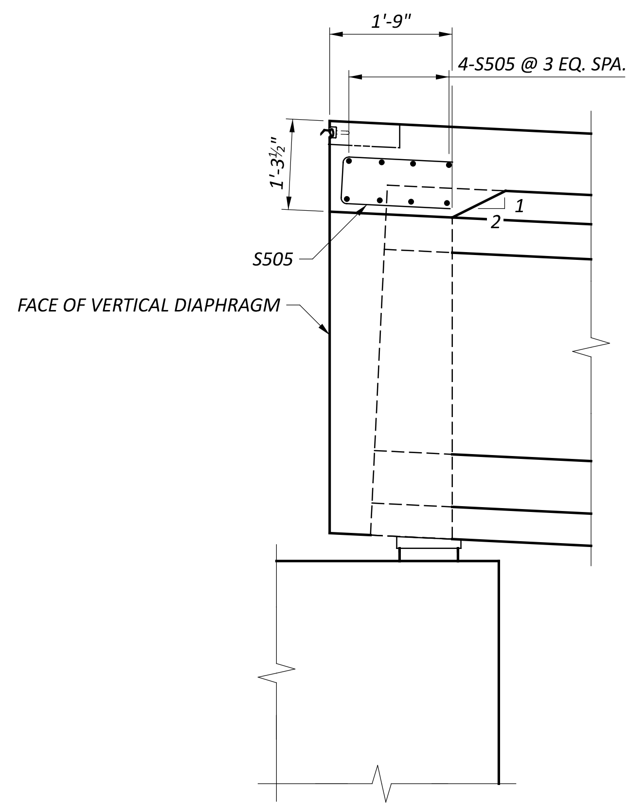
N SECTION 21 PIER 1 SHOWN, PIER 3 OPPOSITE HAND
