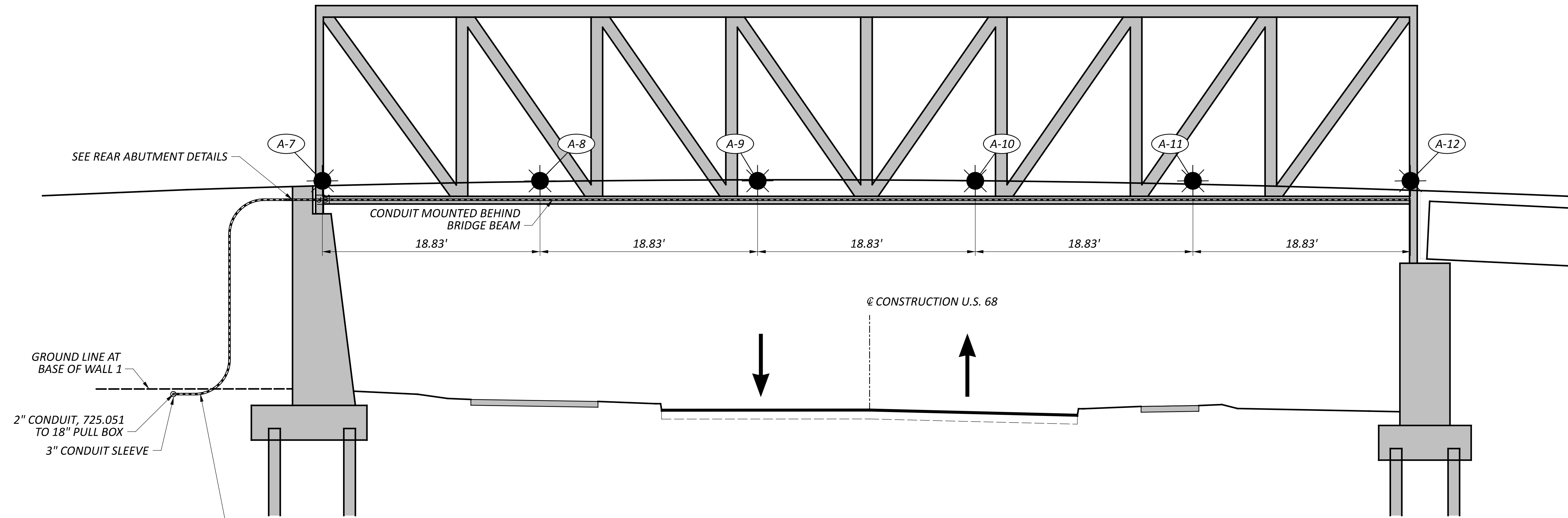
ELEVATION VIEW (LOOKING NORTH)
