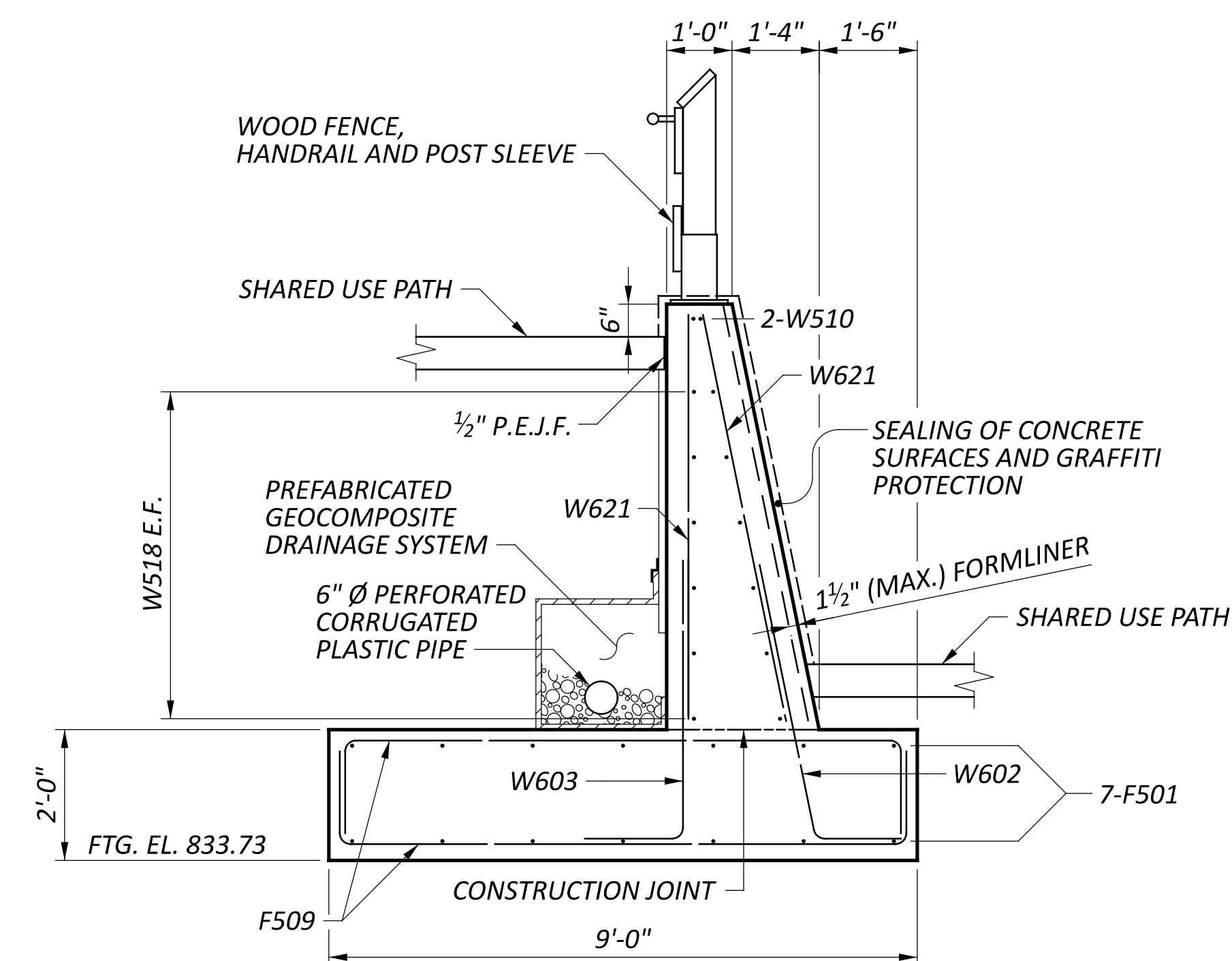
SECTION E 10
