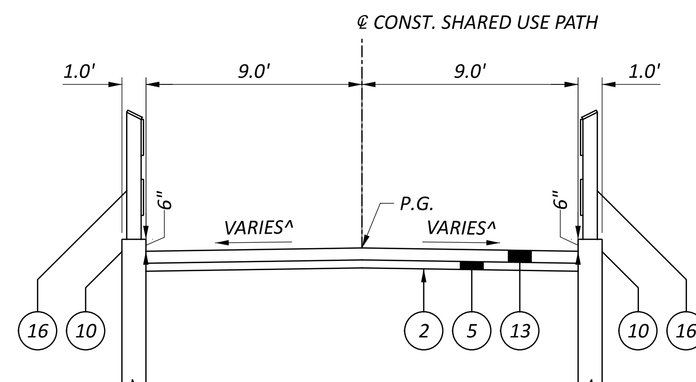
TYPICAL SECTION - SHARED USE PATH
