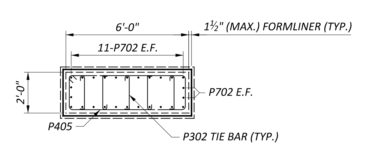
c SECTION 25
