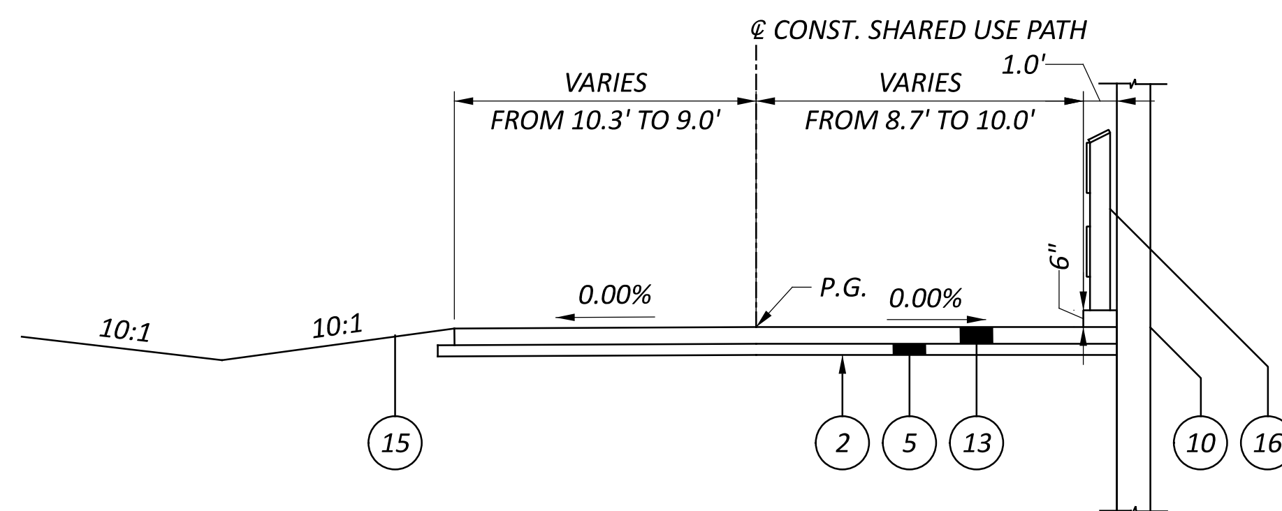
TYPICAL SECTION - SHARED USE PATH
