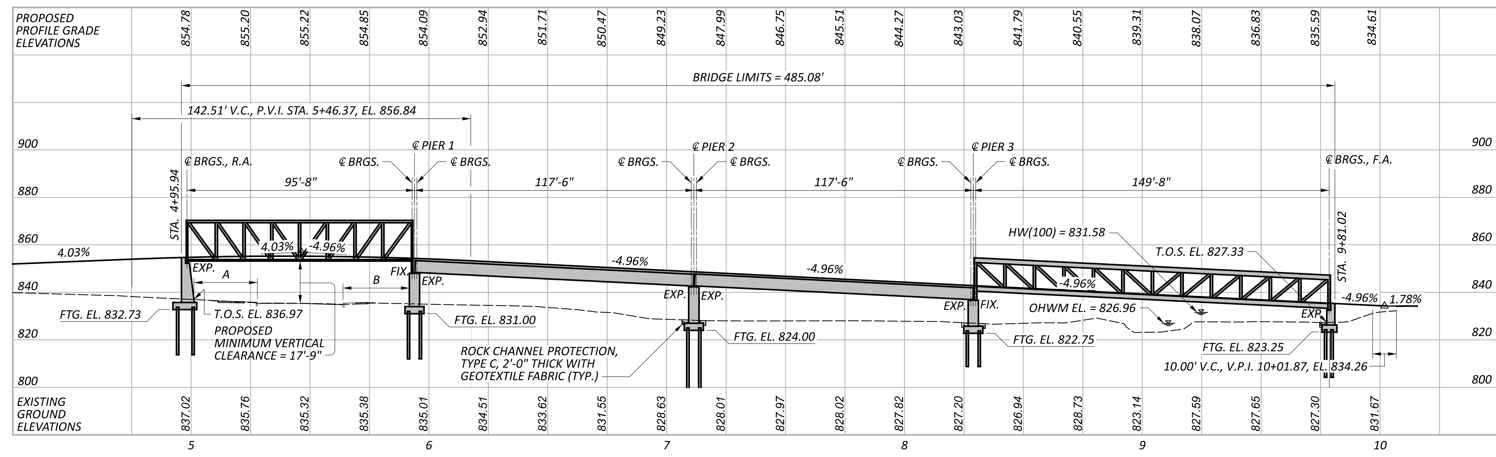
PROFILE ALONG @ CONSTRUCTION SHARED USE PATH
