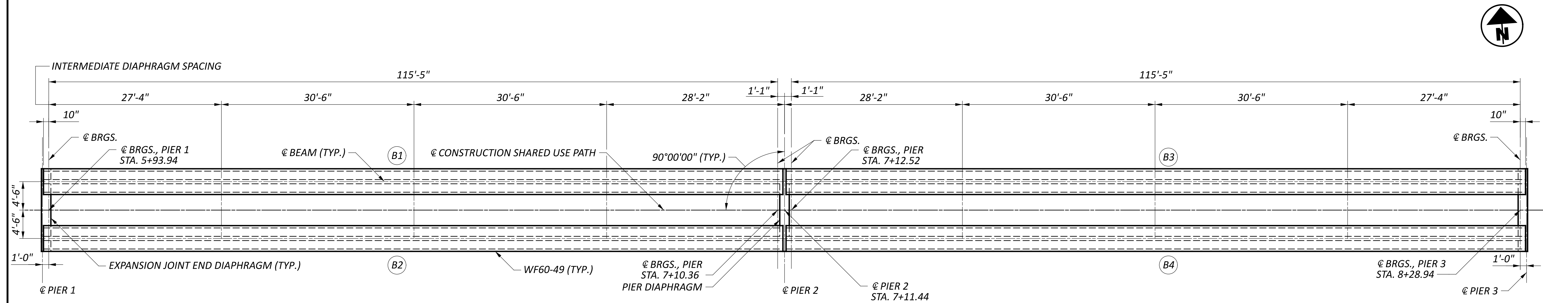
FRAMING PLAN
