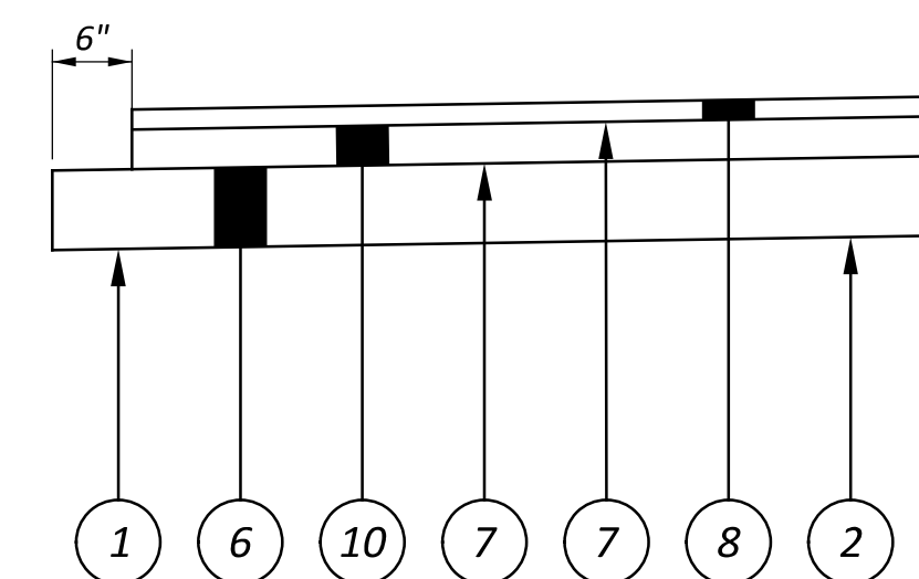
SHARED USE PATH STEP DETAIL
