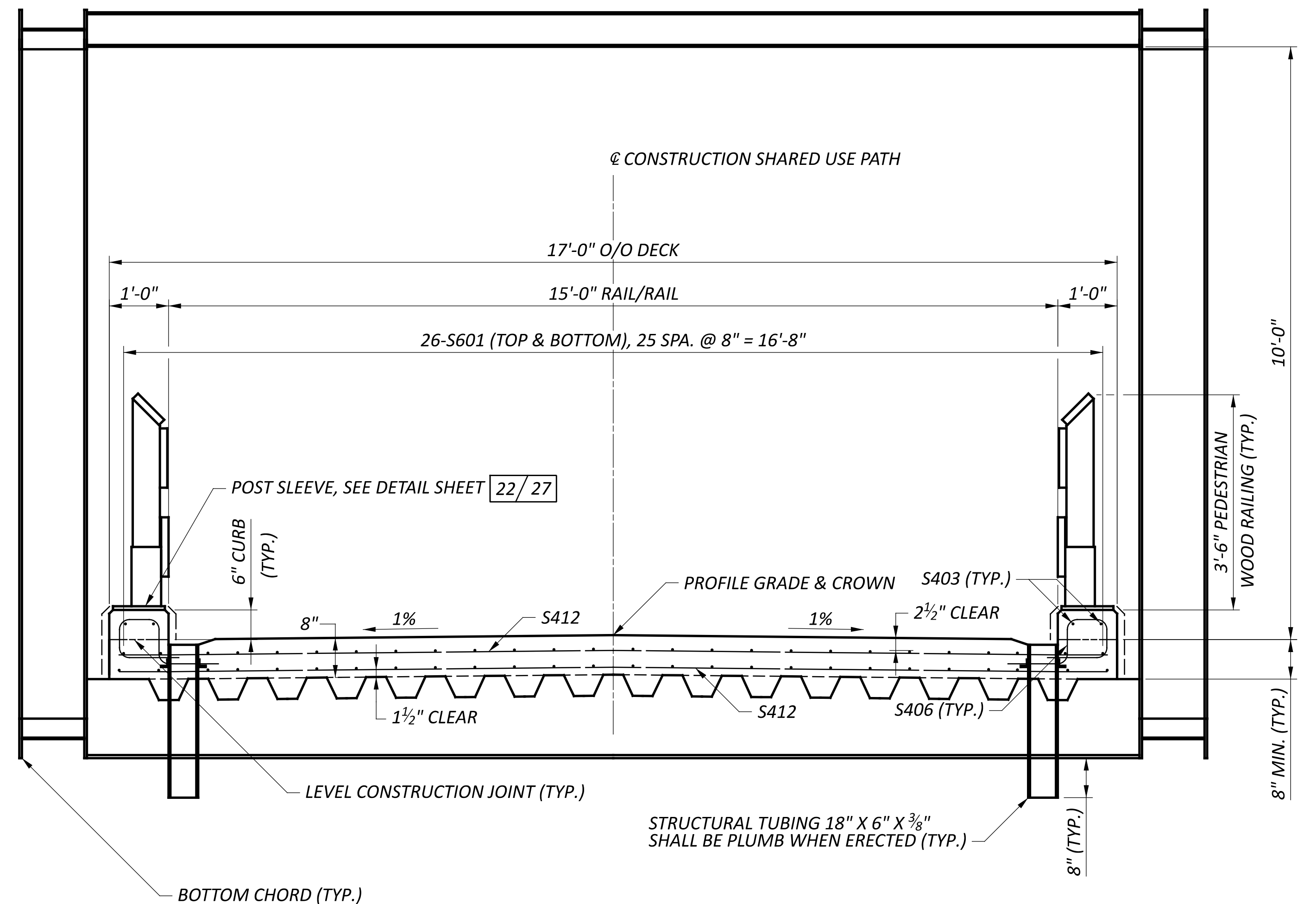
TRANSVERSE SECTION SPAN 4
