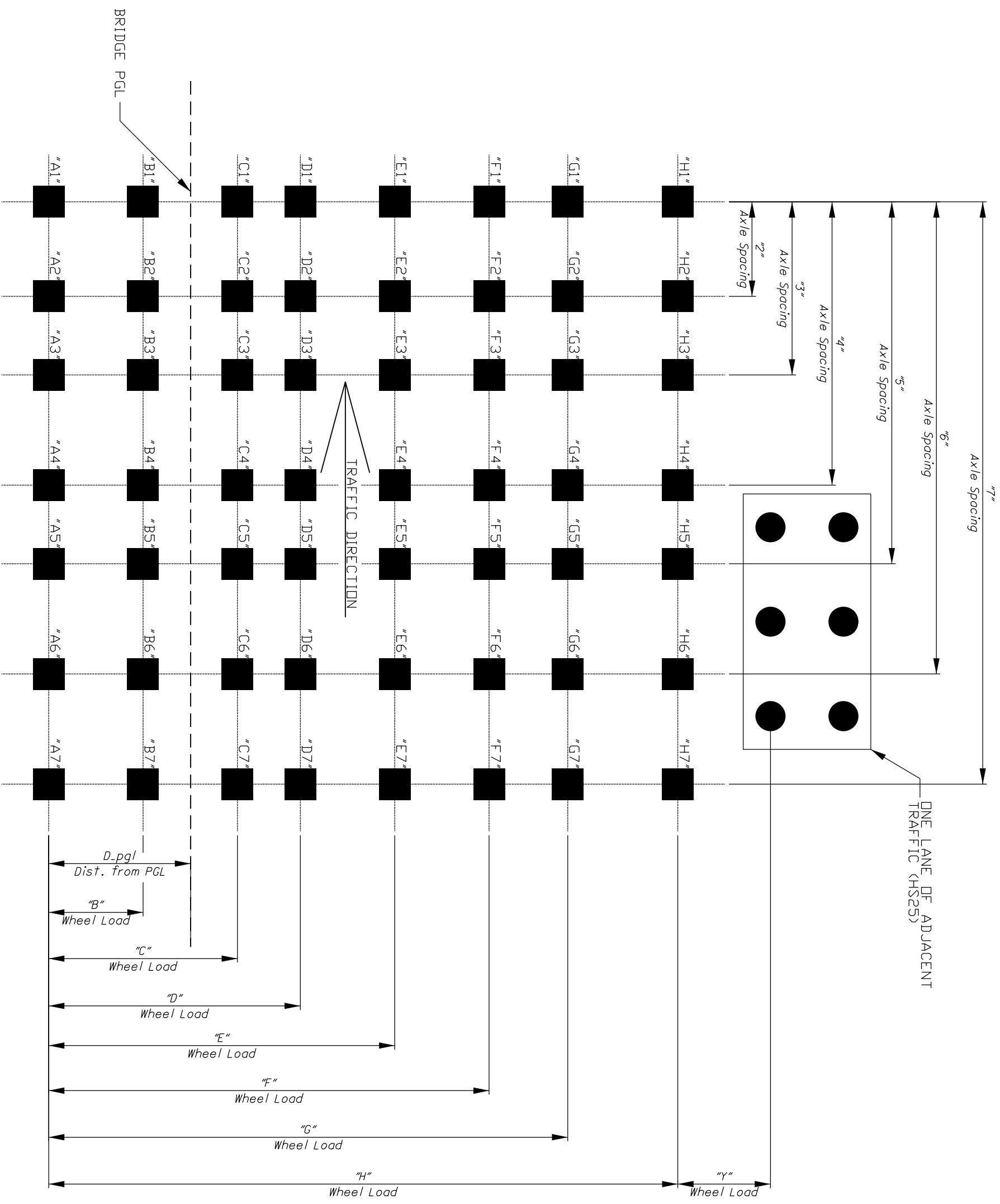
FIGURE 2-1: PERMIT VEHICLE WHEEL CONFIGURATIONS
