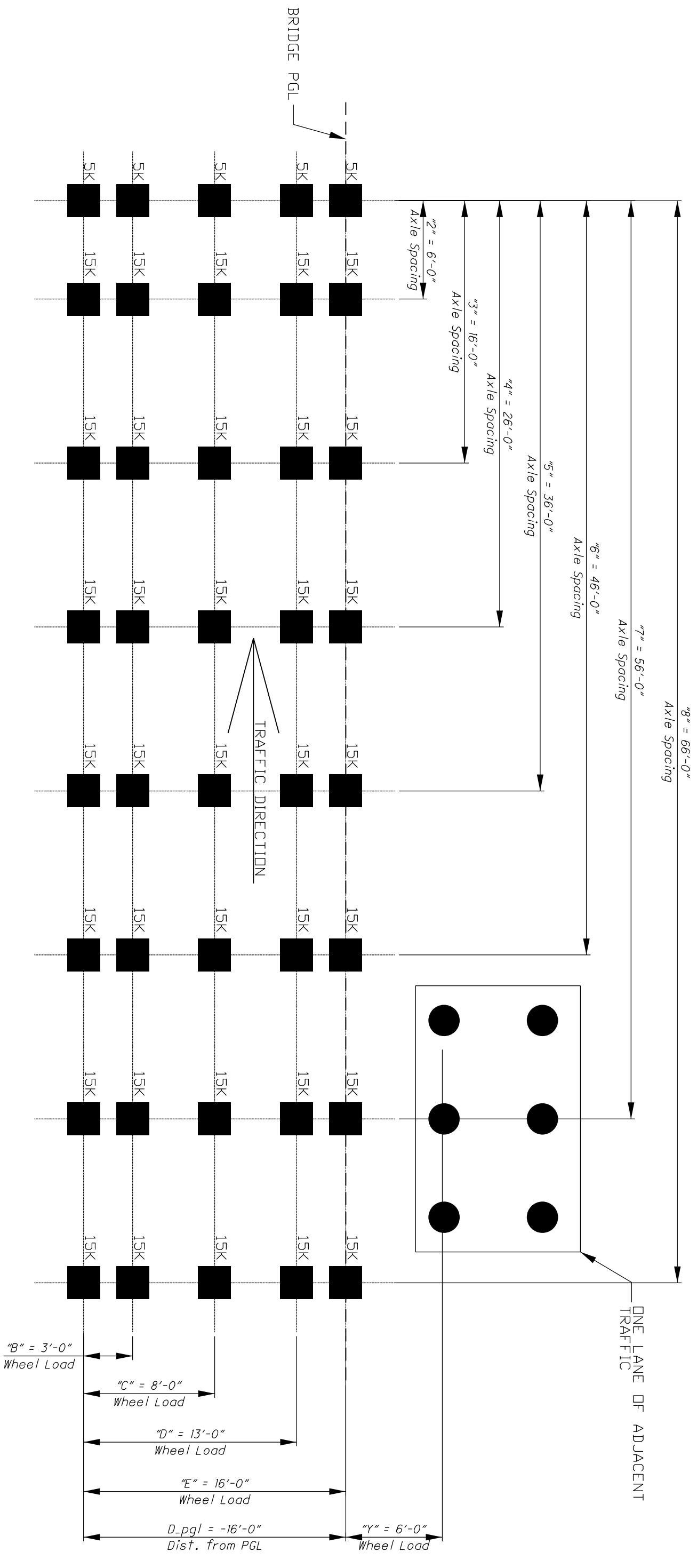
FIGURE 5-2: PERMIT (USER DEFINED) WHEEL CONFIGURATION FOR EXAMPLE 2
