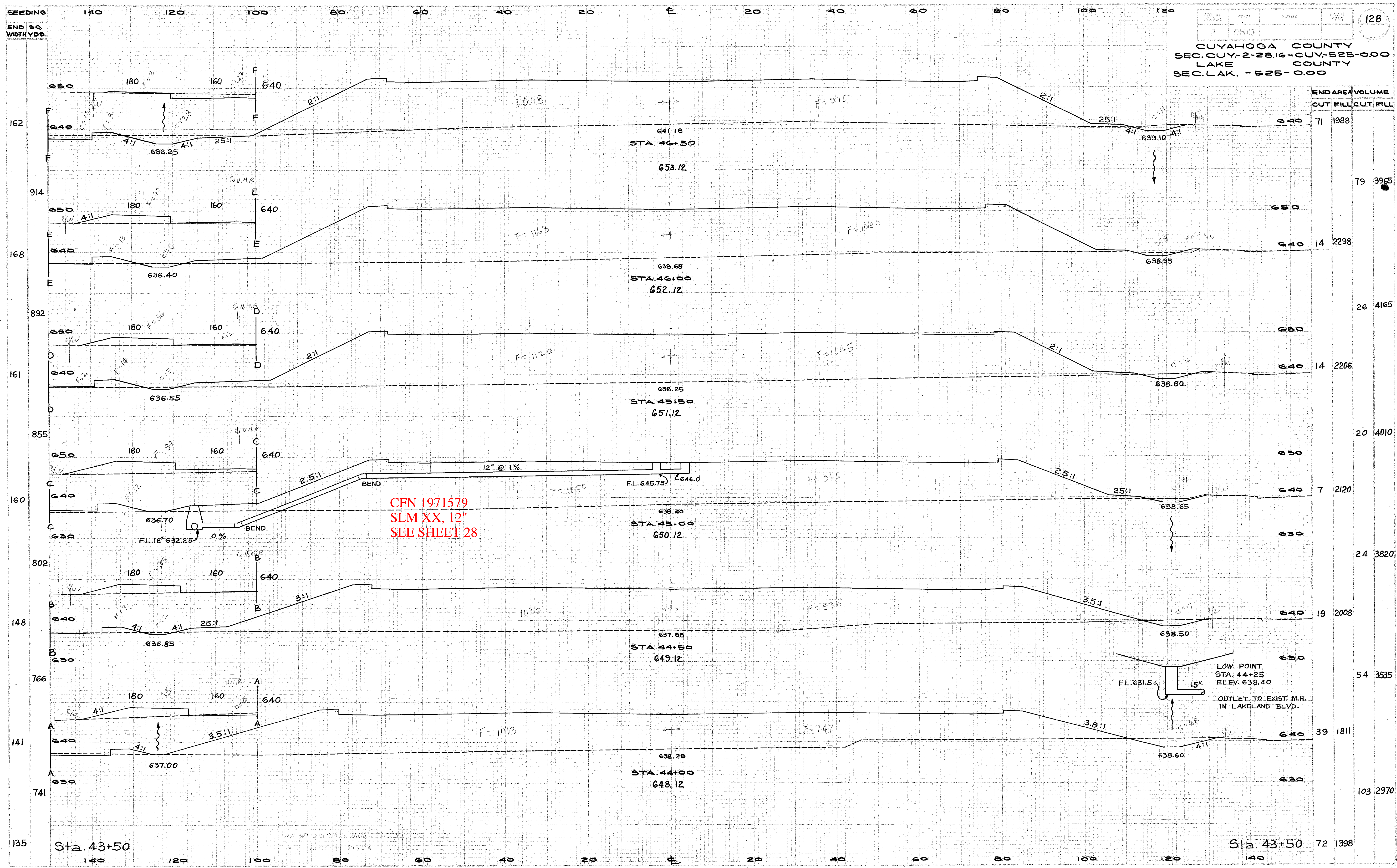
LAKELAND FREEWAY CROSS SECTION STA. 44+00 TO STA. 46+50
