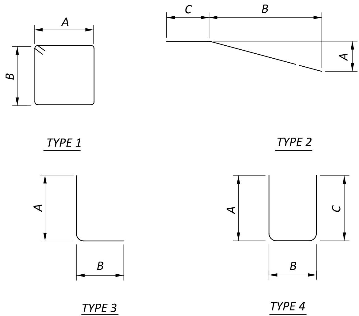
BENDING DIAGRAMS
