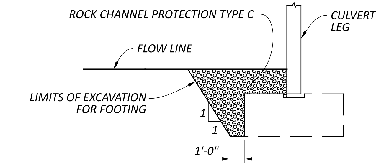
ROCK CHANNEL PROTECTION INSIDE CULVERT
