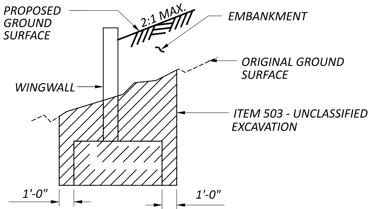
LIMITS OF UNCLASSIFIED EXCAVATION ON WINGWALL
