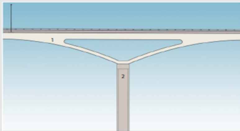
MAIN SPAN PIER SIDE ELEVATION (PIERS 3-11)
