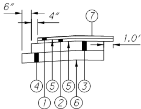
BASE AND SUBBASE STEP DETAIL
