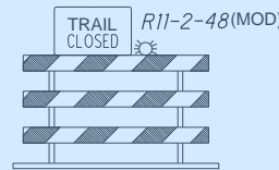
10' TYPE III SOLID BARRICADE
