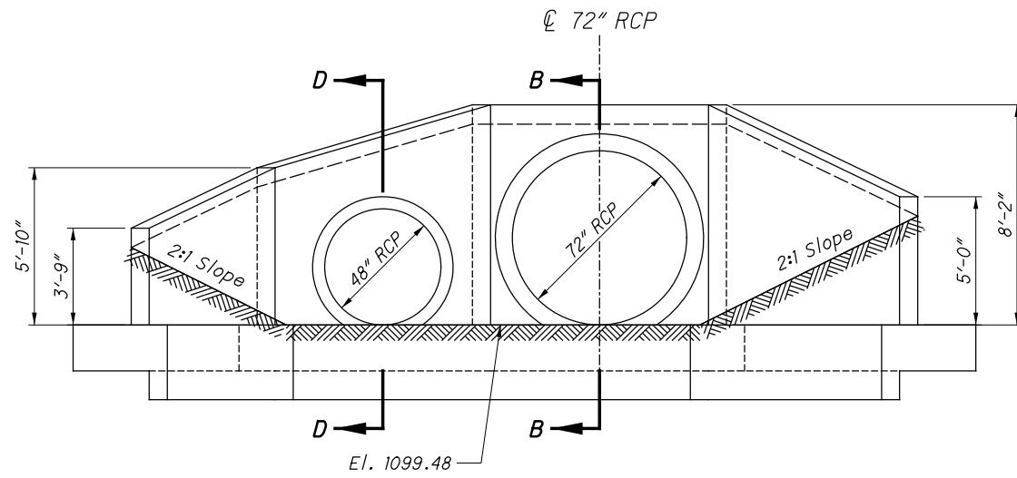
ELEVATION VIEW
