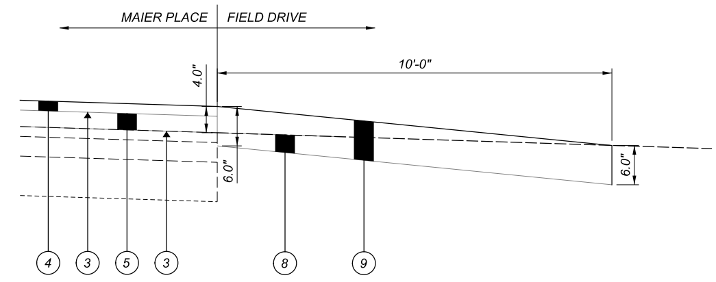
AGGREGATE (FIELD DRIVE) DRIVEWAY TRANSITION DETAIL
