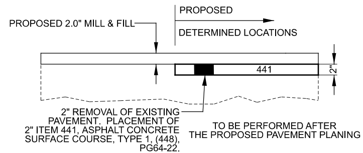
PARTIAL DEPTH PAVEMENT REPAIR, (441) 2" DETAIL
