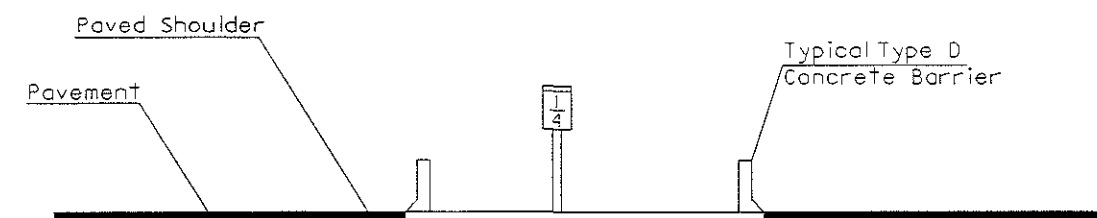
Double Median Barrier
