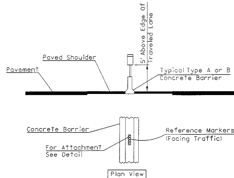
Single Median Barrier
