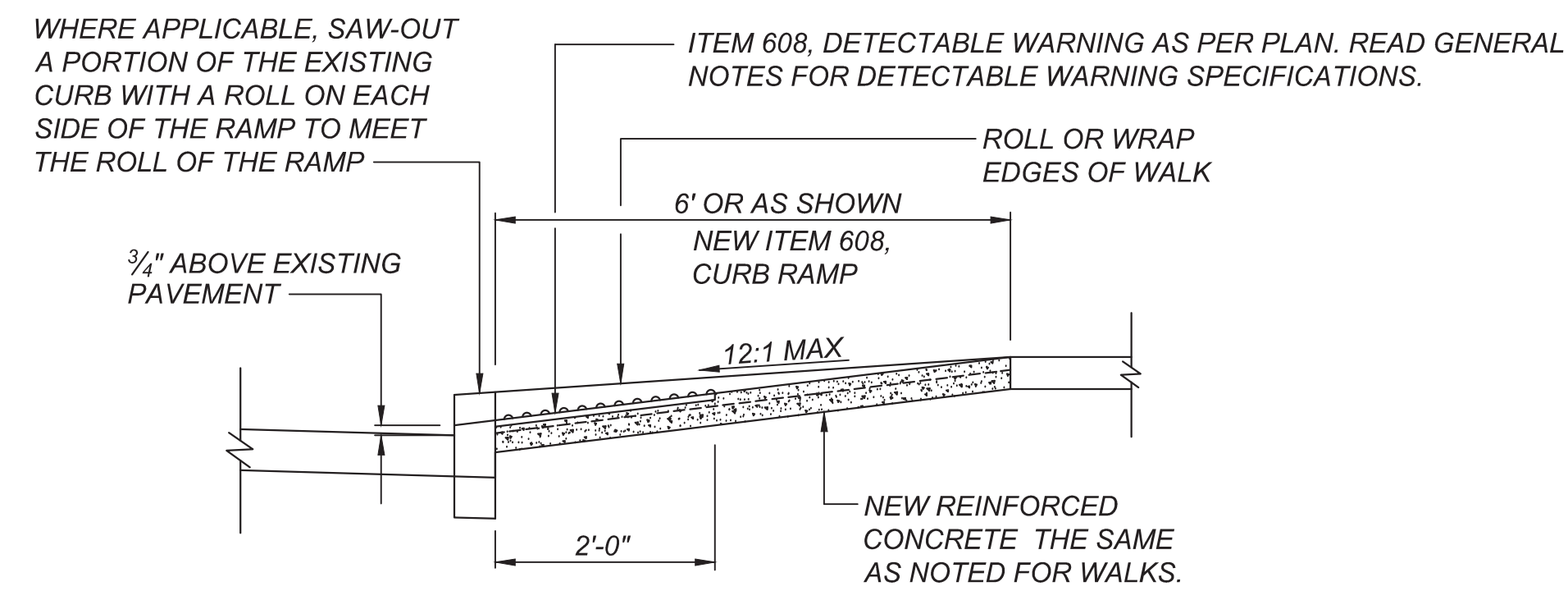
TYPICAL SECTION THRU NEW HANDICAP ITEM 608, CURB RAMPS NO SCALE
