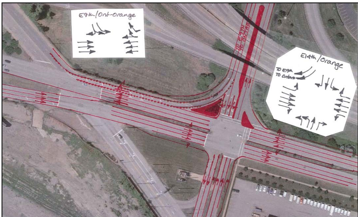
Figure 3.5 Conceptual Reconfiguration of E.14 th Street/Orange
