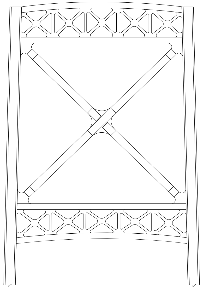
Tower C - East Elevation (Upper)
