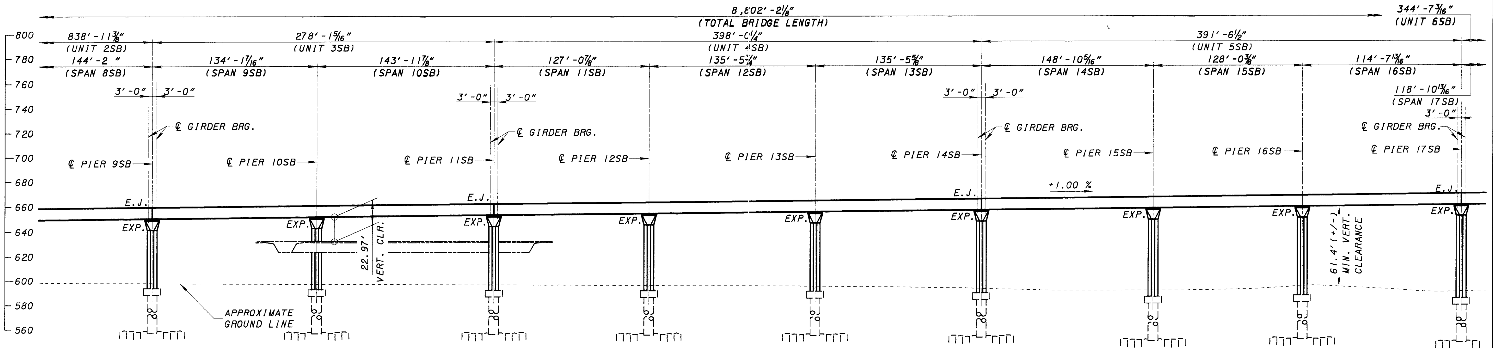
ELEVATION (STATIONS AND SPAN LENGTHS SHOWN ARE TAKEN ALONG \phi SURVEY & \phi CONSTRUCTION I-280)
