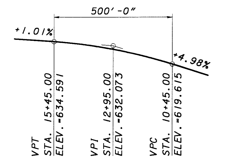
VERTICAL CURVE DIAGRAM
