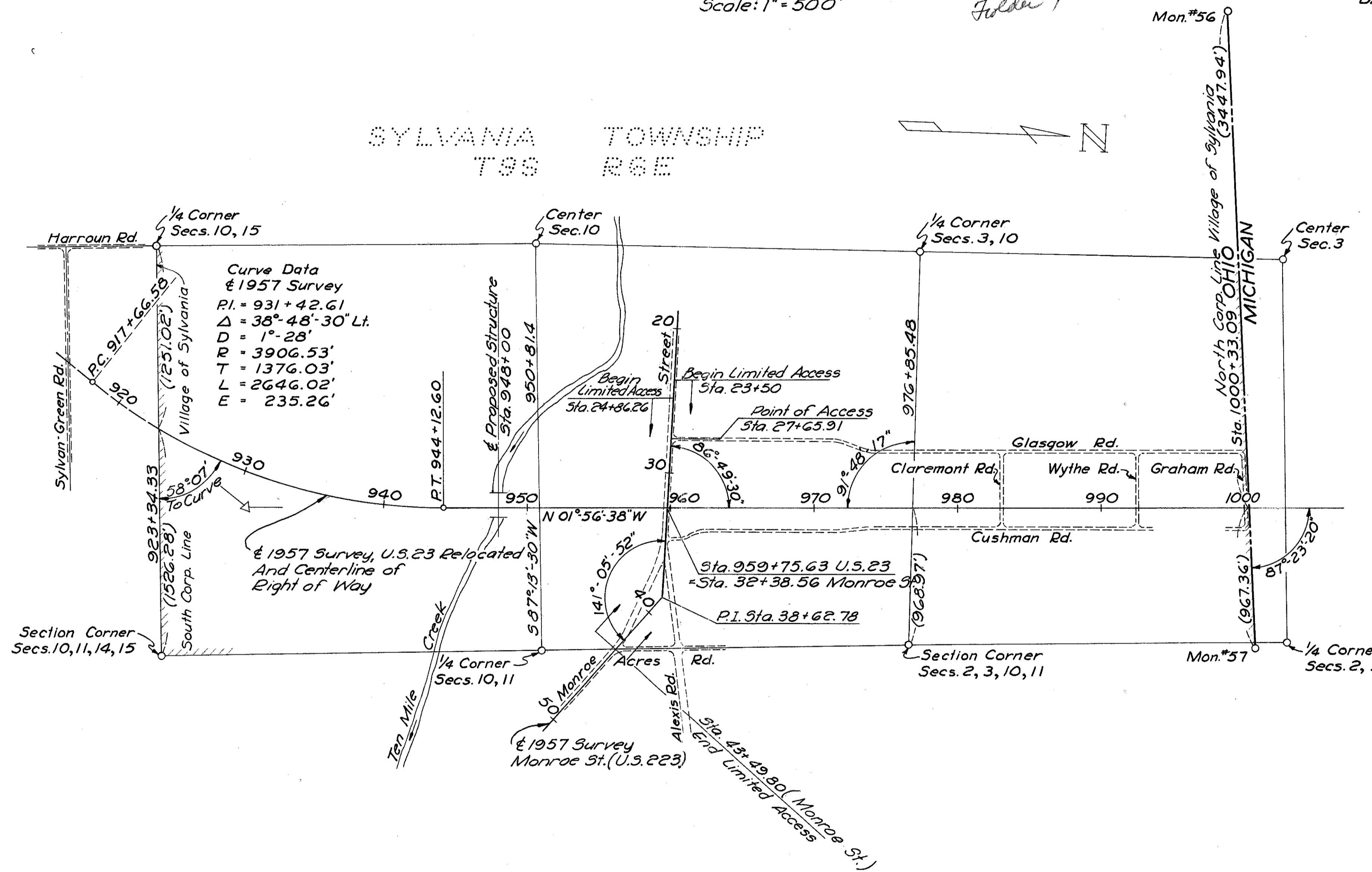
CENTERLINE REFERENCE MONUMENTS TO BE SET AFTER CONSTRUCTION
