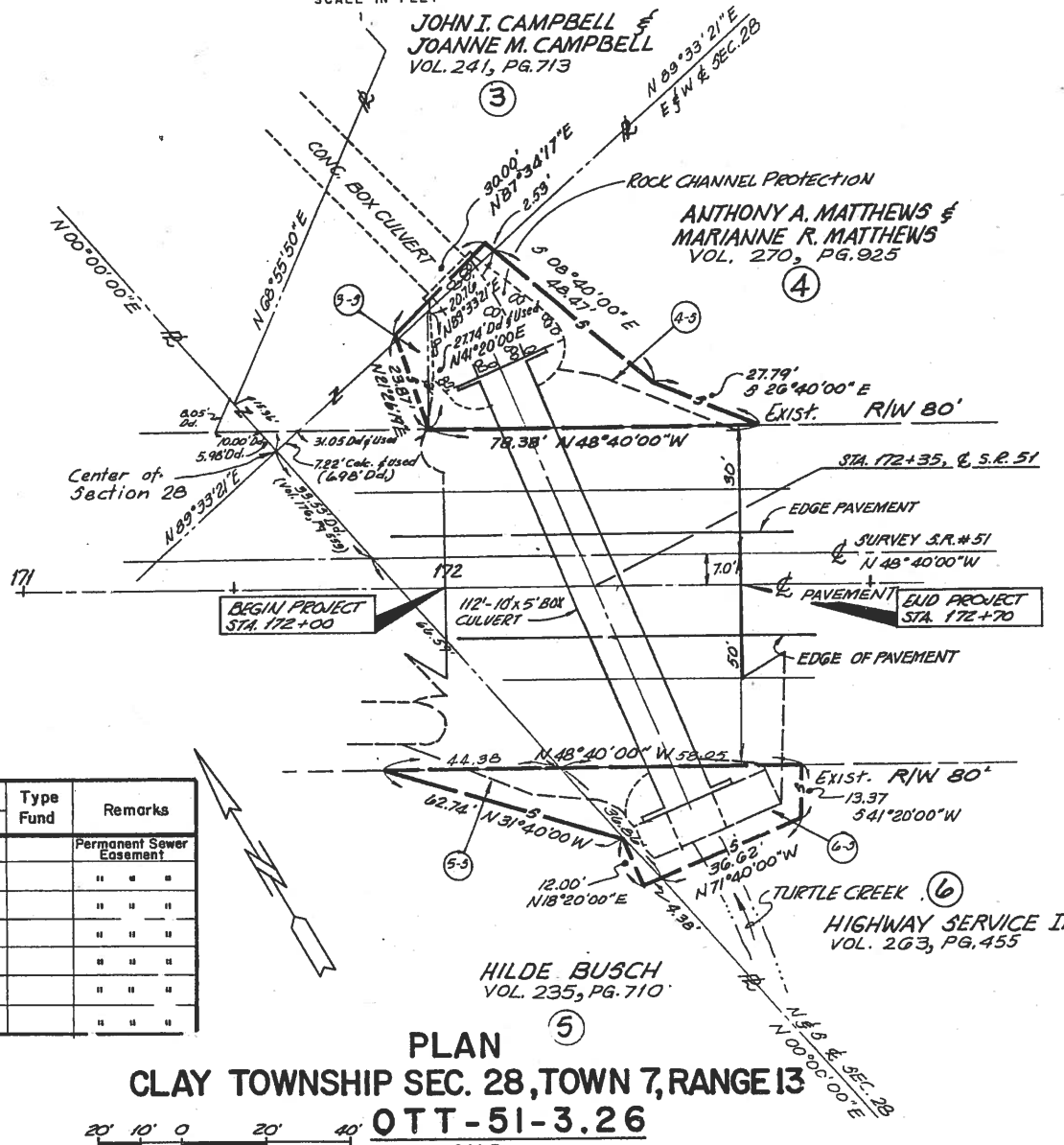
LOCATION PLAN OTT-51-3.26
