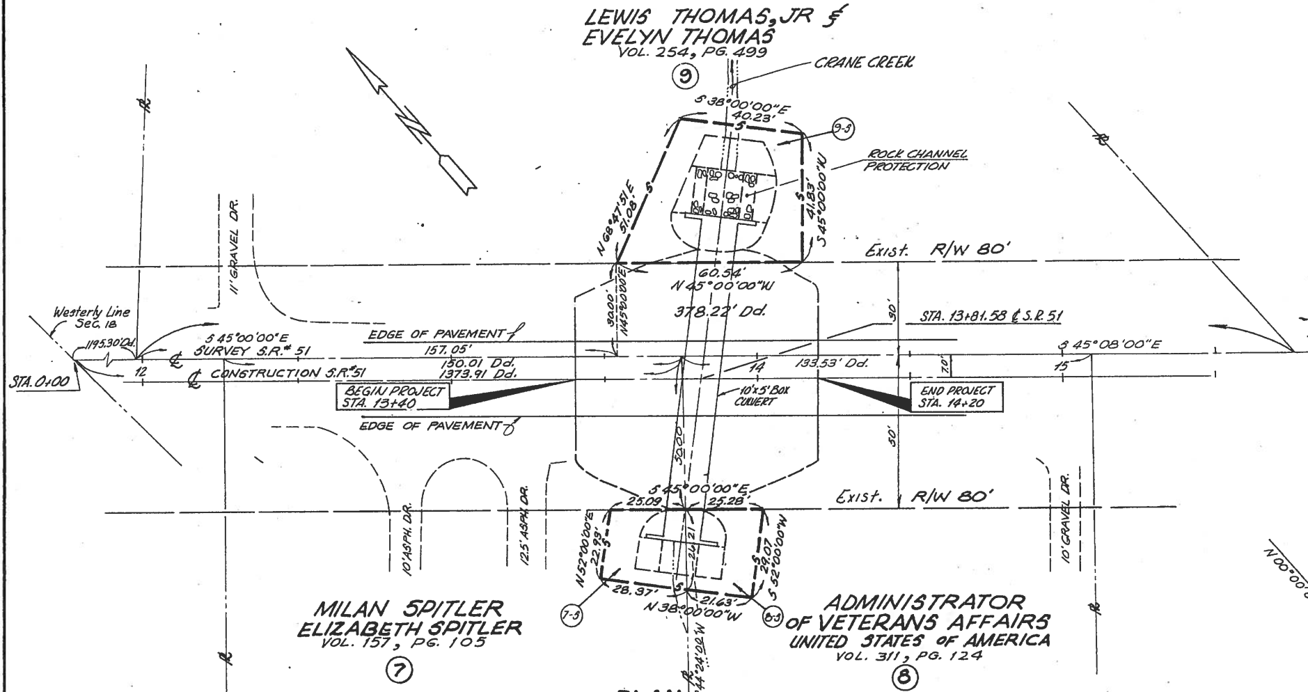
PLAN ALLEN TOWNSHIP SEC. 18, TOWN 7, RANGE 13 OTT-51-0.25
