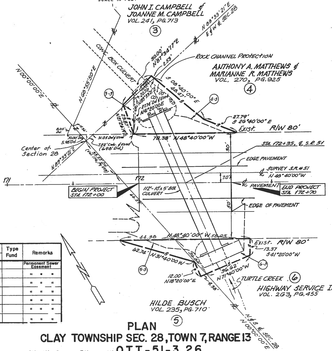
LOCATION PLAN OTT-51-3.26
