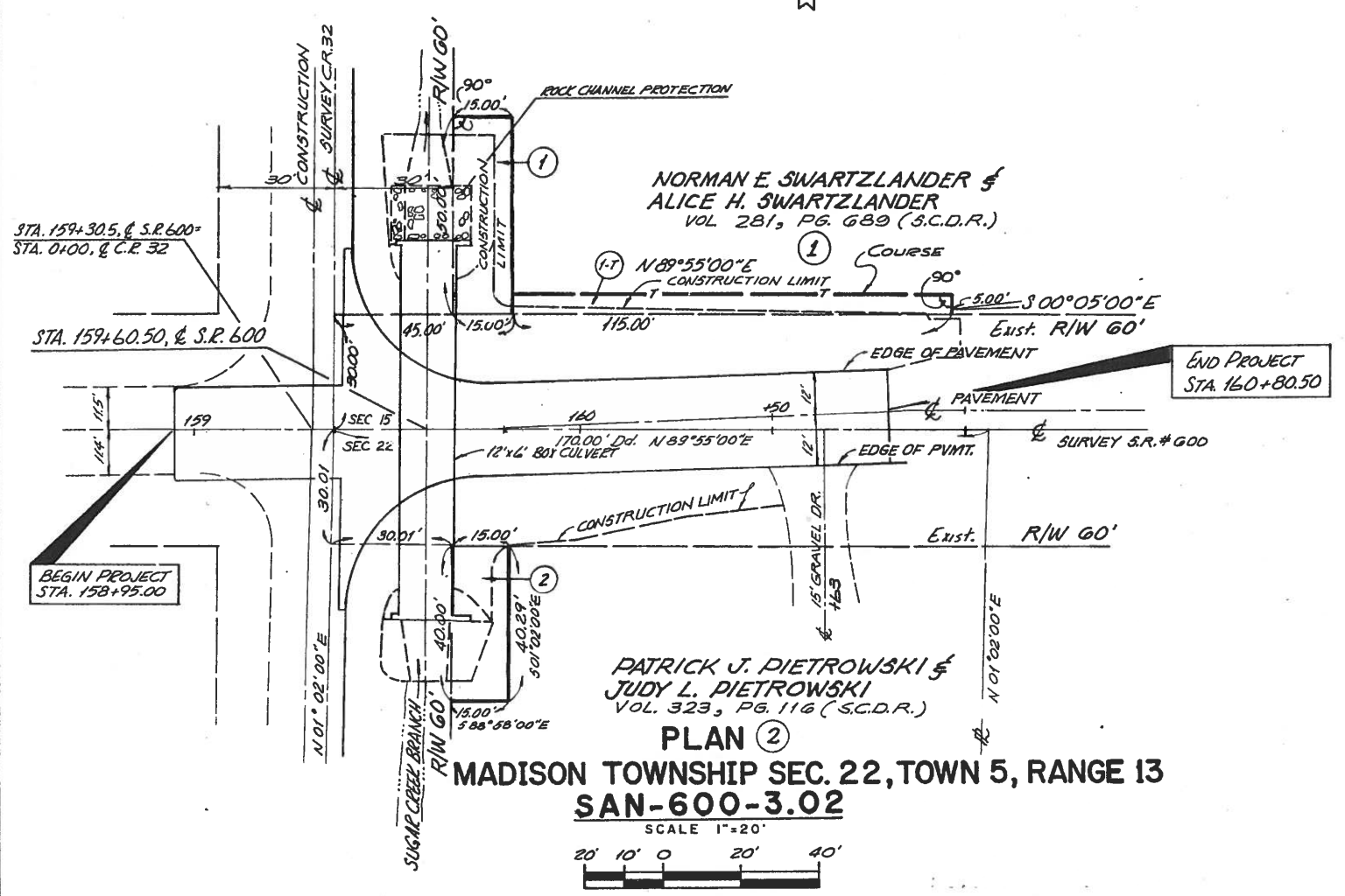
LOCATION PLAN SAN-600-3.02 SCALE IN FEET
