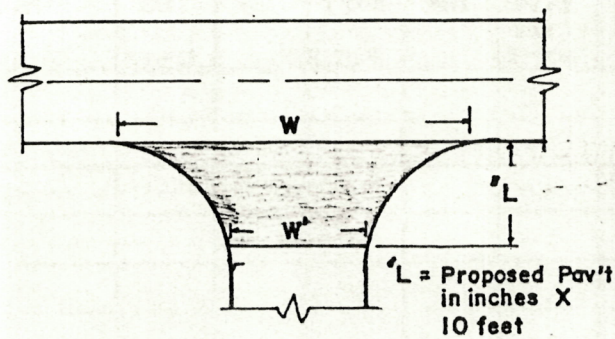
INTERSECTION TYPICAL
