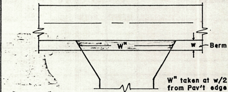
DRIVEWAY TYPICAL
