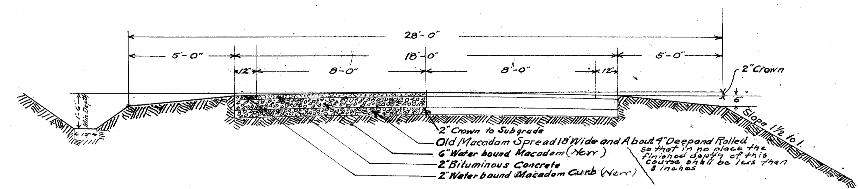
Bituminous Concrete with Macadam Base. Type A
