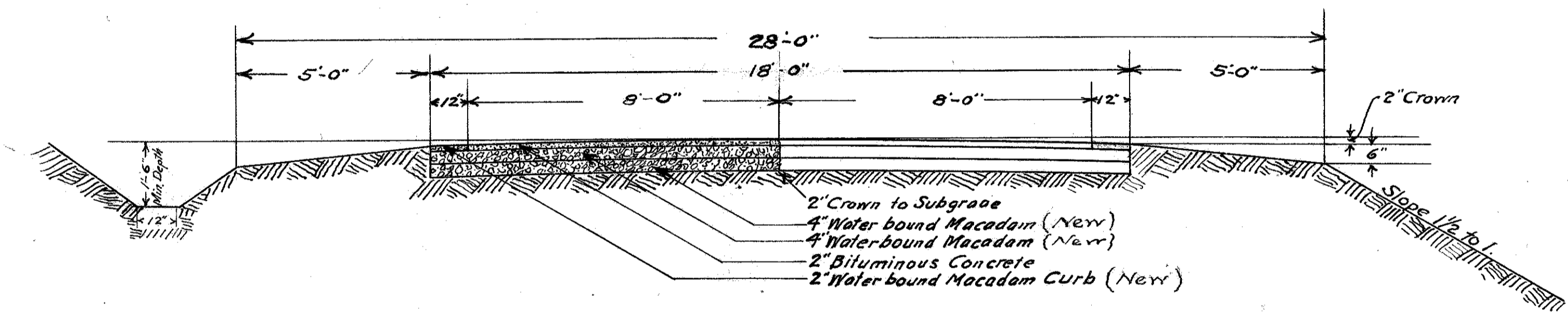
Bituminous Concrete with Macadam Base. Type B
