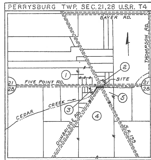
LOCATION PLAN SCALE IN FEET
