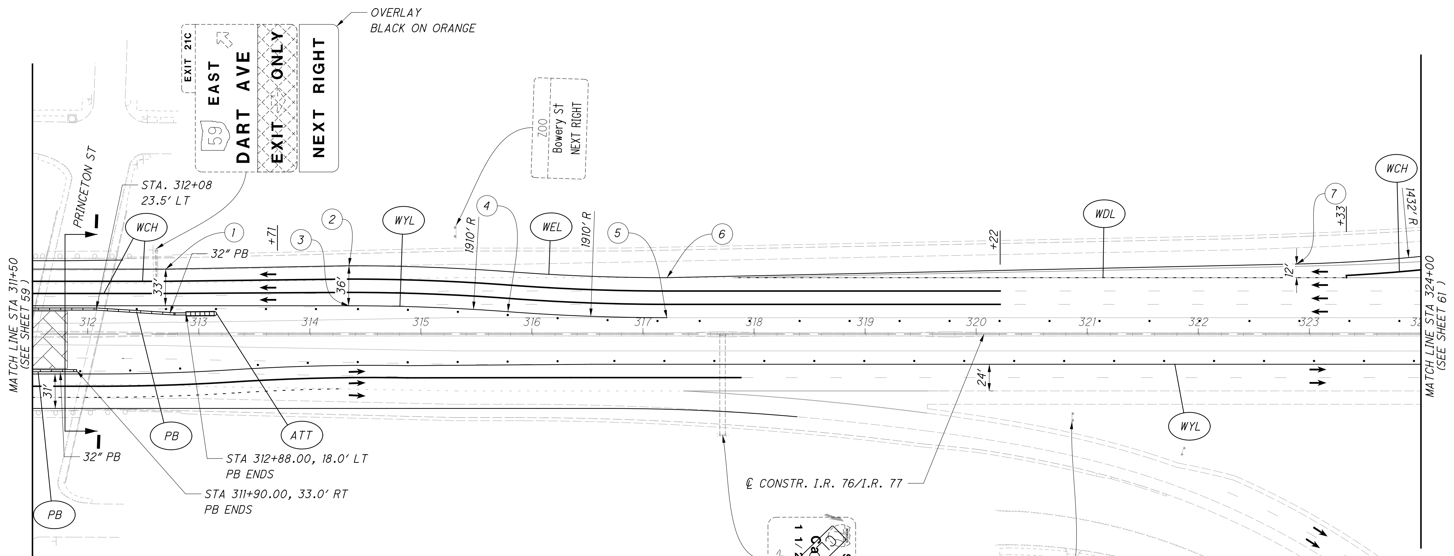
PHASE 4A SECTION I-I IR 76/77 UNDER PRINCETON ST
