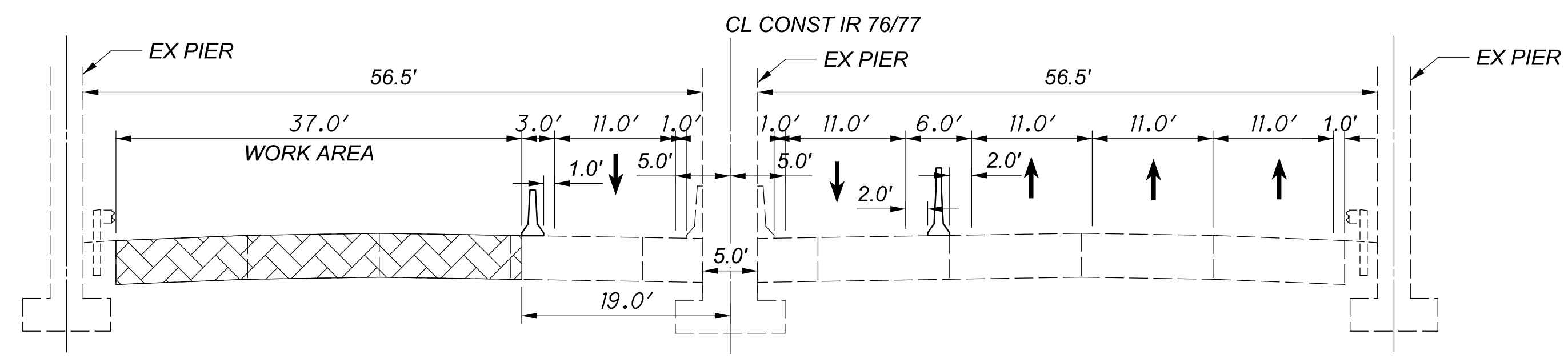
PHASE 3A STEPS 1 AND 2 SECTION H-H IR 76/77 UNDER SR 59
