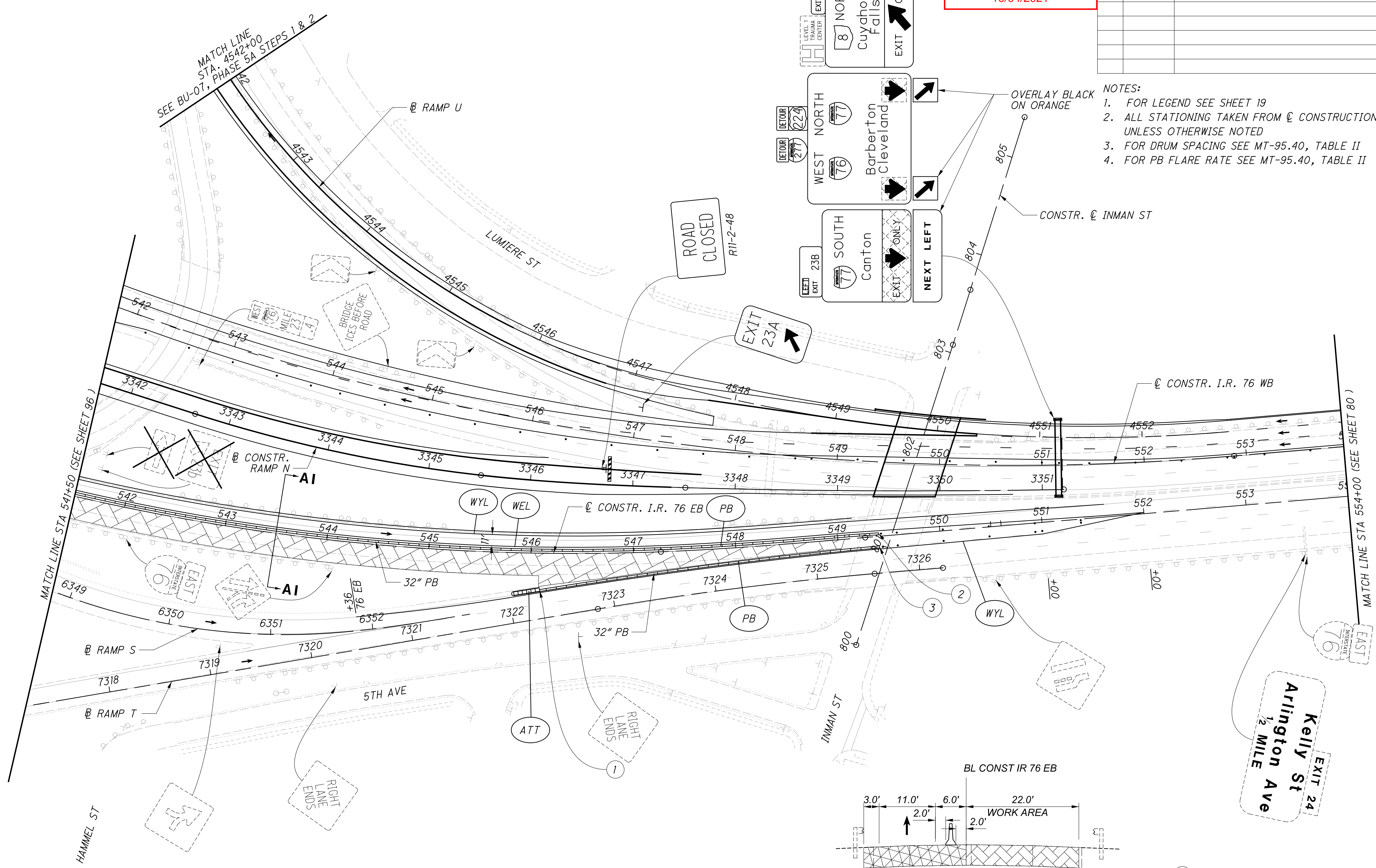
PHASE 5A STEP 2 SECTION AI-AI STA. 543+50
