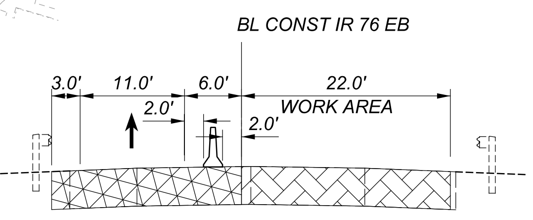
PHASE 5A STEP 2 SECTION AI-AI STA. 543+50
