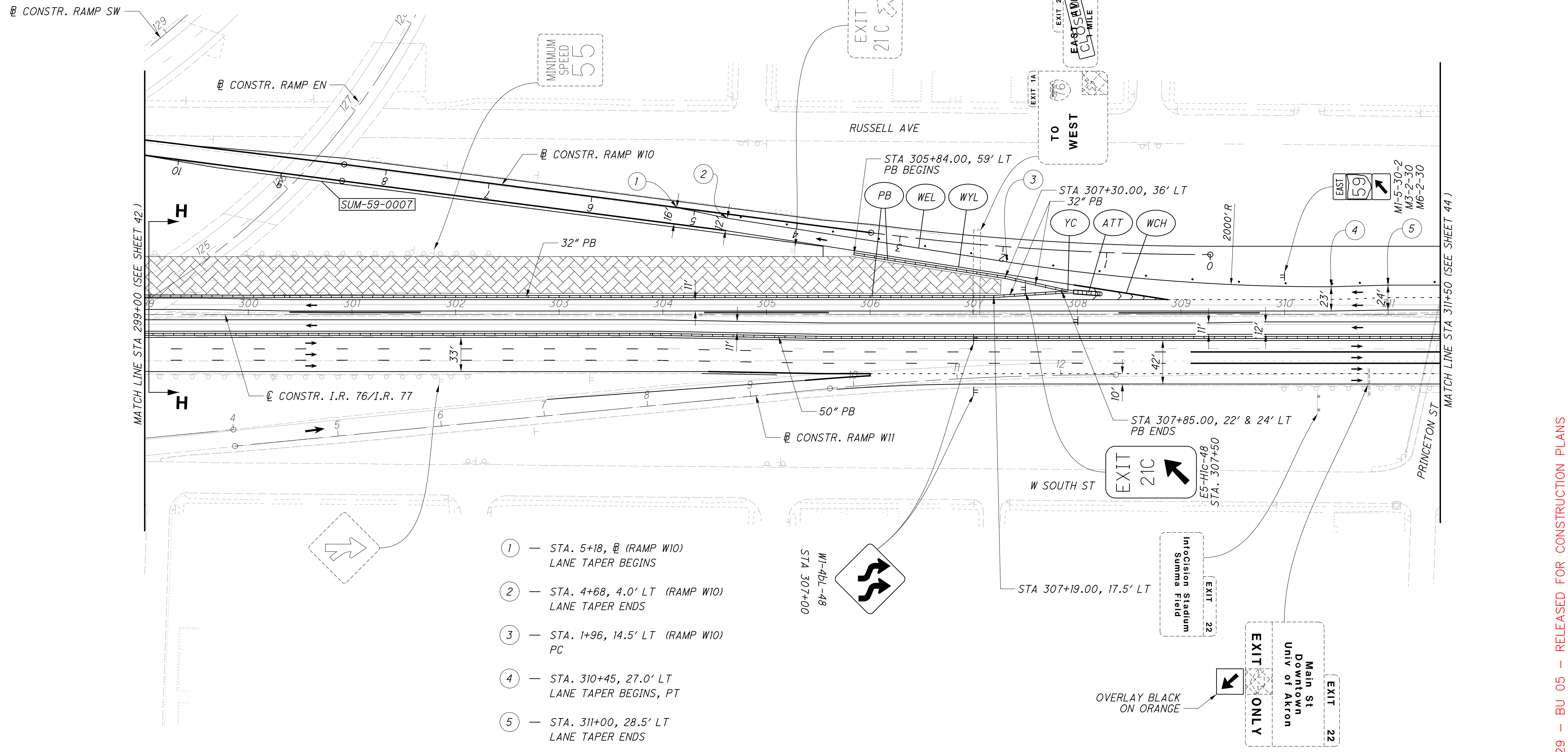
PHASE 3A STEPS 1 AND 2 SECTION H-H IR 76/77 UNDER SR 59
