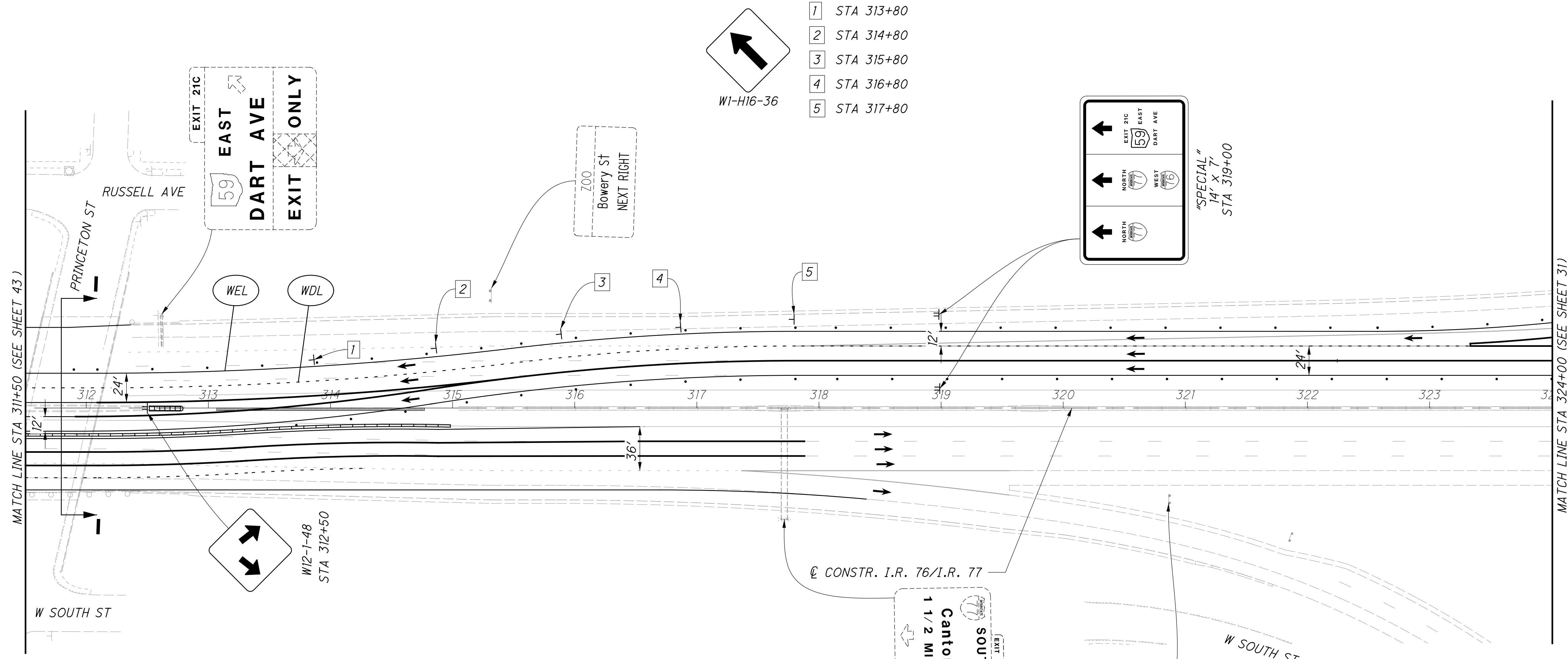
PHASE 3A STEP 2 IR 76/77 UNDER PRINCETON ST
