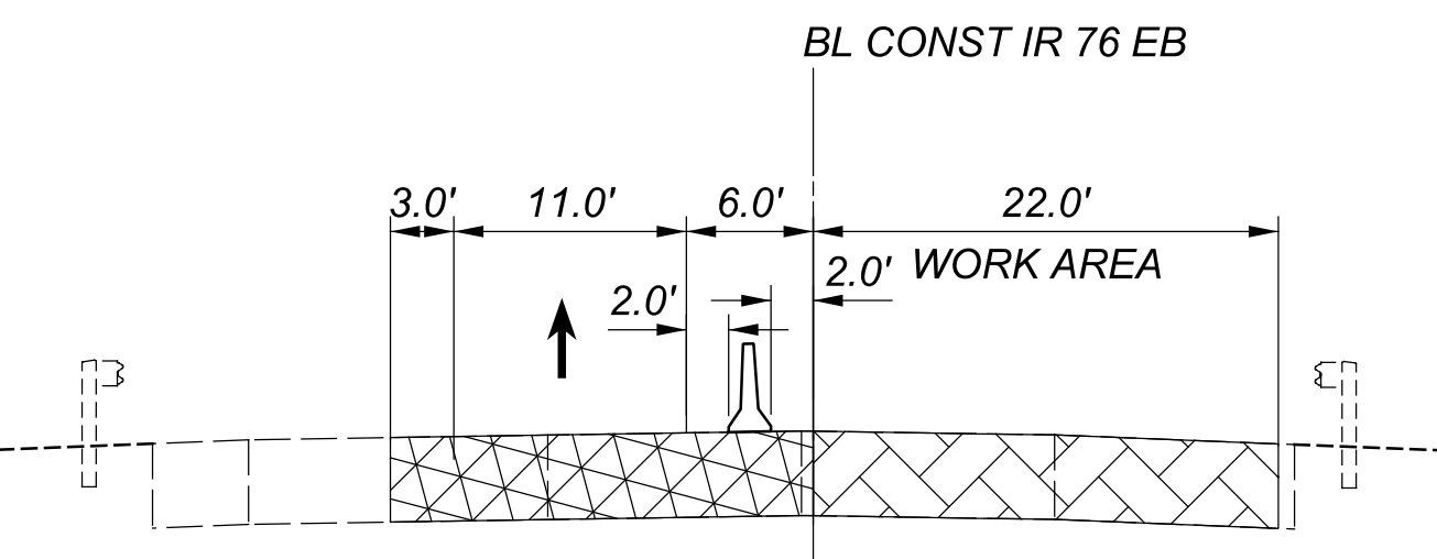
PHASE 5A STEP 2 SECTION AF-AF STA. 535+00
