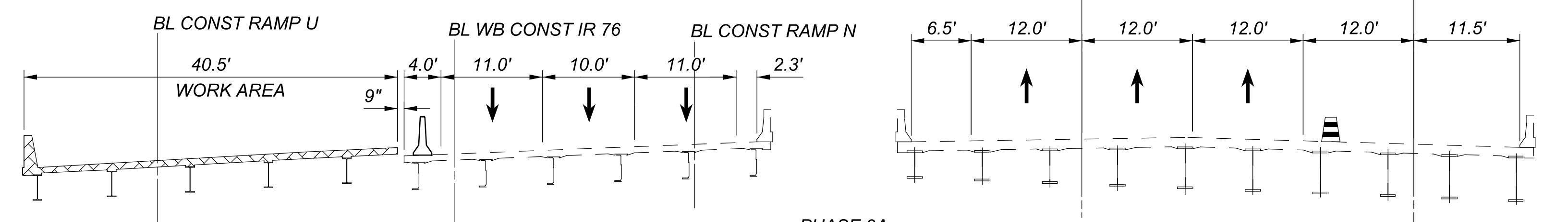
PHASE 3A SECTION P-P IR 76 WB OVER INMAN STREET
