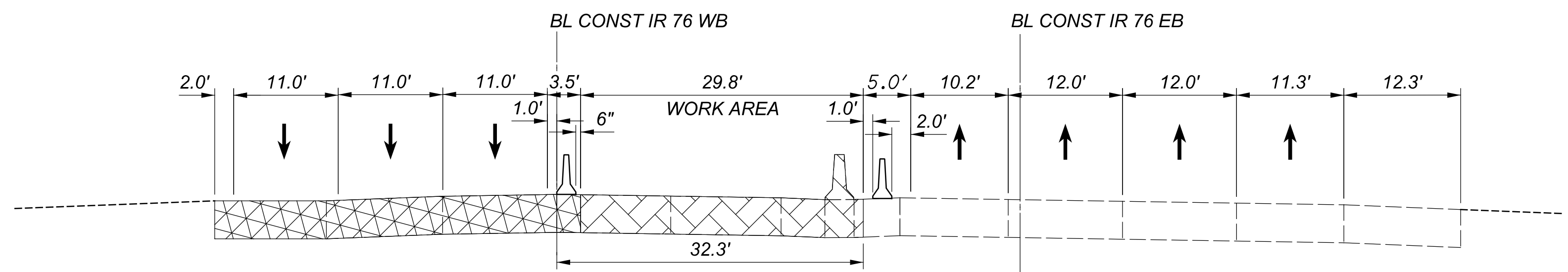
PHASE 4A SECTION AH-AH STA. 557+00
