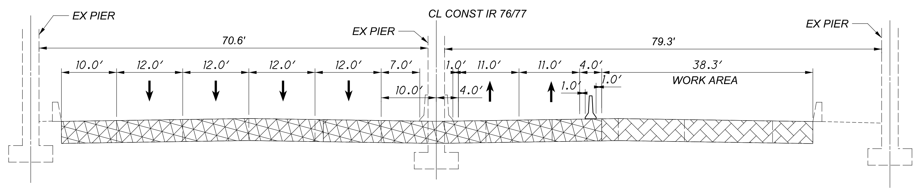
PHASE 5A SECTION G-G IR 76/77 UNDER HILLCREST PEDESTRIAN BRIDGE
