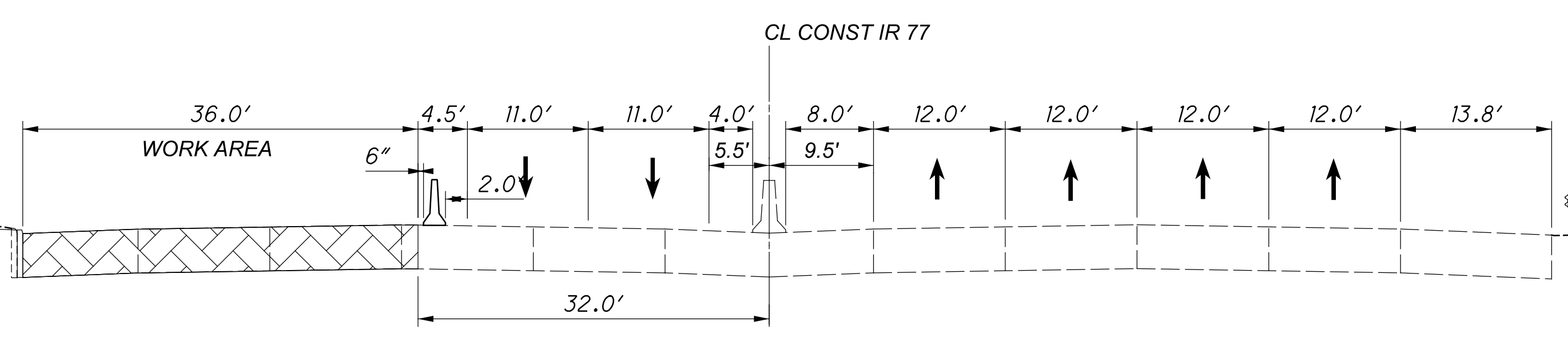
PHASE 3A SECTION X-X IR 76 STA 513+00
