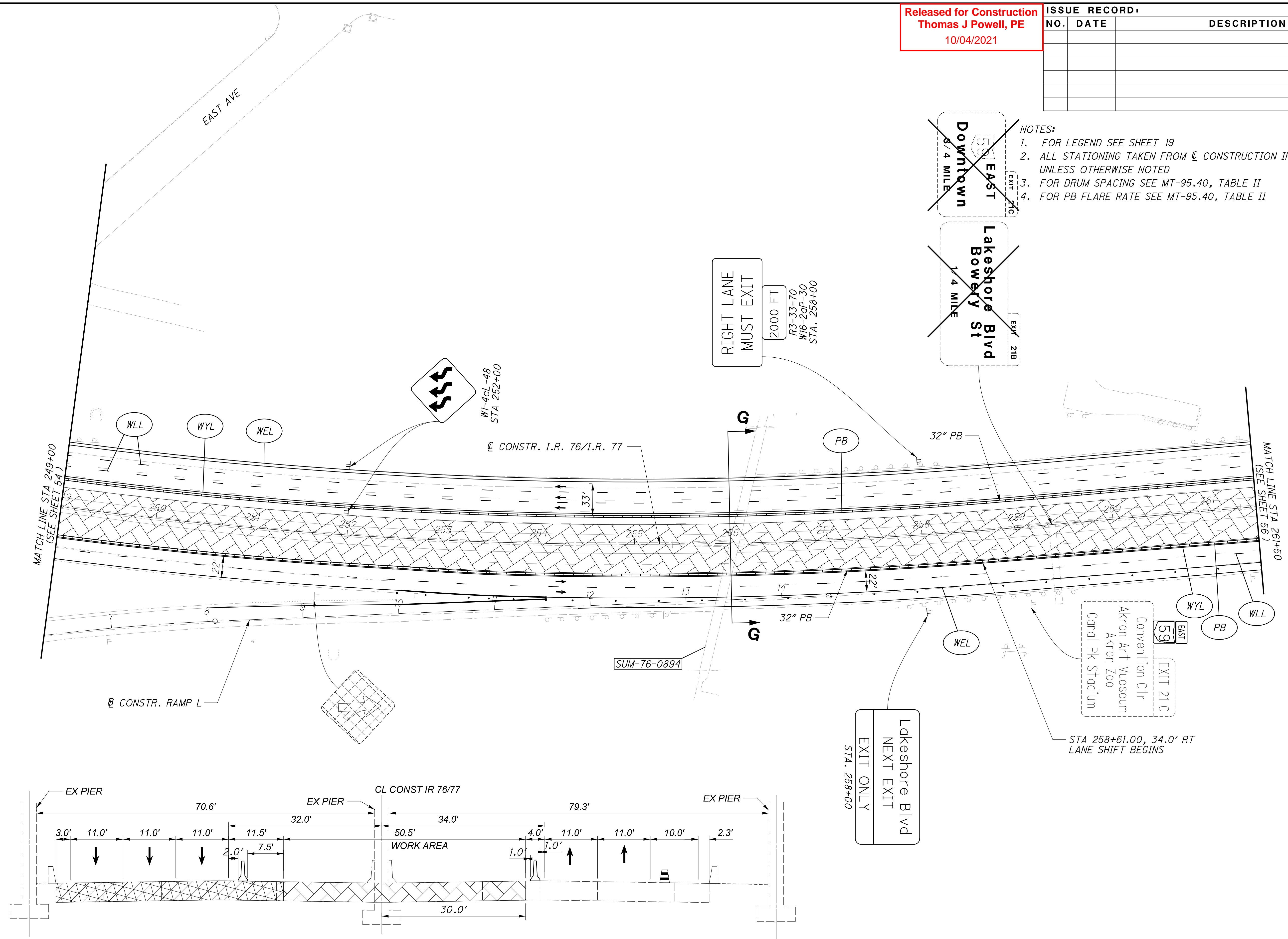
PHASE 4A SECTION G-G IR 76/77 UNDER HILLCREST PEDESTRIAN BRIDGE
