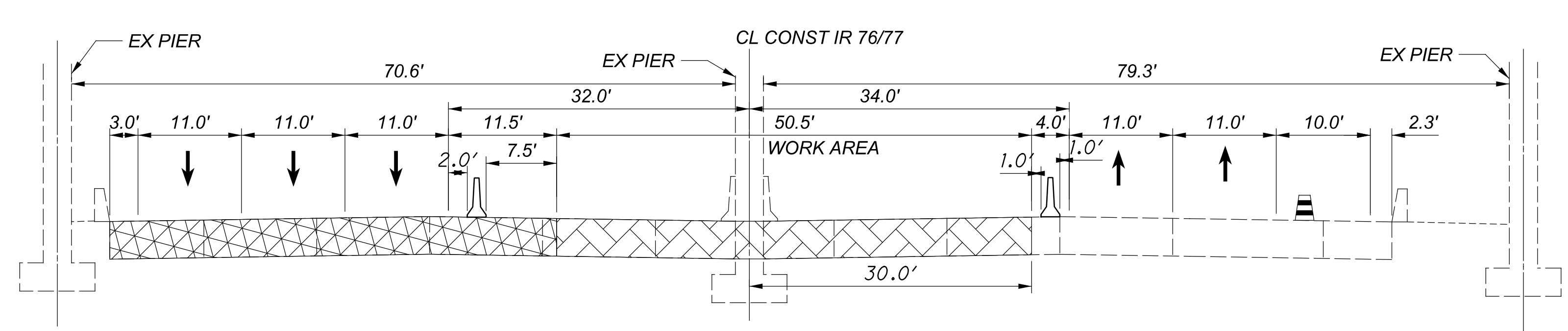
PHASE 4A SECTION G-G IR 76/77 UNDER HILLCREST PEDESTRIAN BRIDGE
