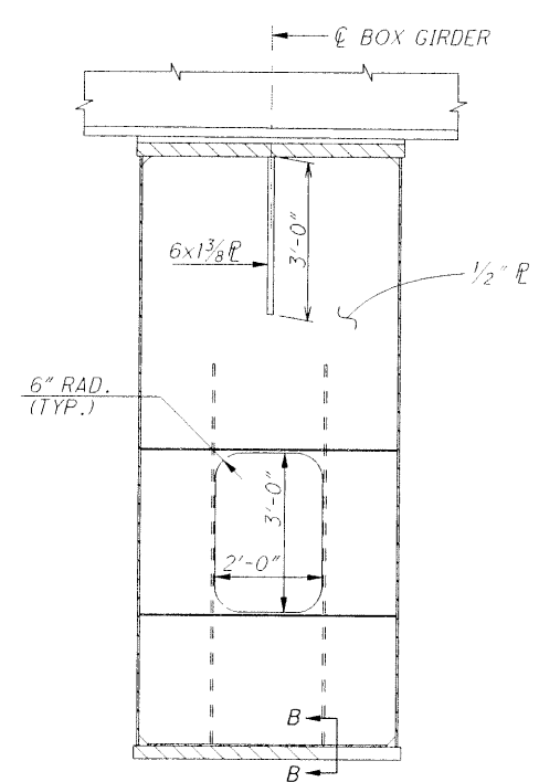
BEARING STIFFENER AT GIRDERS
