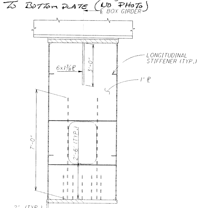
SECTION A - A BEARING STIFFENER AT COLUMNS
