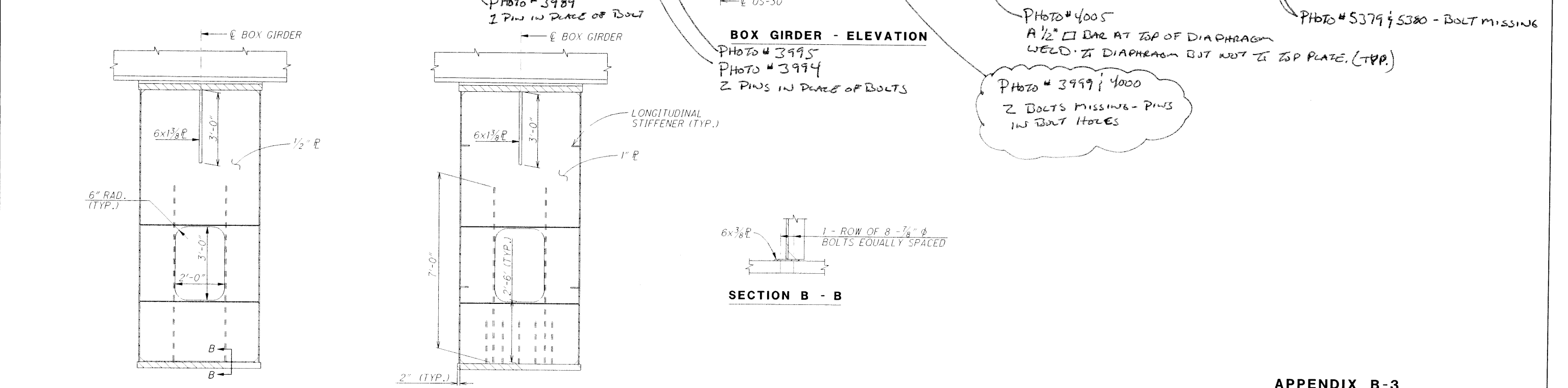
BEARING STIFFENER AT GIRDERS
