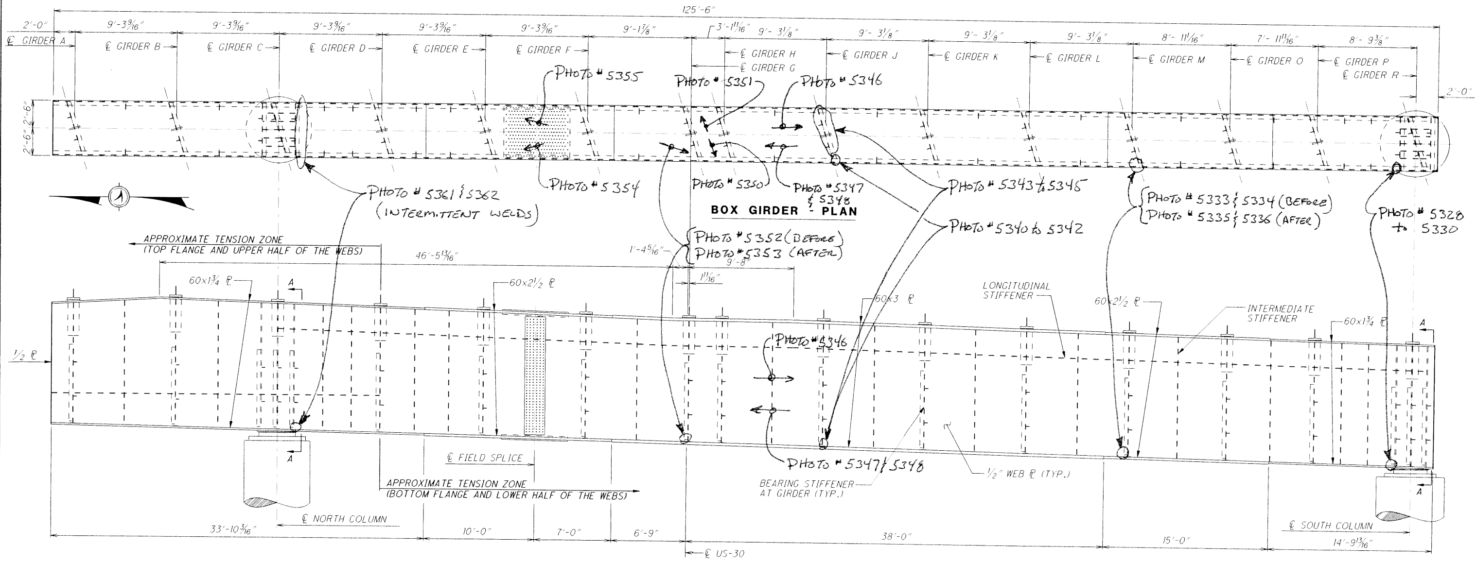
BOX GIRDER - ELEVATION
