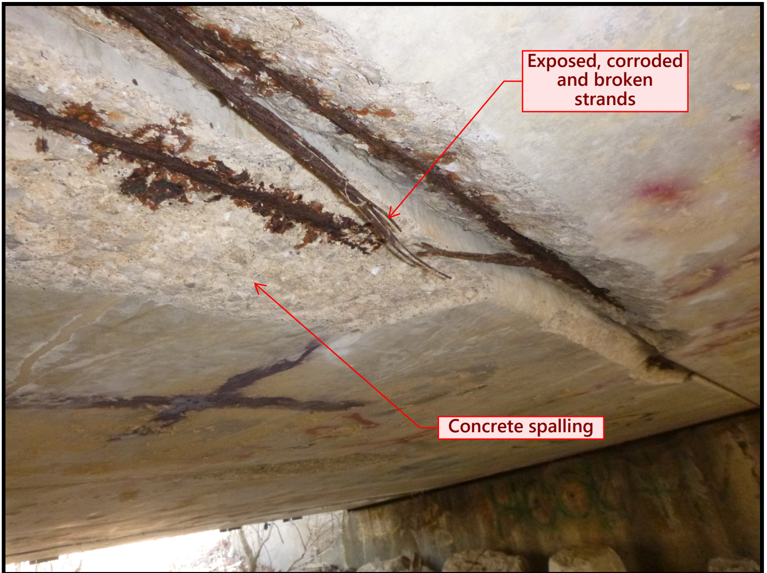
Photo 1. Current condition of prestressed box beams on Key Blvd Bridge over South Fork Licking River.
