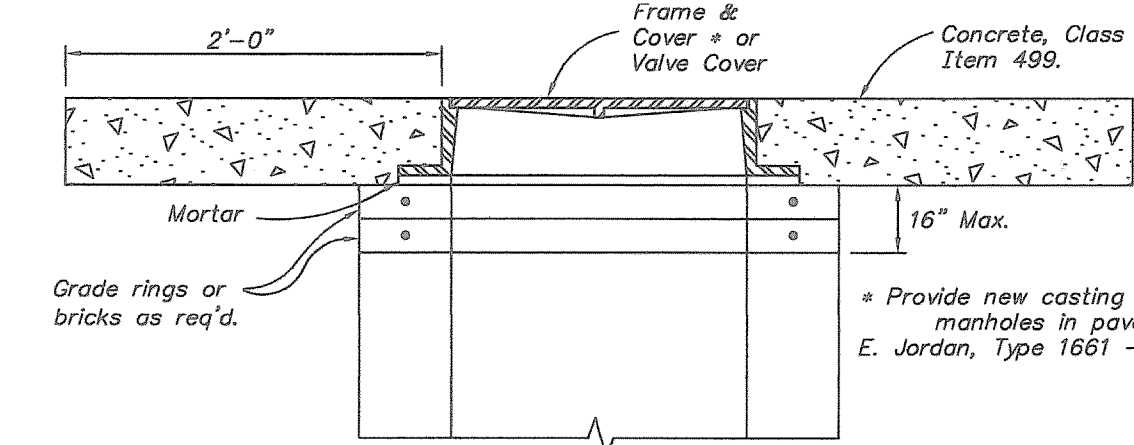
MANHOLE/VALVE COVER PAVEMENT DETAIL Not to Scale
