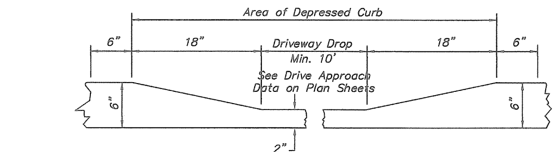
DROP CURB DETAIL (At Back of Curb) Not to Scale
