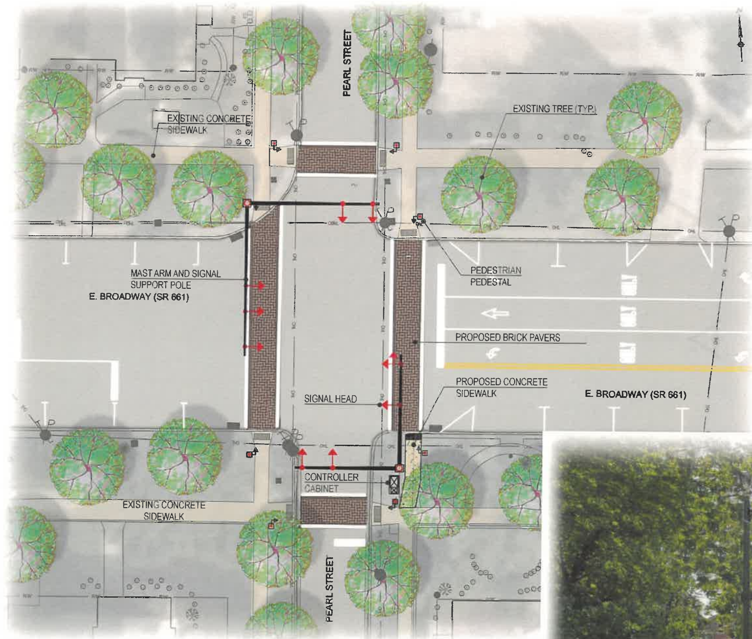
CONCEPTUAL PLAN
