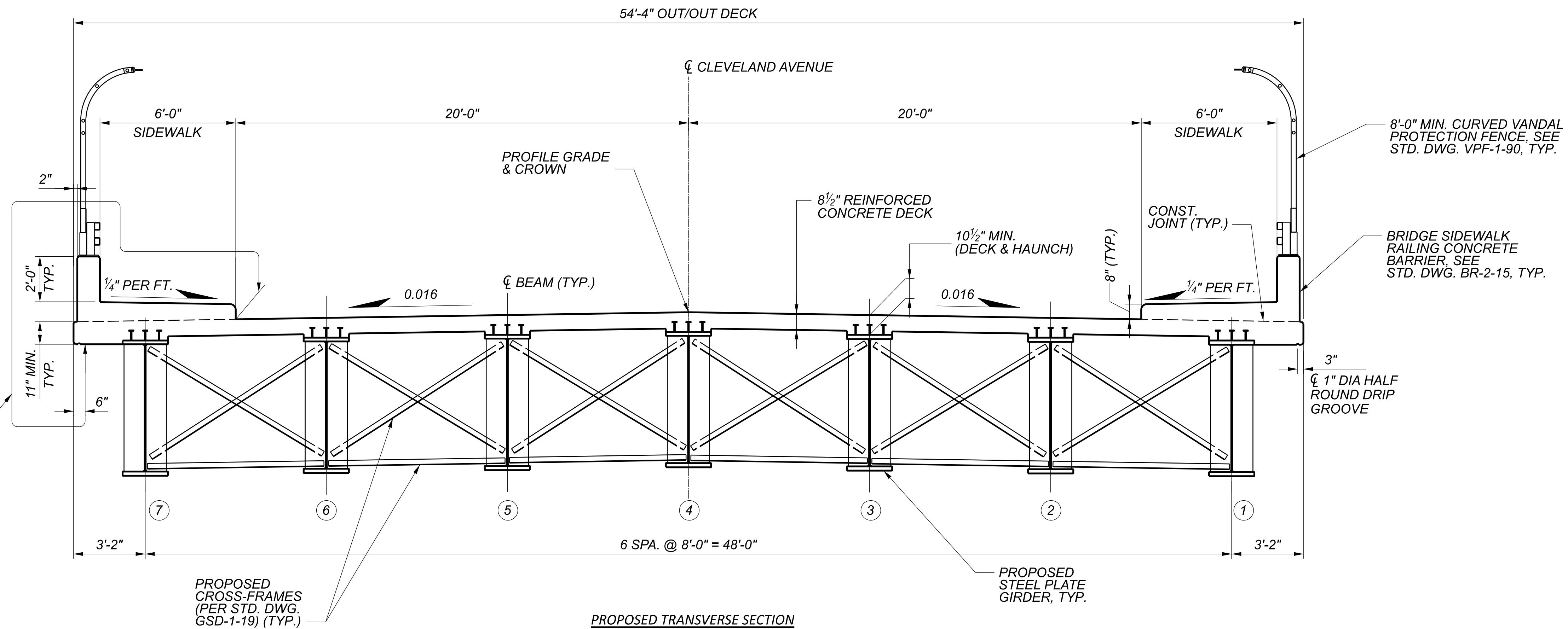
PROPOSED TRANSVERSE SECTION
