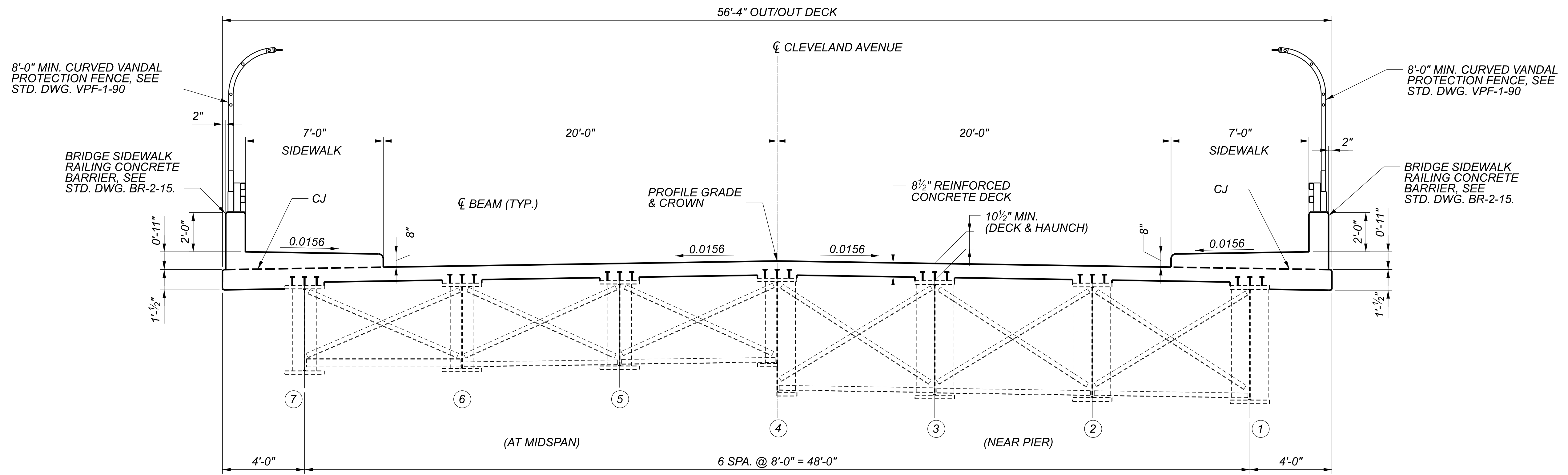
PROPOSED TRANSVERSE SECTION
