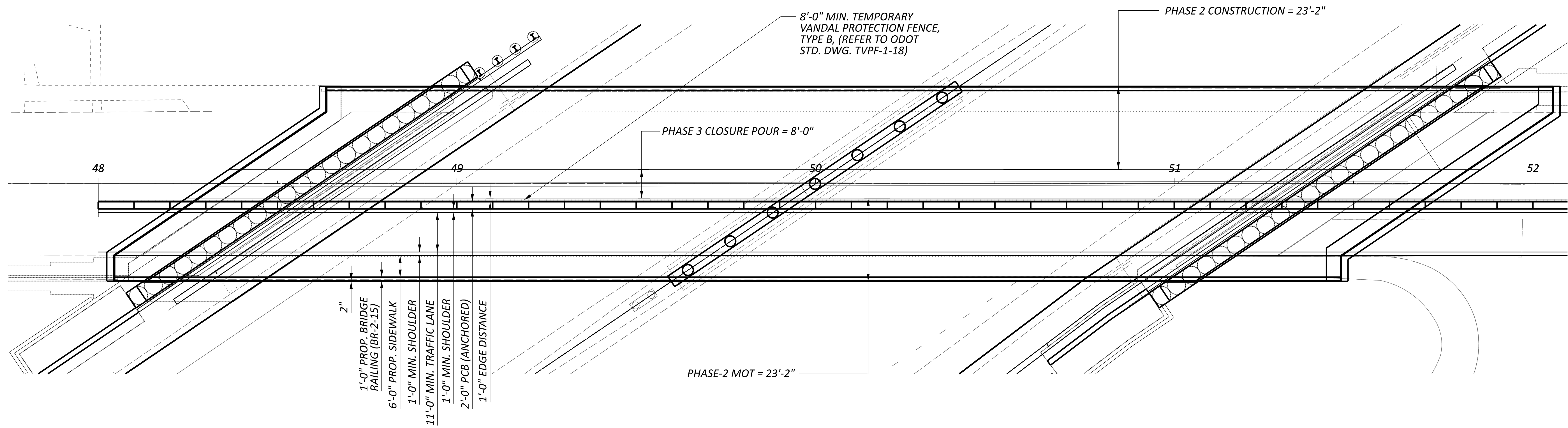
PHASE 2 (MOT & CONSTRUCTION) AND PHASE 3 (CLOSURE POUR)
