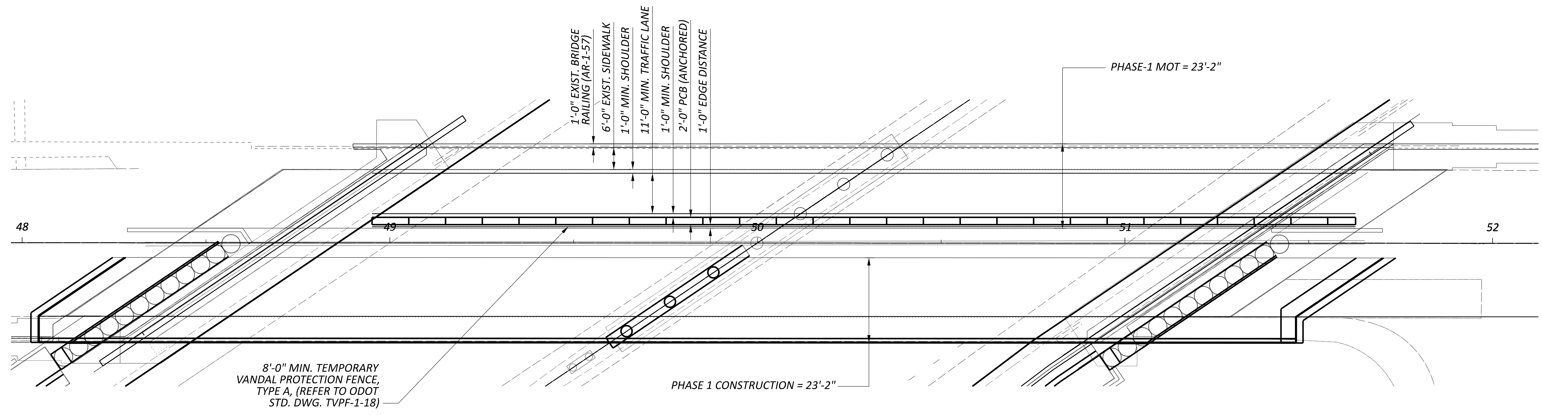
PHASE 1 (MOT & CONSTRUCTION)
