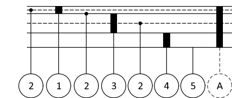
TYPICAL SECTION: PAVEMENT REPAIR, AS PER PLAN
