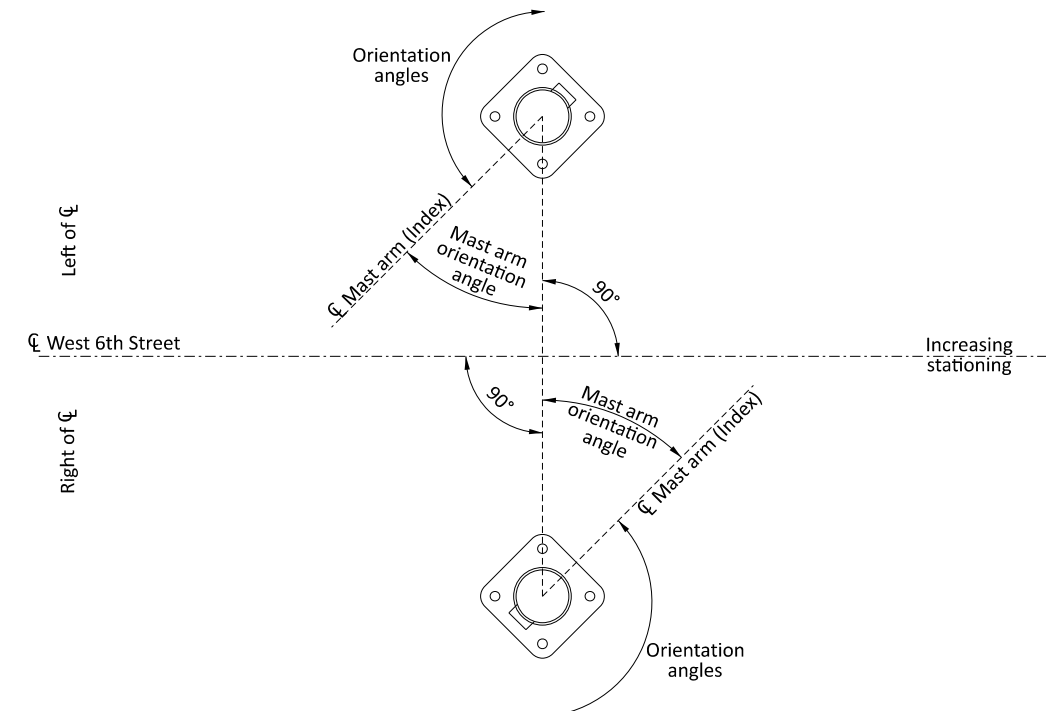
POLE ORIENTATION
