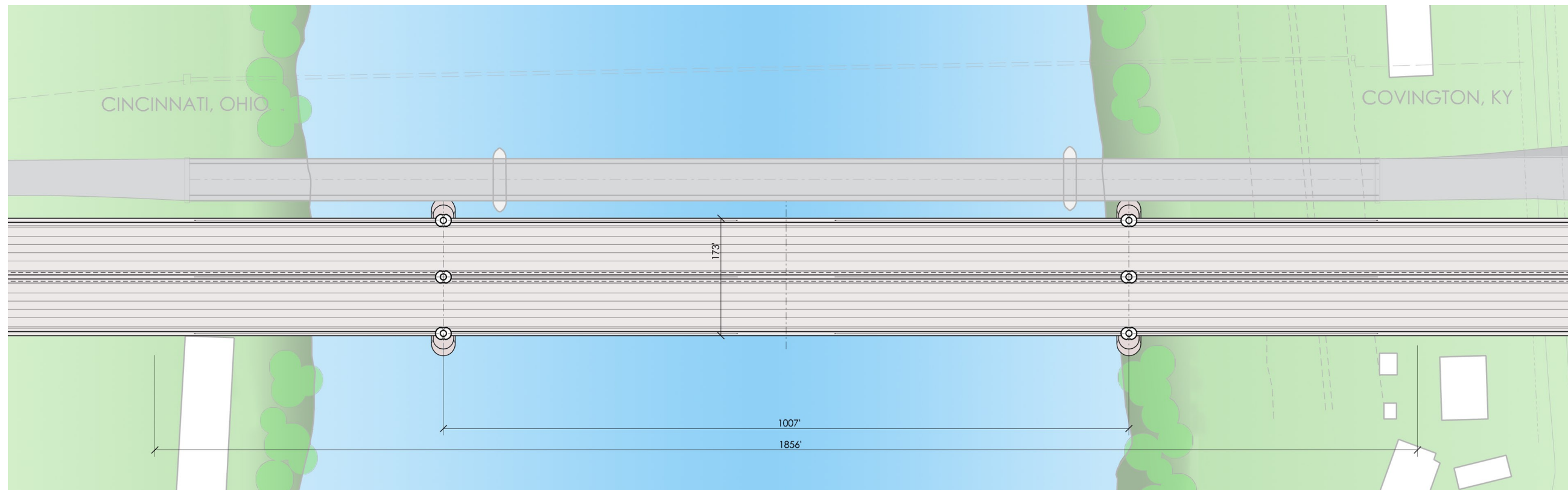
CONCEPT 7 BRENT SPENCE BRIDGE
