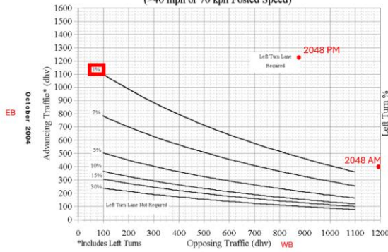
2-Lane Highway Left Turn Lane Warrant (>40 mph or 70 kph Posted Speed)
