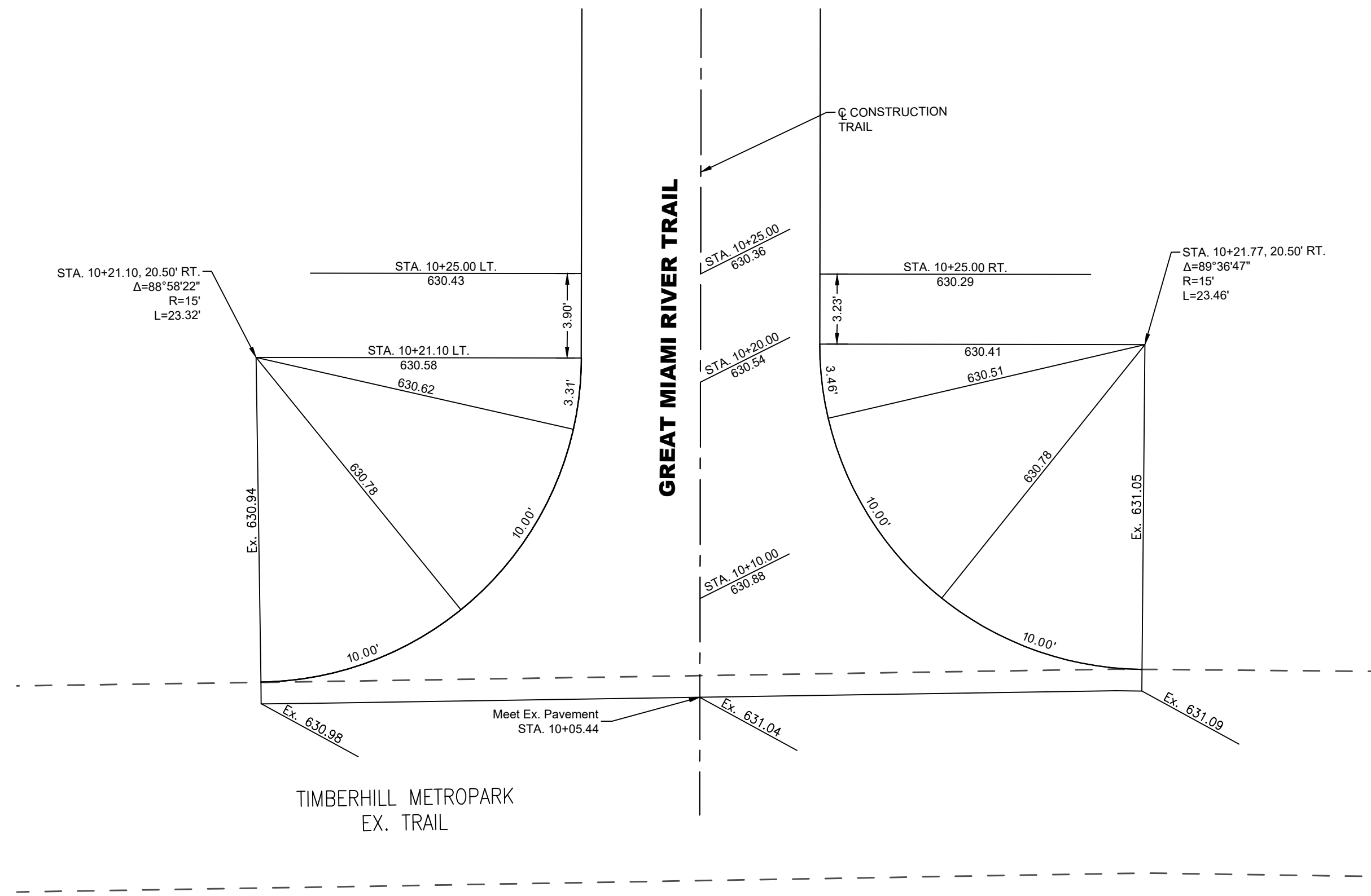
INTERSECTION DETAIL STA. 10+05.44 TO STA. 10+21.77
