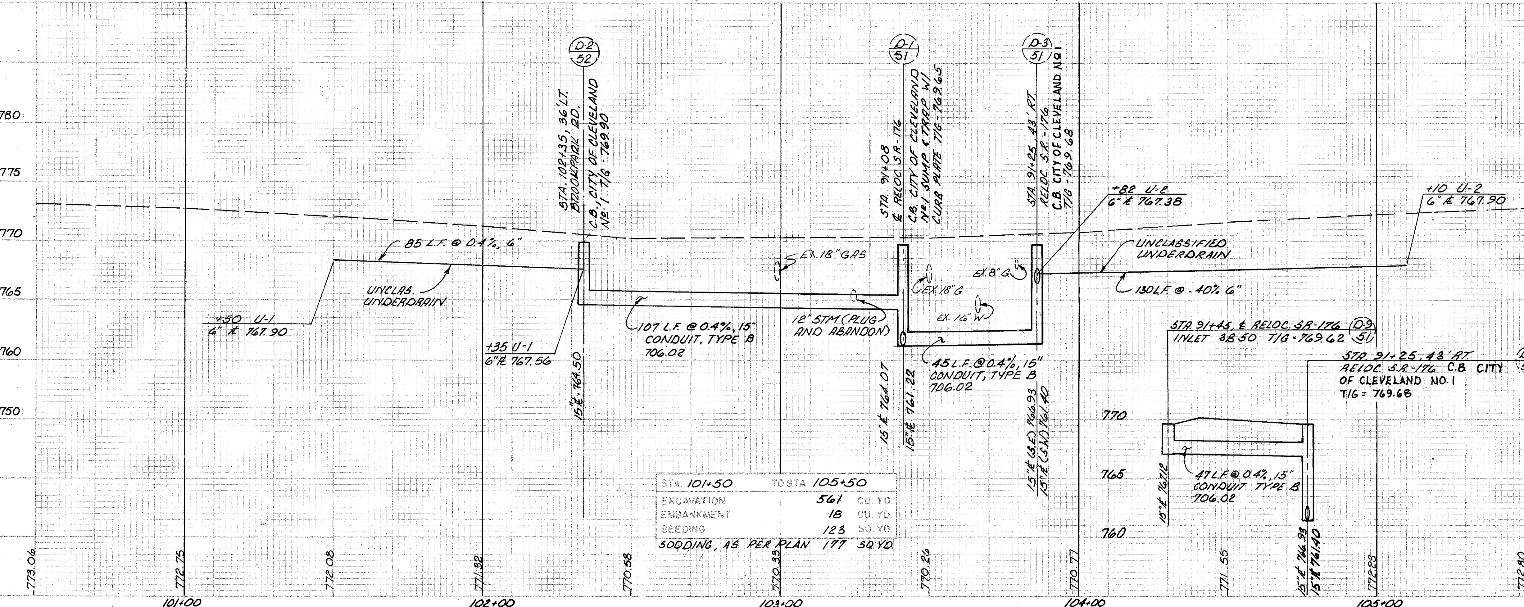
BROOKPARK ROAD PLAN & PROFILE STA. 100+50 TO STA. 105+50
