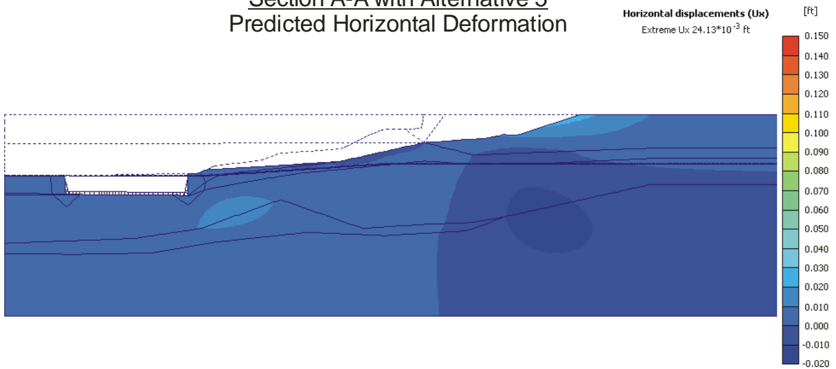
Figure 11: Predicted Deformations for Section A-A Alternative 5
