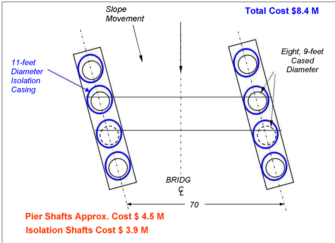
Figure 9.9: Pier foundation with casing isolation
