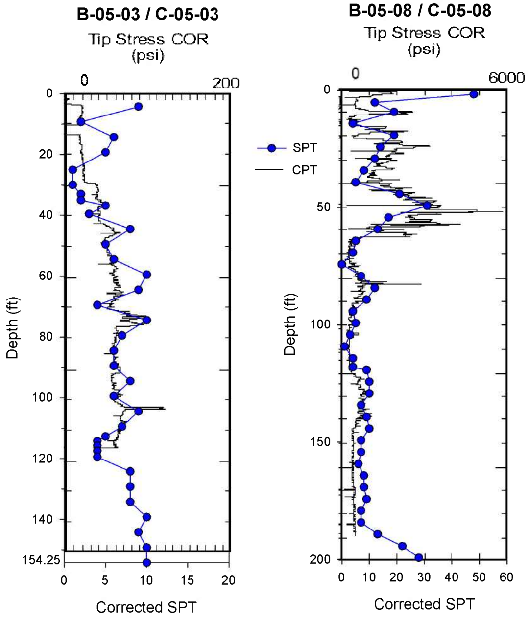
Figure 6.3: Comparison CPT vs. Corrected SPT for: a) B-05-03/C-05-03, b) B-05-08/C-05-08
