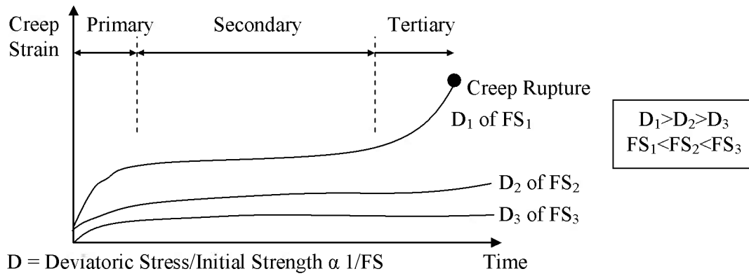
a) Typical creep strain behavior as a function of time and initial stress state.
