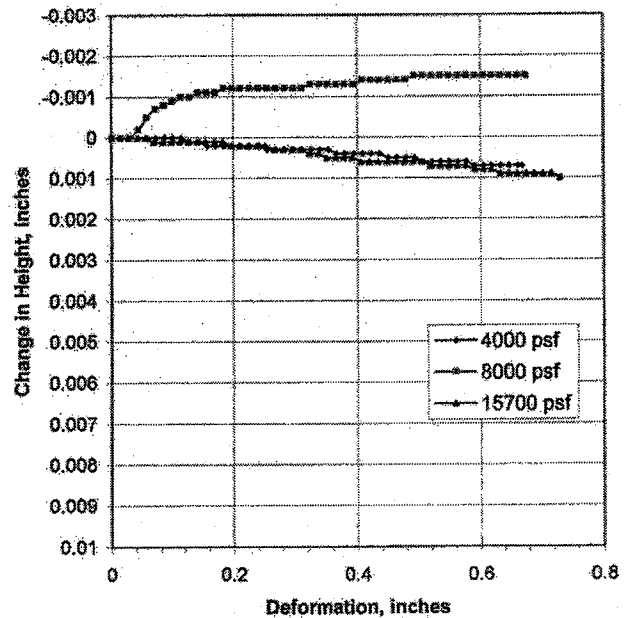
Vertical Deformation
