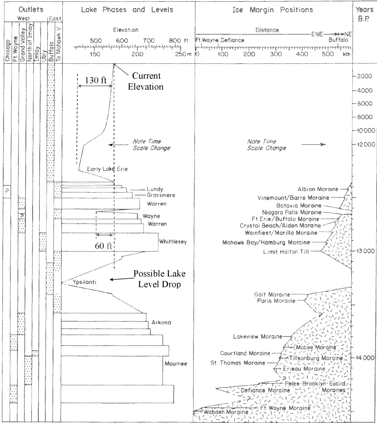
Figure 4: Lake Erie basin lake phases correlated with probable lake outlet and glacial ice boundary (after Calkin and Feenstra, 1985).
