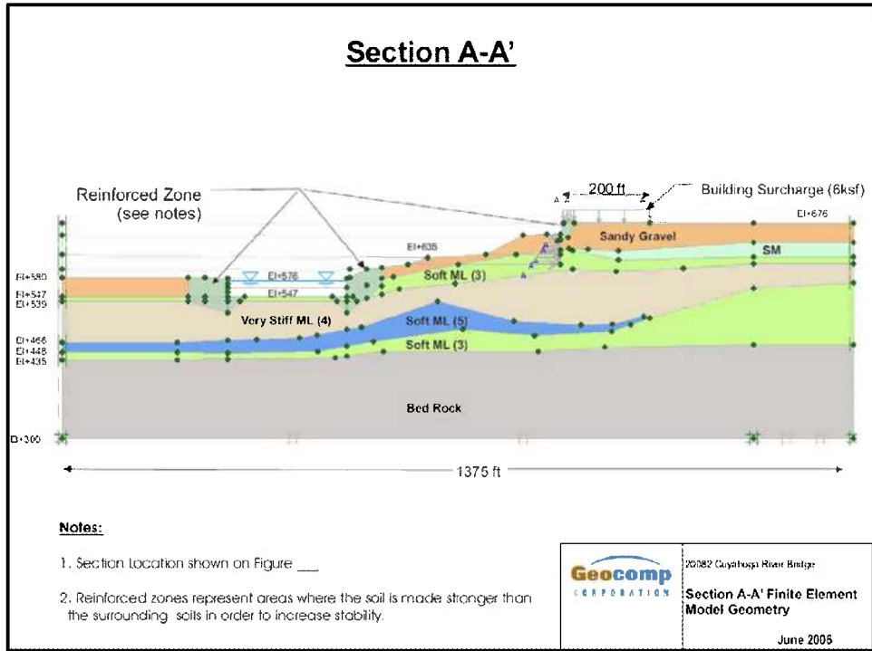
Figure 7B.1: Geometry for Section A-A
