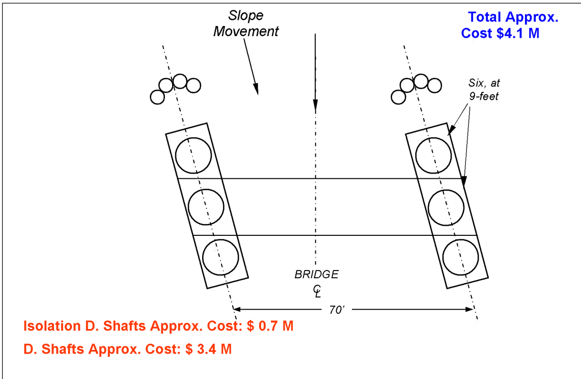
Figure 9.4: sacrificial shafts isolation system
