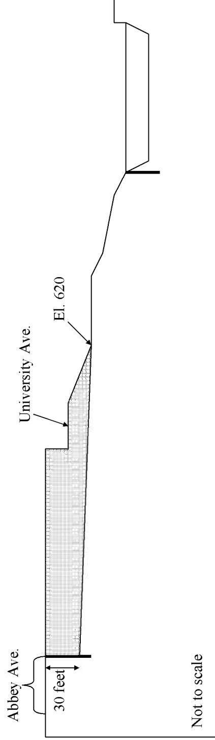
b) Alternative 8: 30-foot vertical excavation north of Abbey Avenue.
