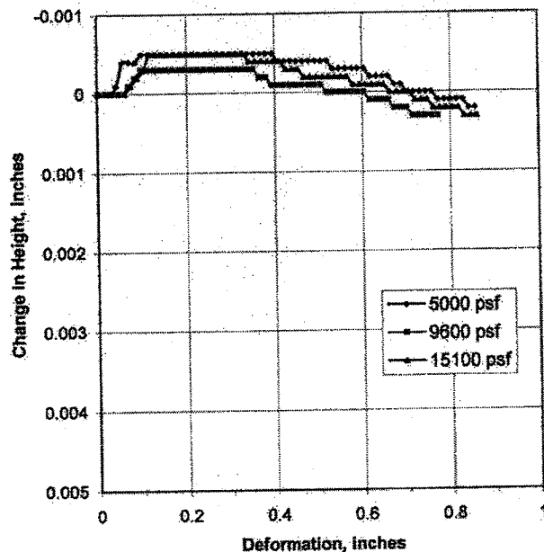
Vertical Deformation
