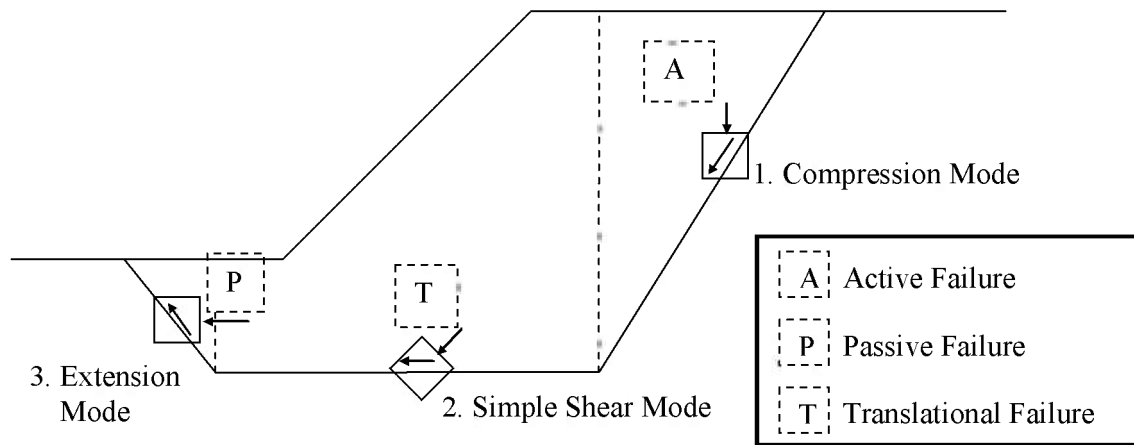
Figure 12: Modes of shear modeled in laboratory testing in relation to field failure conditions (after Terzaghi et al., 1996; Ladd and DeGroot, 2003).
