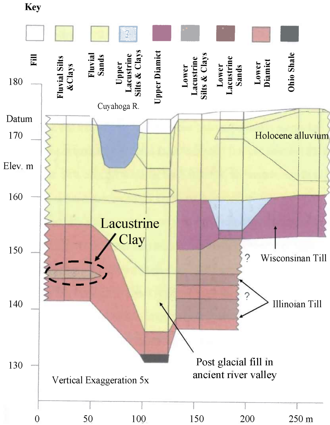
Figure 6: Cross section through the Cuyahoga River Valley near the Eagle Avenue bridge (after Bradley, 2002).
