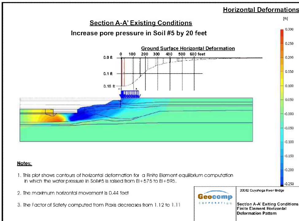
Figure 7B.3: Horizontal Movements in Existing Slope from Increasing Pore Pressure in Soil #5 by 20 ft
