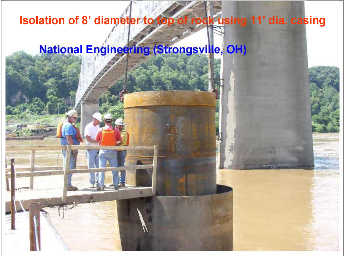
Figure 9.8: Example of an isolated drilled shaft
