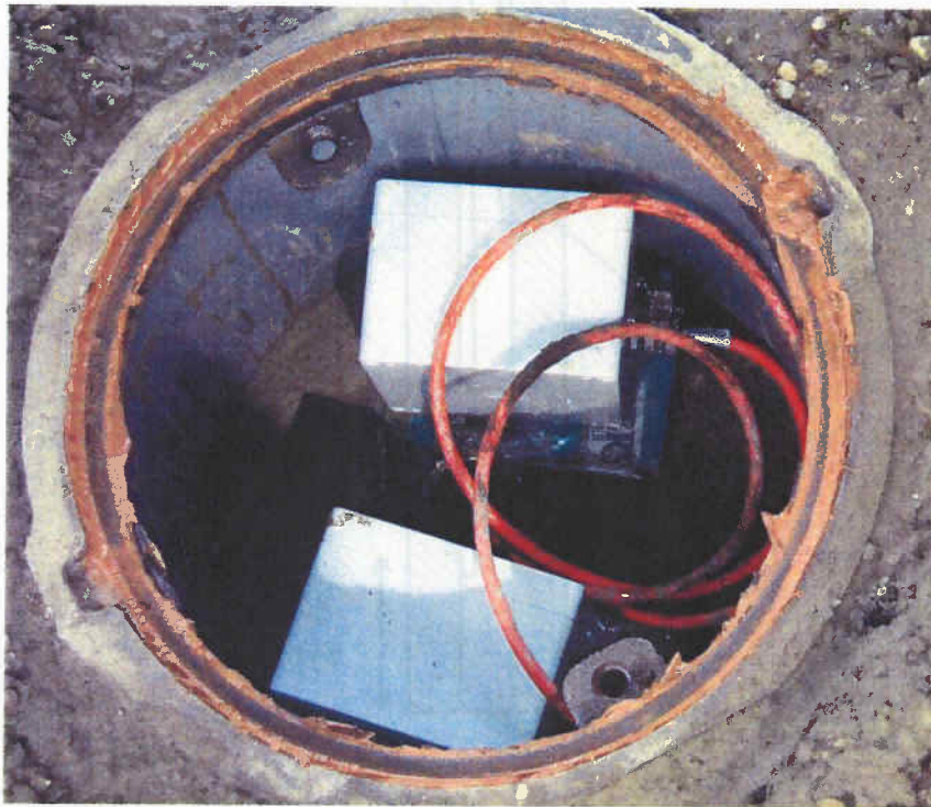
b) Typical VW-piezometer setup including a flushmount protective cover and two miniloggers.
