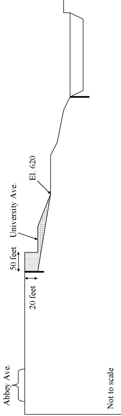
a) Alternative 1. 20-foot vertical excavation located 50 feet behind University Avenue.
