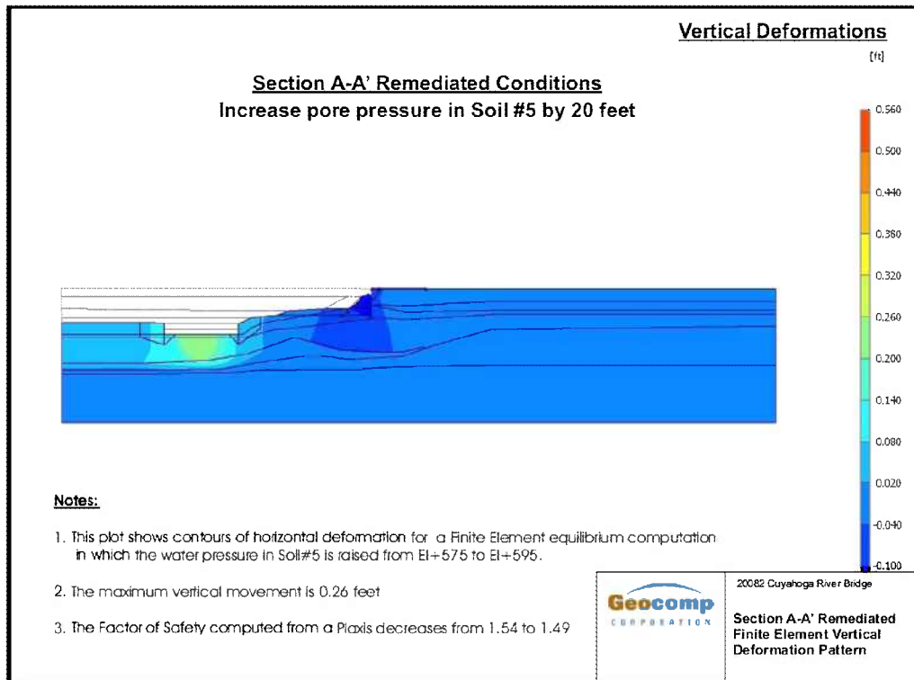
Figure 7B.8: Vertical Displacements of Unloaded Slope from an Increase in Pore Pressure in Soil #5 of 20 ft.
