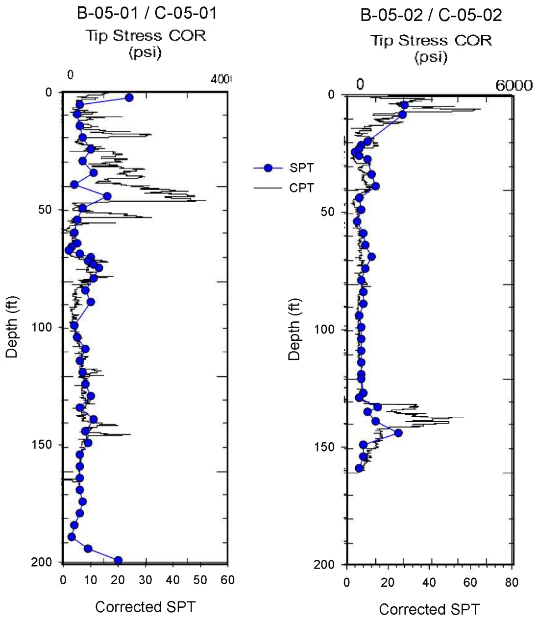
Figure 6.2: Comparison CPT vs. Corrected SPT for: a) B-05-01/C-05-01, b) B-05-02/C-05-02
