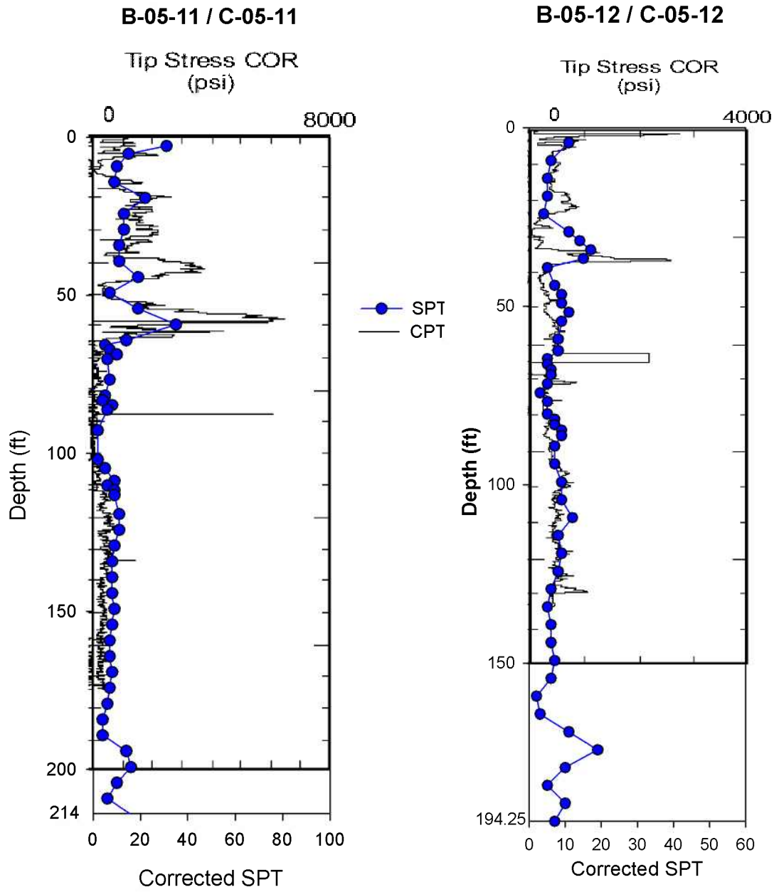
Figure 6.4: Comparison CPT vs. Corrected SPT for: a) B-05-11/C-05-11, b) B-05-12/C-05-12
