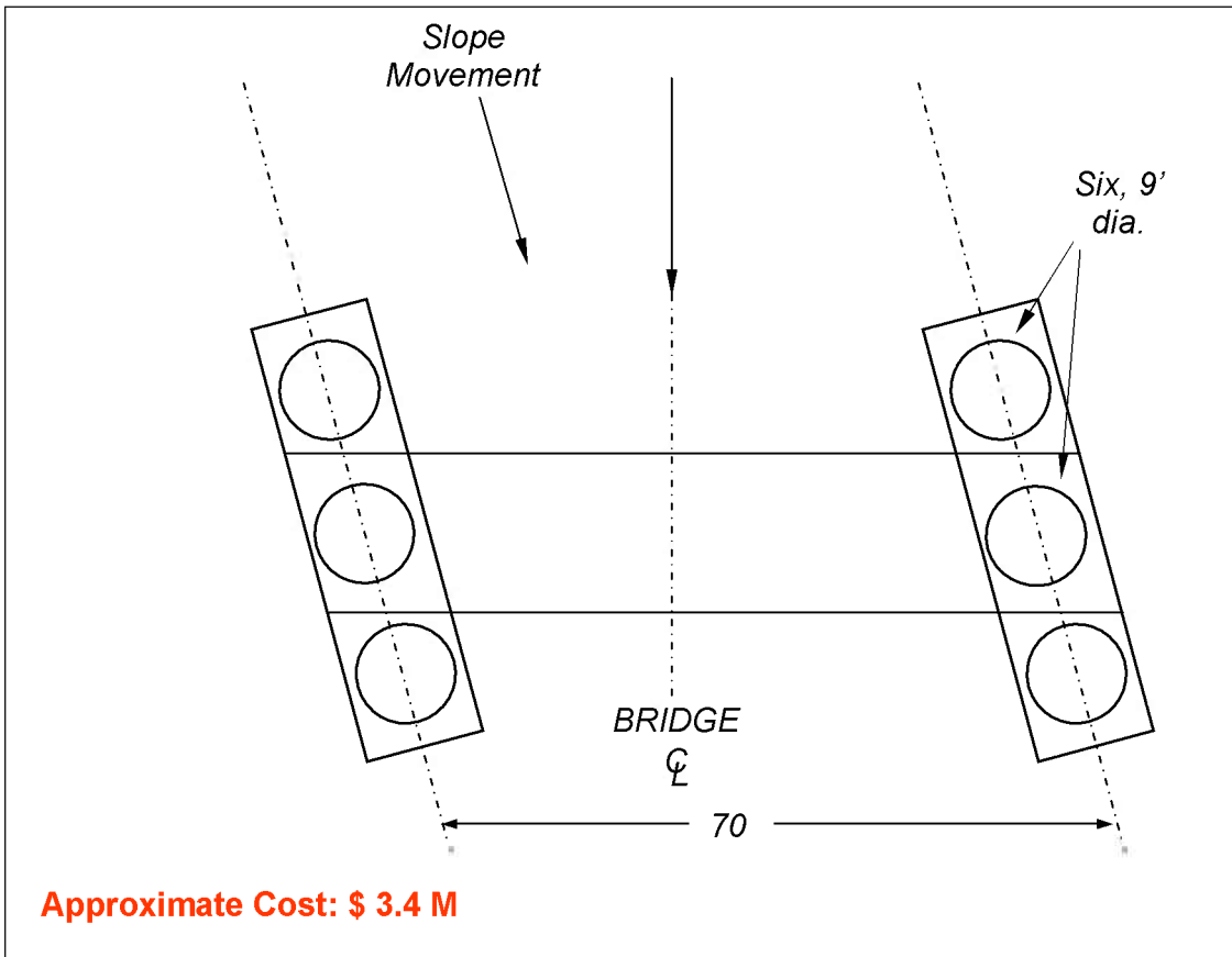
Figure 9.1: Plan view of a possible pier foundation configuration
