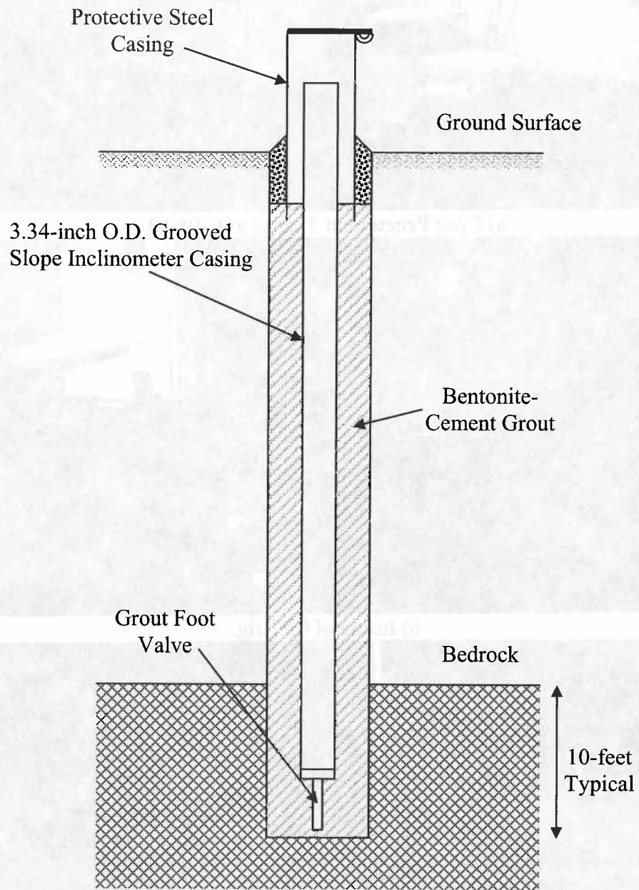
Figure 2: Typical Slope Inclinometer.
