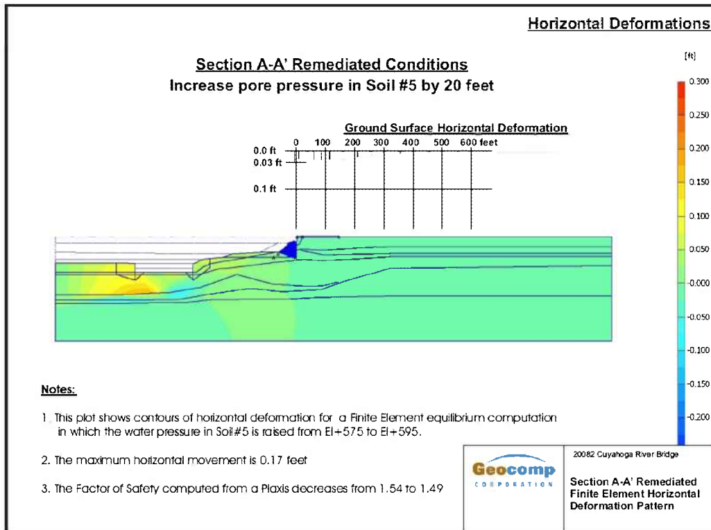
Figure 7B.7: Horizontal Displacements of Unloaded Slope from an Increase in Pore Pressure of 20 ft in Soil #5
