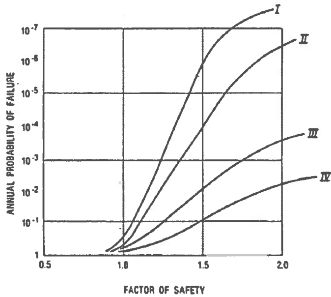
Figure 7B.10: Factor of Safety/Probability of Failure Curves (Lambe 1985)
