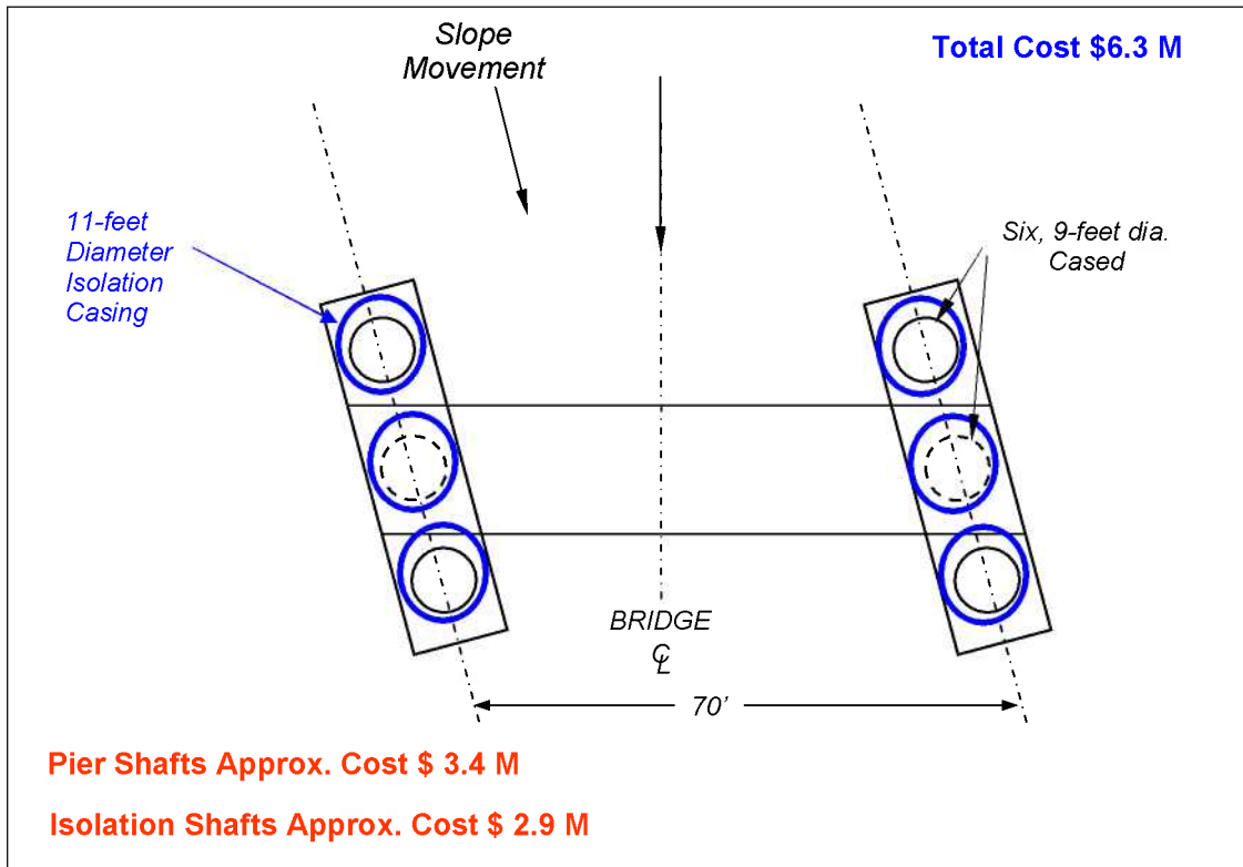
Figure 9.7. Pier foundation with casing isolation system
