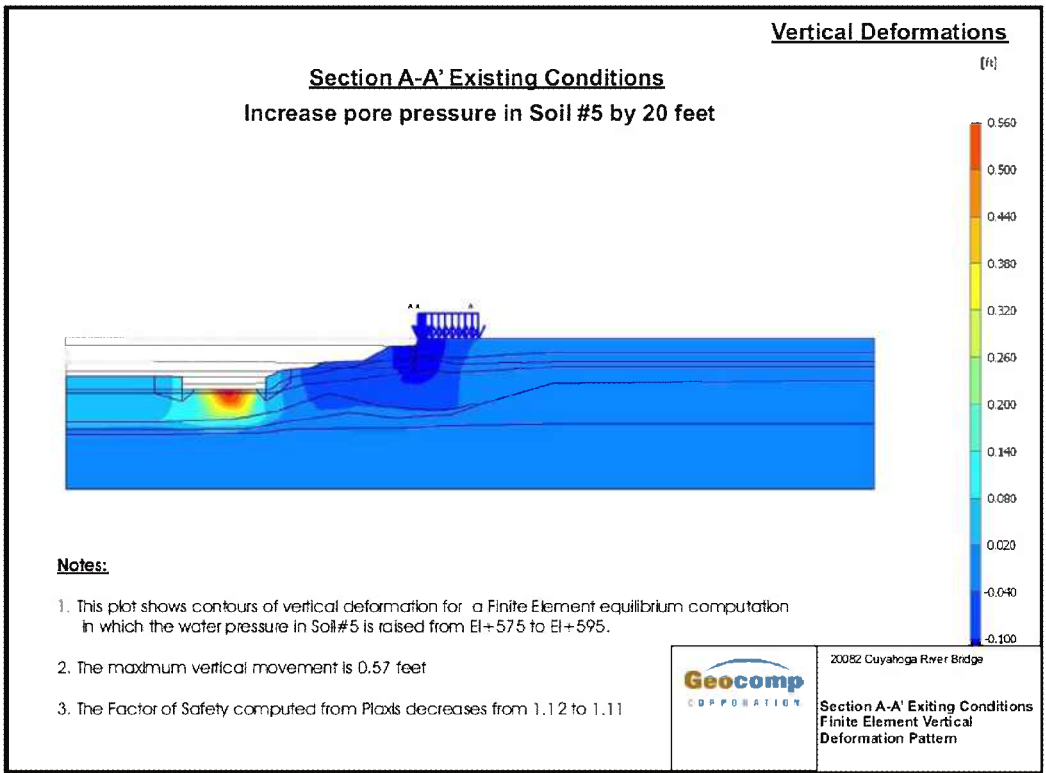
Figure 7B.4: Vertical Movement in Existing Slope from Increasing Pore Pressure in Soil #5 by 20 ft.
