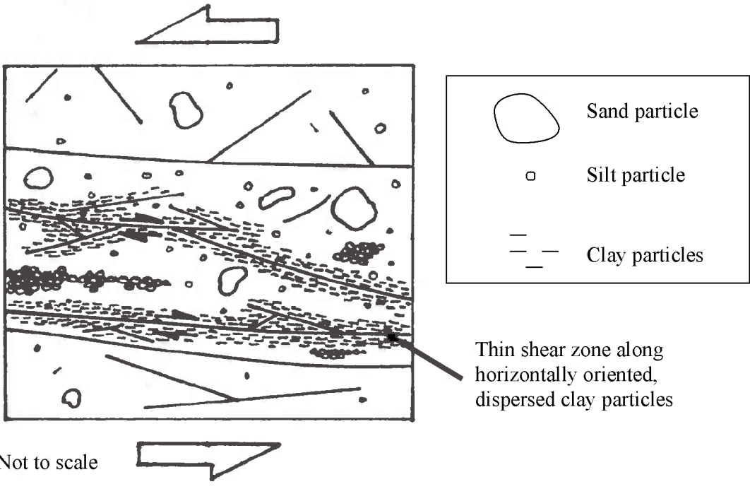
Figure 14: Possible micro-fabric of a hypothetical shear zone.
