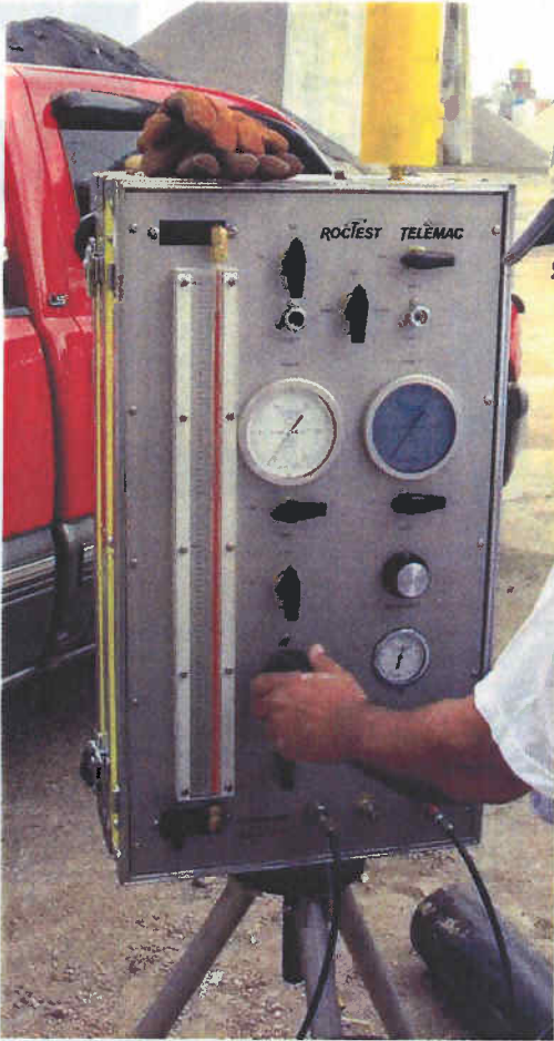
a) Pressuremeter readings device.
