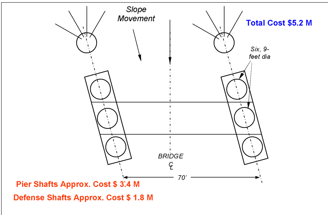
Figure 9.5: Structural fenders isolation system
