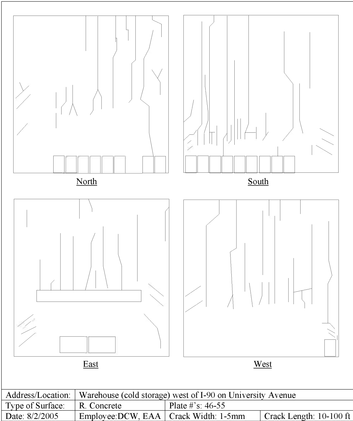
Figure 9: Crack mapping for the warehouse (cold storage) west of I-90 on University Avenue. The location and extent of the cracking is approximate only (BBCM, 2005b).
