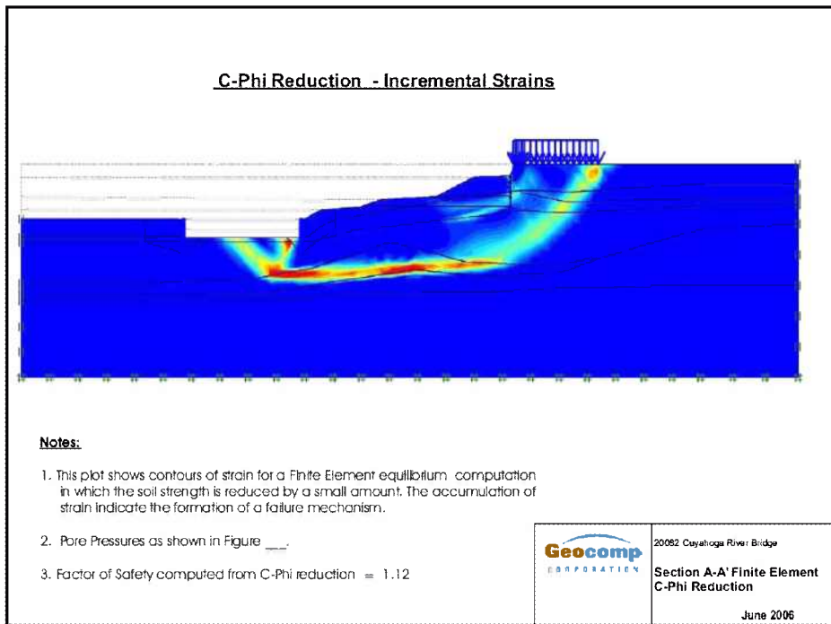
Figure 7B.2: Results of Stability Analysis of Existing Slope with PLAXIS
