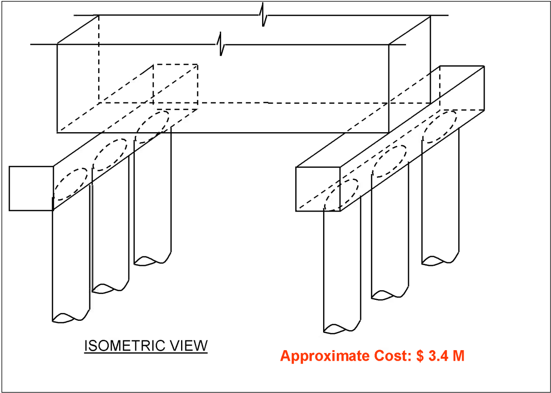
Figure 9.3: Isometric view of Figure 1
