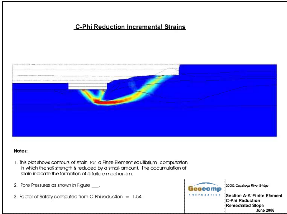
Figure 7B.6: Stability Analysis with PLAXIS for Unloaded Slope
