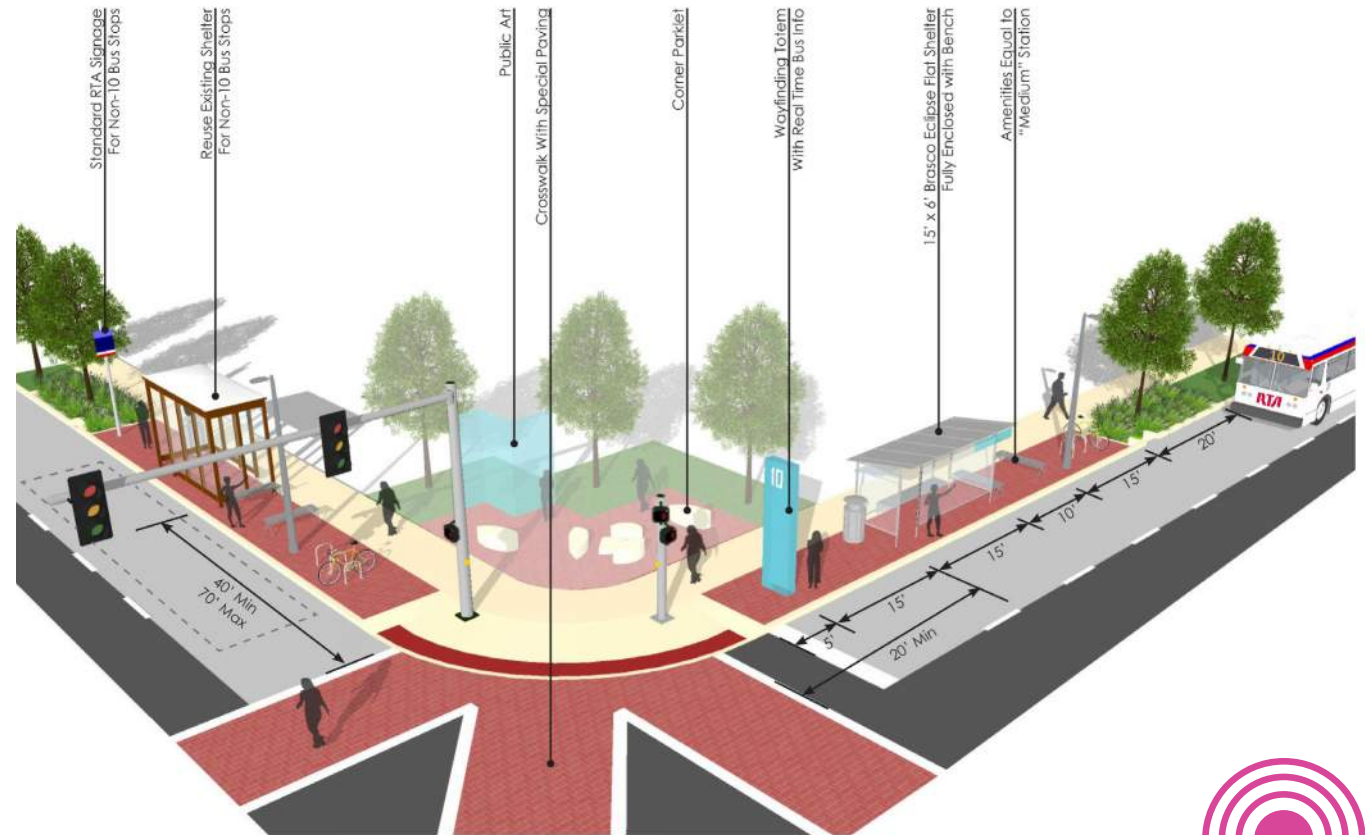
Corner Station
