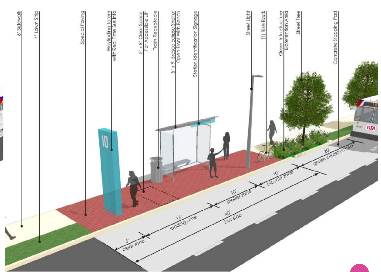
Narrow Station
