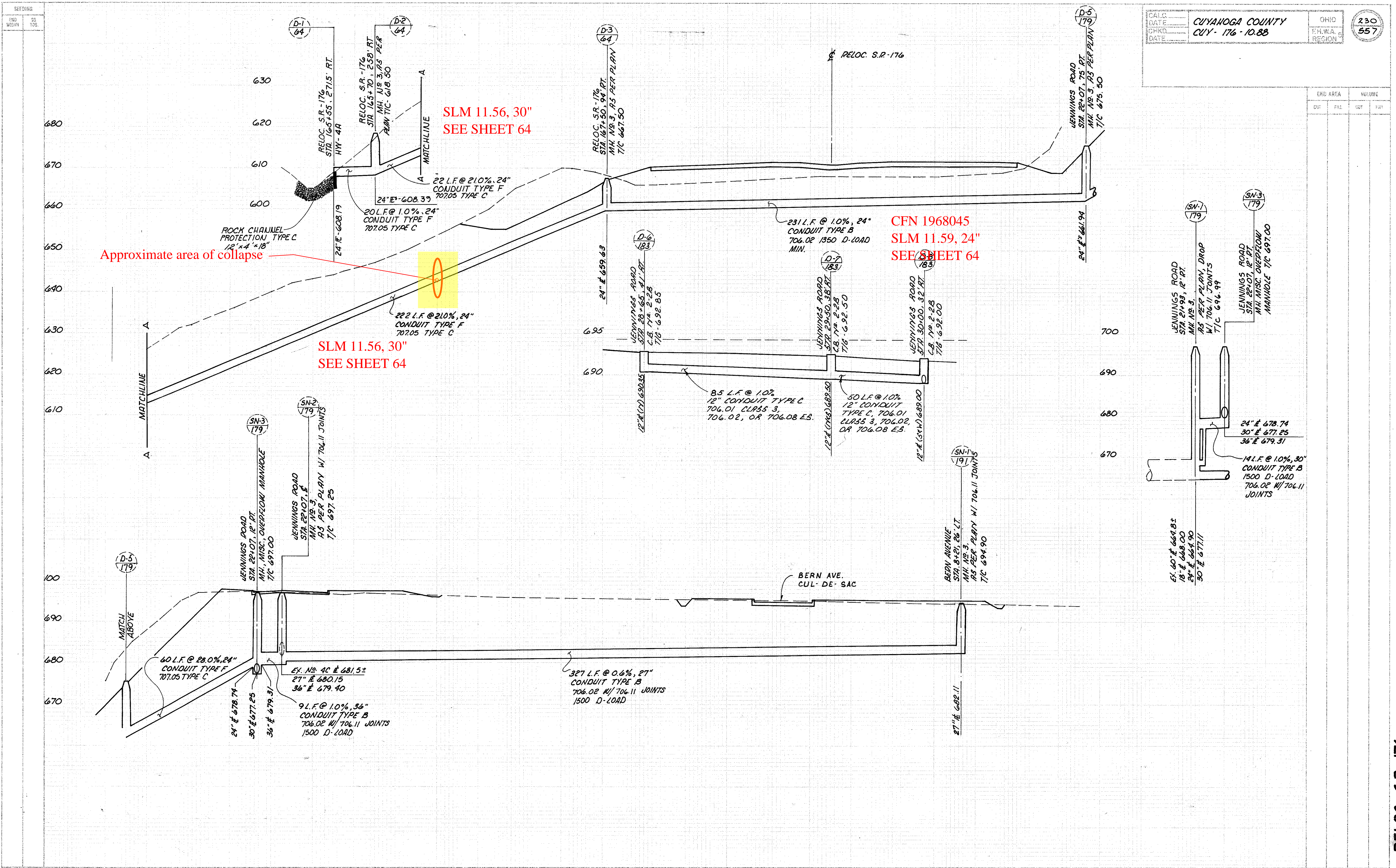
PIPE PROFILES
