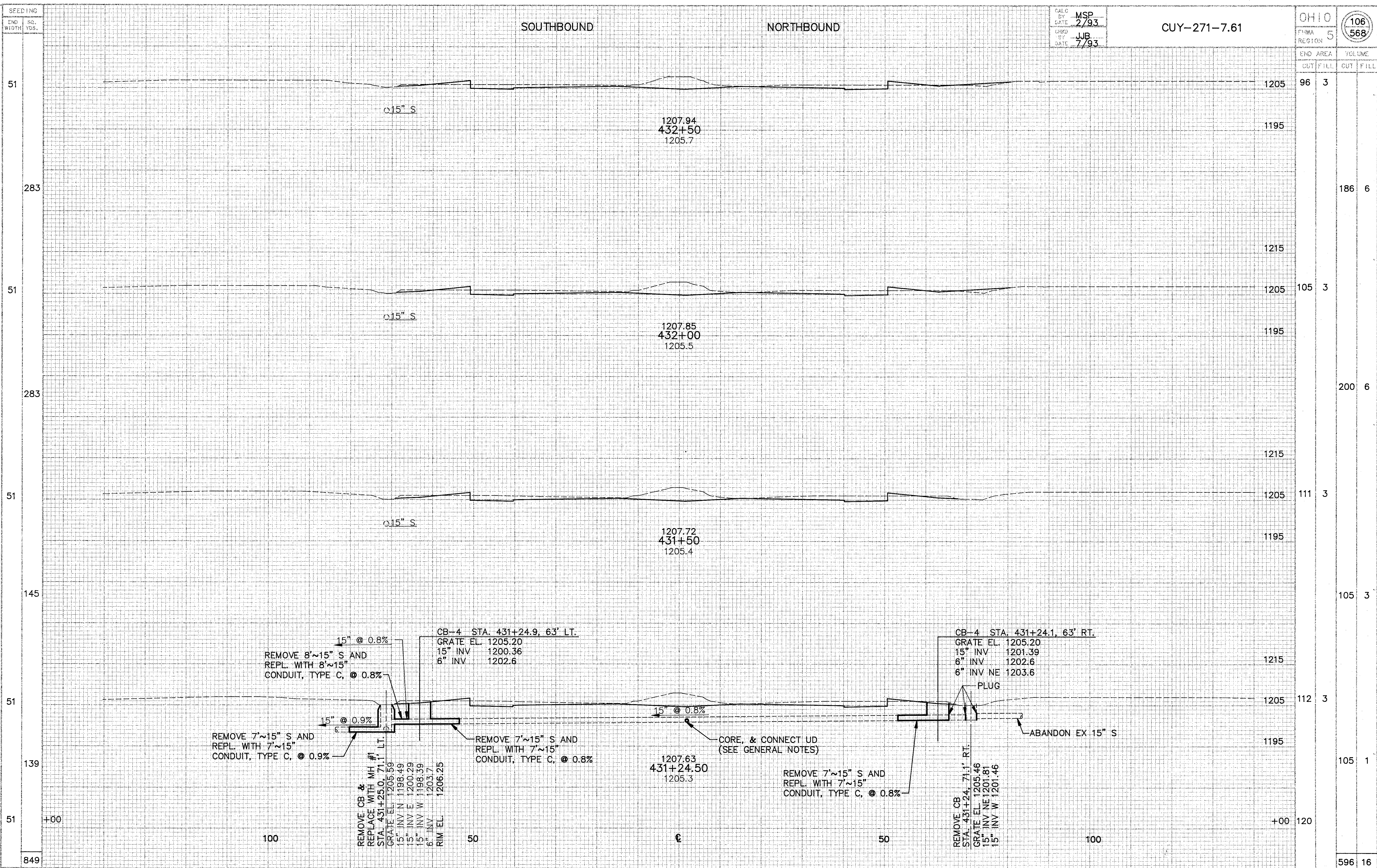
CROSS SECTIONS STA. 431+24.50 TO STA. 432+50
